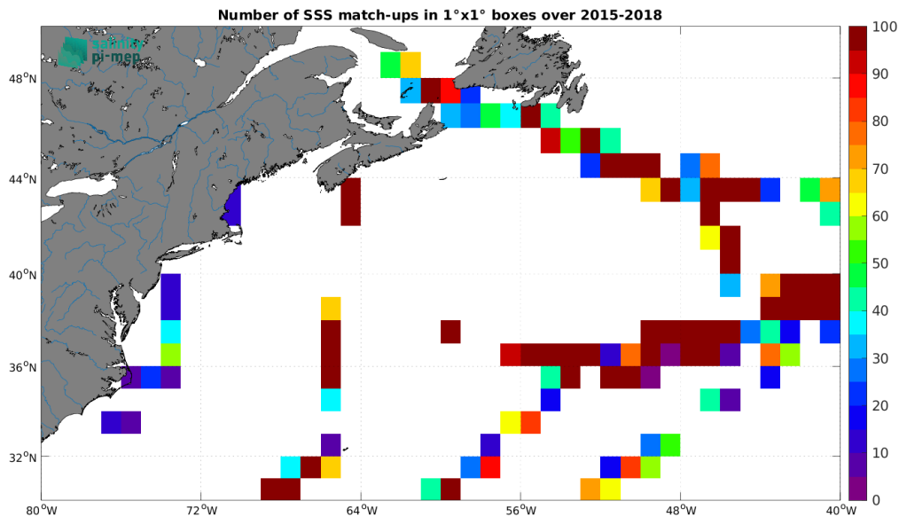
Figure 5: Number of SSS match-ups between TSG (GOSUD-Sailing-ship) SSS and the SMAP SSS L2 v6 - 40 km (RSS) SSS product for the Gulf Stream Pi-MEP region over 1^\circ \times 1^\circ boxes and for the full satellite product period.
