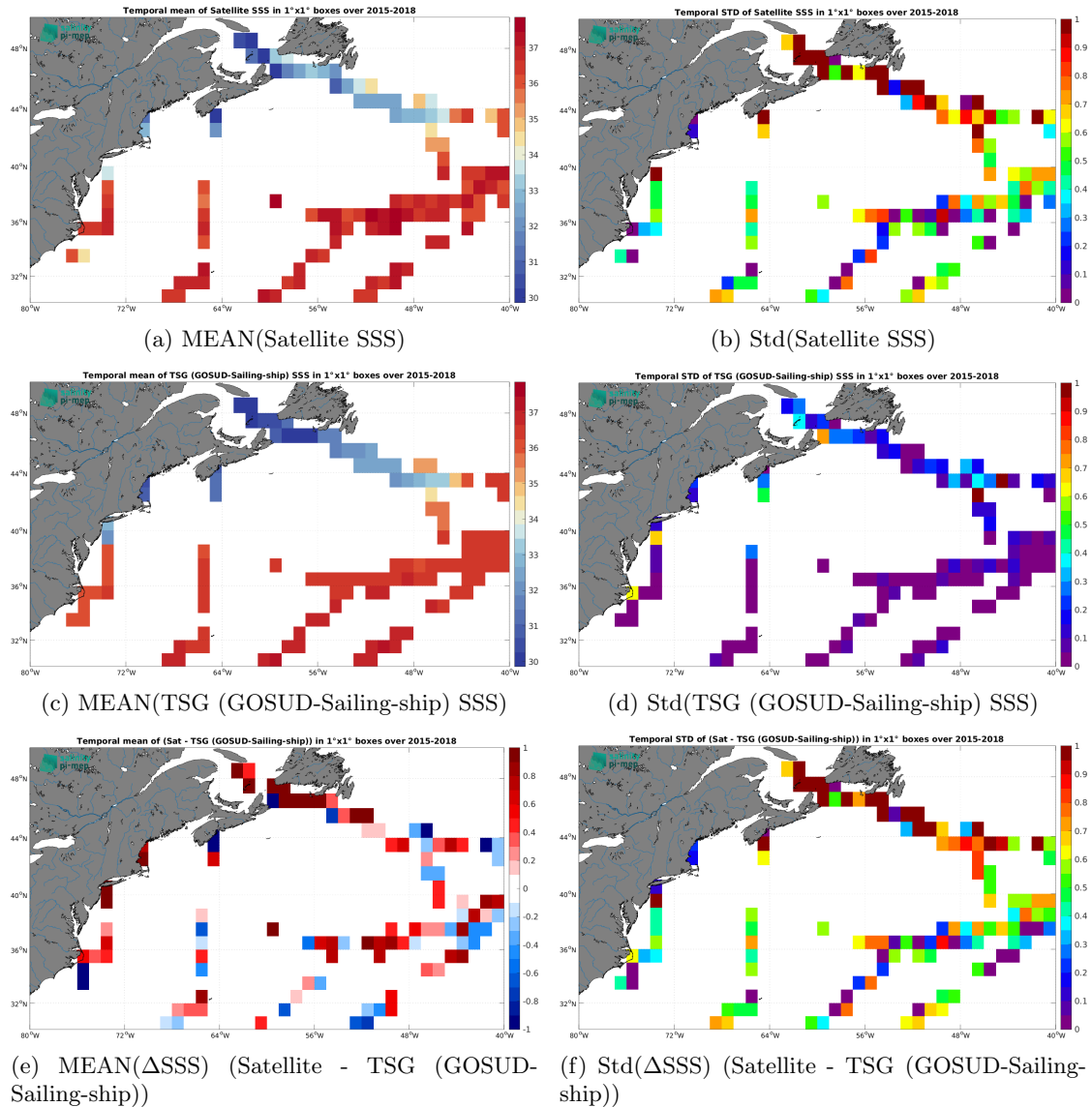
Figure 7: Temporal mean (left) and Std (right) of SSS from SMAP SSS L2 v6 - 40 km (RSS) (top), TSG (GOSUD-Sailing-ship) (middle), and of \Delta SSS (Satellite - TSG (GOSUD-Sailing-ship)). Only match-up pairs are used to generate these maps.
