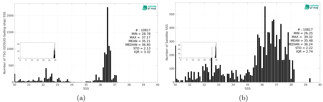
Figure 3: Histograms of SSS from TSG (GOSUD-Sailing-ship) (a) and SMAP SSS L2 v6 - 40 km (RSS) (b) considering all match-up pairs per bins of 0.1 over the Gulf Stream Pi-MEP region and for the full satellite product period.
