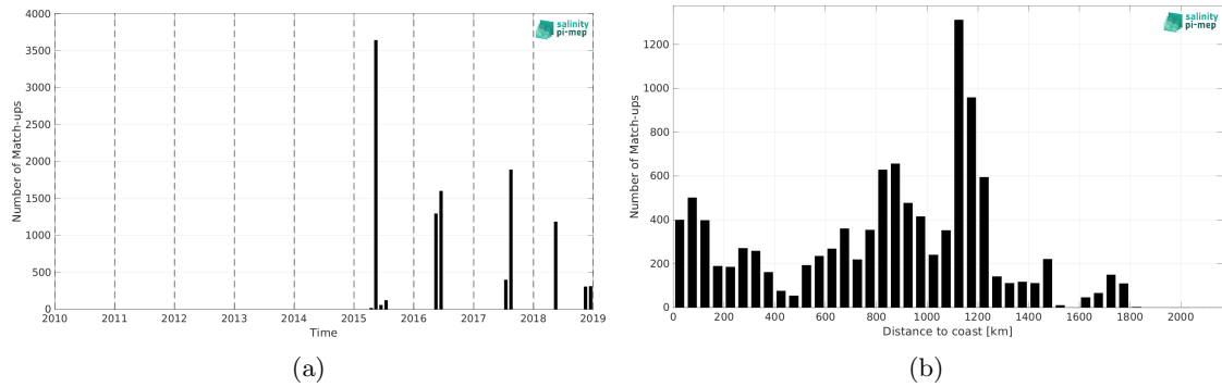
Figure 2: Number of match-ups between TSG (GOSUD-Sailing-ship) and SMAP SSS L2 v6 - 40 km (RSS) SSS as a function of time (a) and as function of the distance to coast (b) over the Gulf Stream Pi-MEP region and for the full satellite product period.
