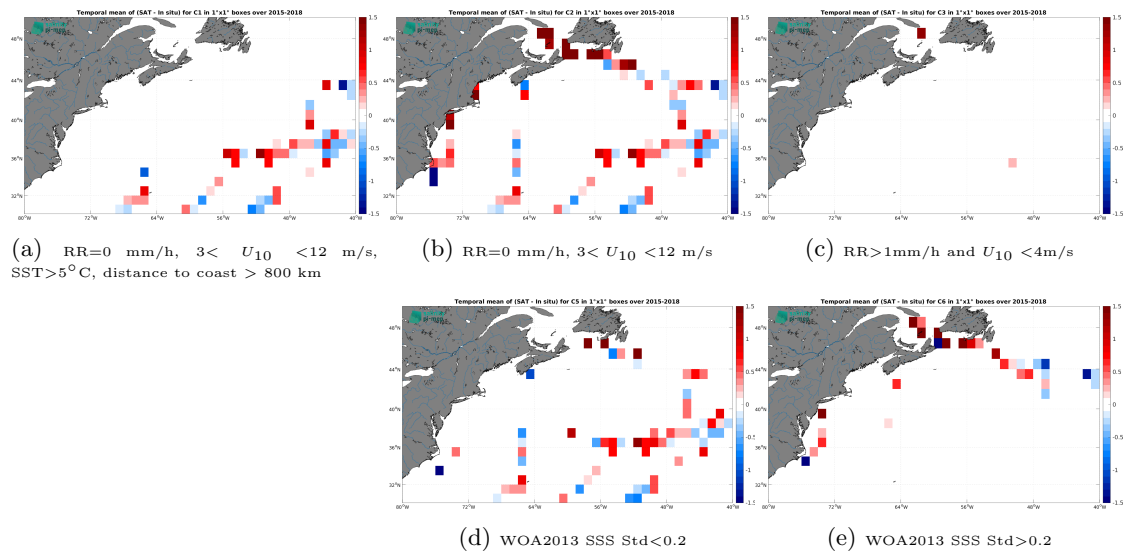
Figure 14: Temporal mean gridded over spatial boxes of size 1^\circ \times 1^\circ of \Delta SSS (SMAP SSS L2 v6 - 40 km (RSS) - TSG (GOSUD-Sailing-ship)) for 5 different subdatasets corresponding to:RR=0 mm/h, 3 < U_{10} < 12 m/s, SST > 5°C, distance to coast > 800 km (a), RR=0 mm/h, 3 < U_{10} < 12 m/s (b), RR > 1mm/h and U_{10} < 4 m/s (c), WOA2013 SSS Std < 0.2 (d), WOA2013 SSS Std > 0.2 (e).
