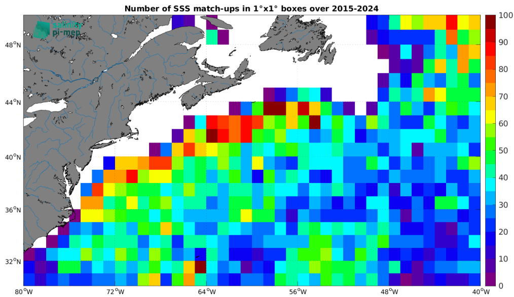
Figure 5: Number of SSS match-ups between Argo SSS and the SMAP SSS L2 v6 - 40 km (RSS) SSS product for the Gulf Stream Pi-MEP region over 1^\circ \times 1^\circ boxes and for the full satellite product period.
