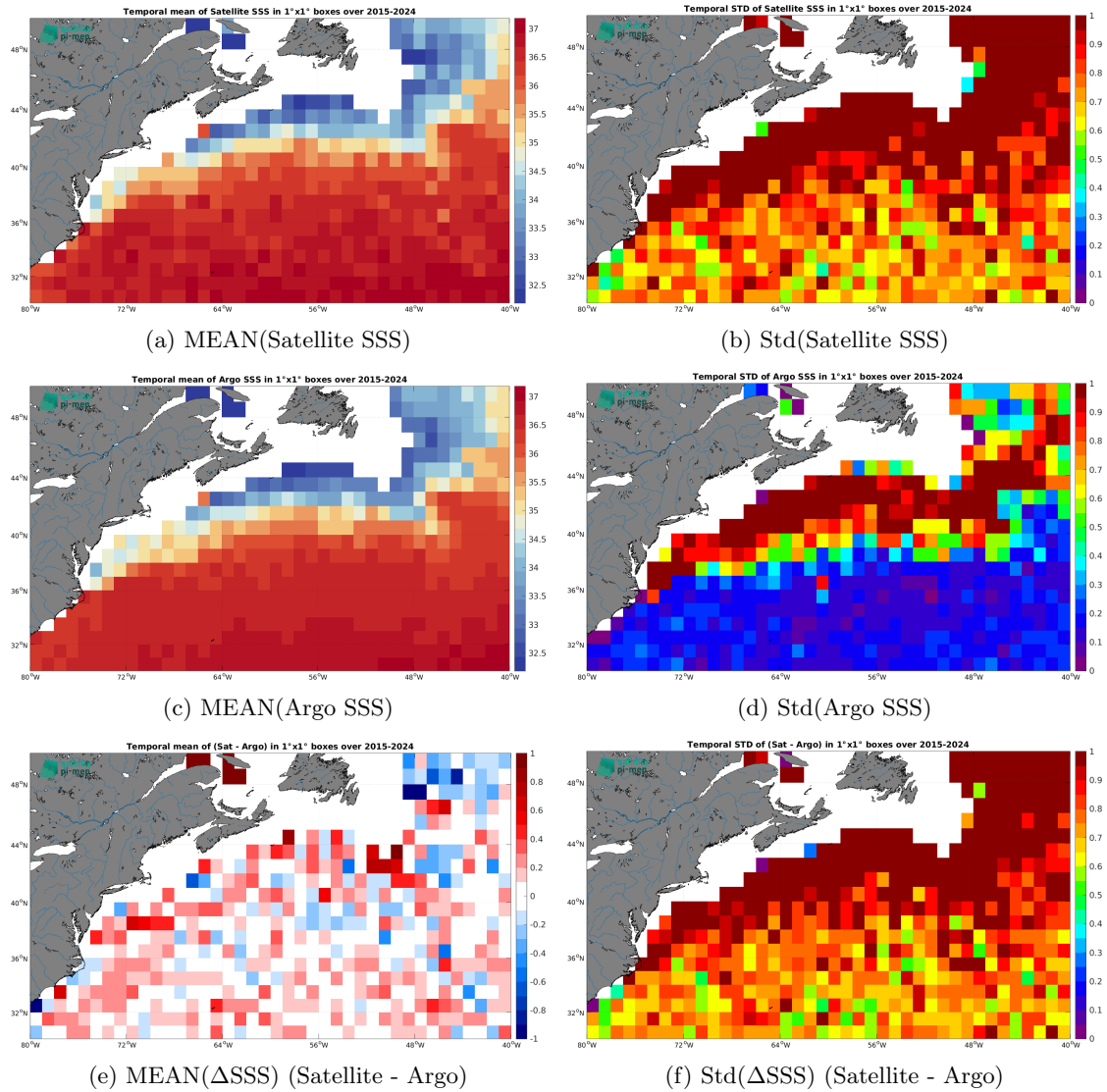
Figure 7: Temporal mean (left) and Std (right) of SSS from SMAP SSS L2 v6 - 40 km (RSS) (top), Argo (middle), and of \Delta SSS (Satellite - Argo). Only match-up pairs are used to generate these maps.
