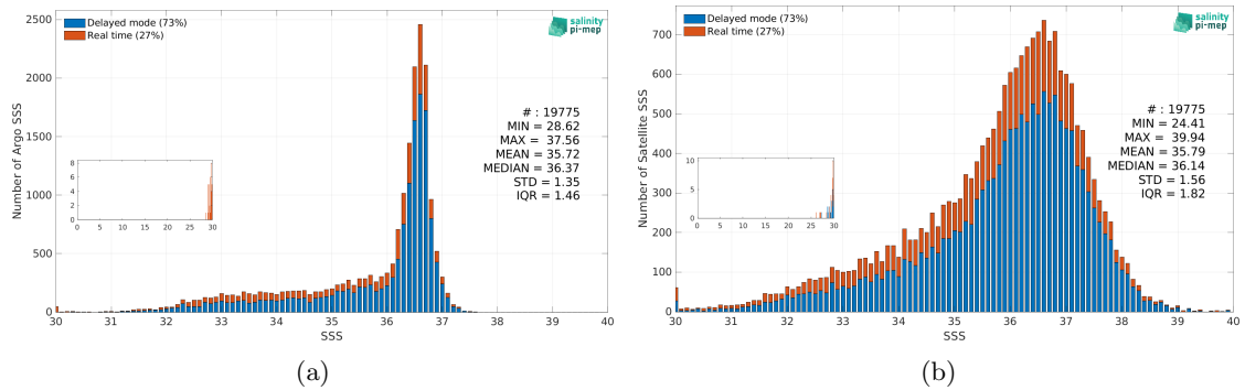
Figure 3: Histograms of SSS from Argo (a) and SMAP SSS L2 v6 - 40 km (RSS) (b) considering all match-up pairs per bins of 0.1 over the Gulf Stream Pi-MEP region and for the full satellite product period.
