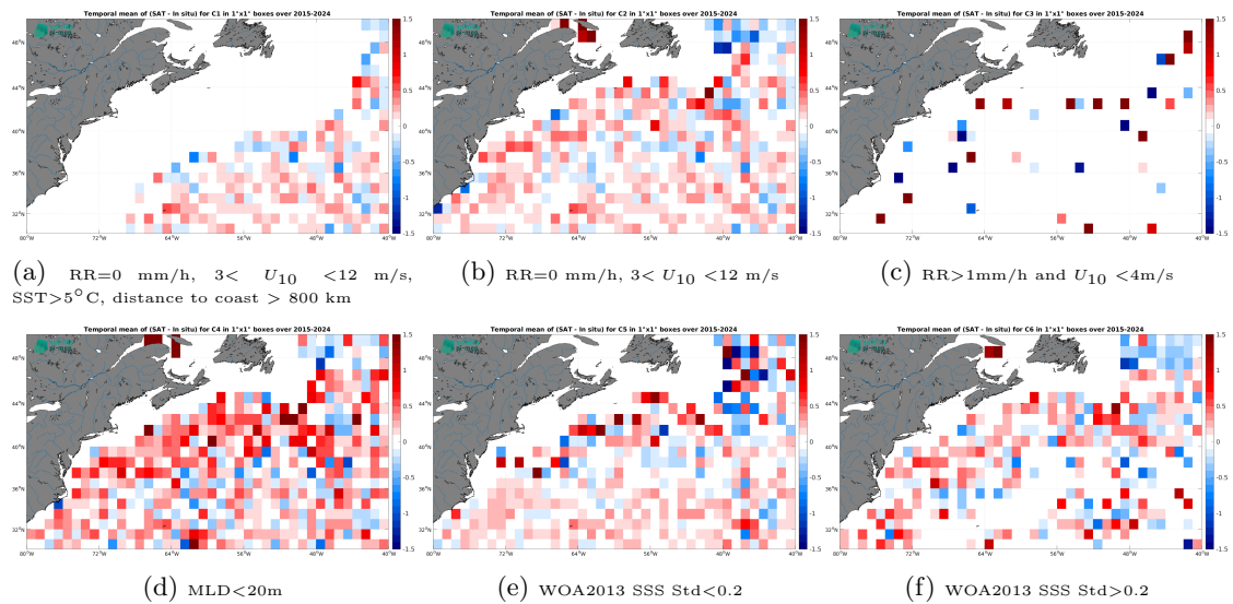
Figure 14: Temporal mean gridded over spatial boxes of size 1^\circ \times 1^\circ of \Delta SSS (SMAP SSS L2 v6 - 40 km (RSS) - Argo) for 6 different subdatasets corresponding to:RR=0 mm/h, 3 < U_{10} < 12 m/s, SST >5^\circ C, distance to coast > 800 km (a), RR=0 mm/h, 3 < U_{10} < 12 m/s (b), RR >1 mm/h and U_{10} < 4 m/s (c),MLD <20 m (d),WOA2013 SSS Std <0.2 (e),WOA2013 SSS Std >0.2 (f).
