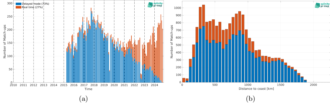
Figure 2: Number of match-ups between Argo and SMAP SSS L2 v6 - 40 km (RSS) SSS as a function of time (a) and as function of the distance to coast (b) over the Gulf Stream Pi-MEP region and for the full satellite product period.
