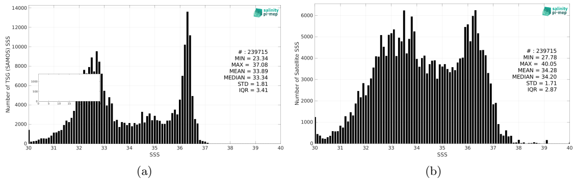
Figure 2: Histograms of SSS from TSG (SAMOS) (a) and SMAP SSS L2 v5 (RSS) (b) considering all match-up pairs per bins of 0.1 over the Gulf Stream Pi-MEP region and for the full satellite product period.
