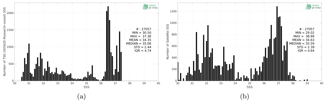
Figure 2: Histograms of SSS from TSG (GOSUD-Research-vessel) (a) and SMAP SSS L2 v5 (RSS) (b) considering all match-up pairs per bins of 0.1 over the Gulf Stream Pi-MEP region and for the full satellite product period.
