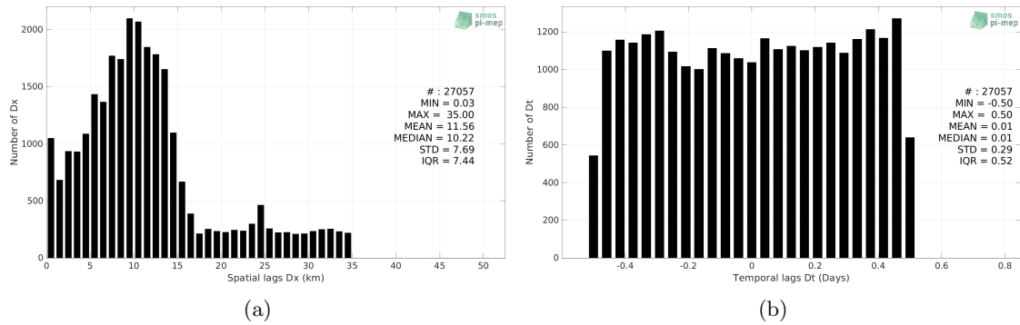
Figure 5: Histograms of the spatial (a) and temporal (b) lags between the location/time of the TSG (GOSUD-Research-vessel) measurement and the date of the corresponding SMAP SSS L2 v5 (RSS) SSS pixel.
