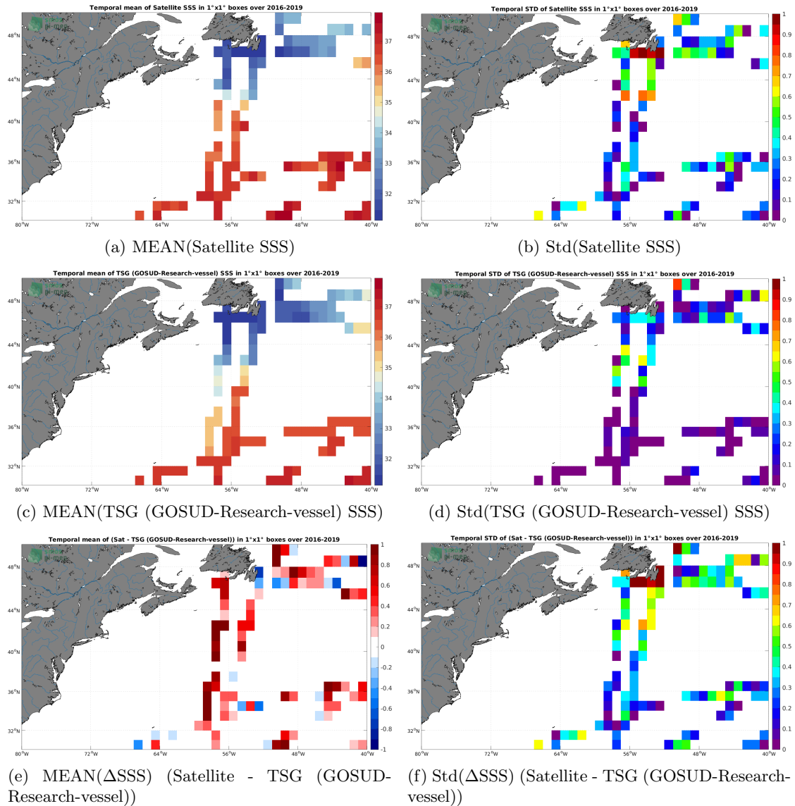
Figure 6: Temporal mean (left) and Std (right) of SSS from SMAP SSS L2 v5 (RSS) (top), TSG (GOSUD-Research-vessel) (middle), and of \Delta SSS (Satellite - TSG (GOSUD-Research-vessel)). Only match-up pairs are used to generate these maps.
