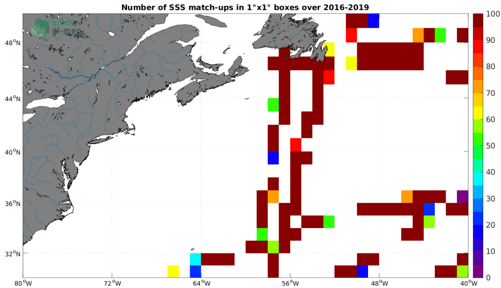
Figure 4: Number of SSS match-ups between TSG (GOSUD-Research-vessel) SSS and the SMAP SSS L2 v5 (RSS) SSS product for the Gulf Stream Pi-MEP region over 1^\circ \times 1^\circ boxes and for the full satellite product period.
