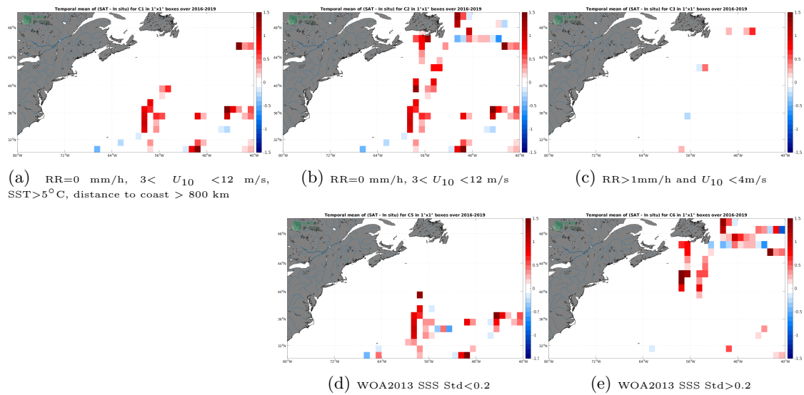
Figure 12: Temporal mean gridded over spatial boxes of size 1^\circ \times 1^\circ of \Delta SSS (SMAP SSS L2 v5 (RSS) - TSG (GOSUD-Research-vessel)) for 5 different subdatasets corresponding to:RR=0 mm/h, 3 < U_{10} < 12 m/s, SST > 5°C, distance to coast > 800 km (a), RR=0 mm/h, 3 < U_{10} < 12 m/s (b), RR > 1mm/h and U_{10} < 4 m/s (c), WOA2013 SSS Std < 0.2 (d), WOA2013 SSS Std > 0.2 (e).
