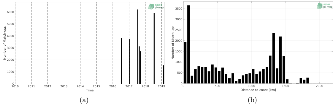
Figure 1: Number of match-ups between TSG (GOSUD-Research-vessel) and SMAP SSS L2 v5 (RSS) SSS as a function of time (a) and as function of the distance to coast (b) over the Gulf Stream Pi-MEP region and for the full satellite product period.
