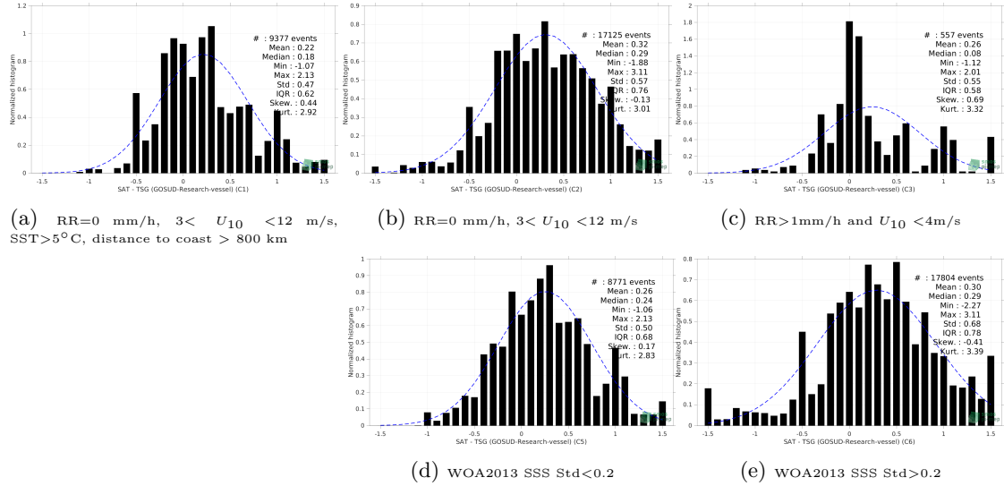
Figure 13: Normalized histogram of \Delta SSS (SMAP SSS L2 v5 (RSS) - TSG (GOSUD-Research-vessel)) for 5 different subdatasets corresponding to: RR=0 mm/h, 3 < U_{10} < 12 m/s, SST >5^{\circ} C, distance to coast > 800 km (a), RR=0 mm/h, 3 < U_{10} < 12 m/s (b), RR >1 mm/h and U_{10} < 4 m/s (c), WOA2013 SSS Std <0.2 (d), WOA2013 SSS Std >0.2 (e).
