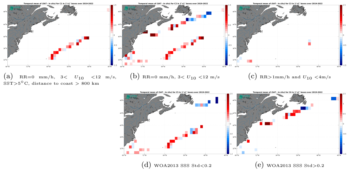
Figure 12: Temporal mean gridded over spatial boxes of size 1^\circ \times 1^\circ of \Delta SSS (SMAP SSS L2 v5 (RSS) - Saicdrone) for 5 different subdatasets corresponding to:RR=0 mm/h, 3 < U_{10} < 12 m/s, SST >5^\circ C, distance to coast > 800 km (a), RR=0 mm/h, 3 < U_{10} < 12 m/s (b), RR >1 mm/h and U_{10} < 4 m/s (c), WOA2013 SSS Std <0.2 (d), WOA2013 SSS Std >0.2 (e).
