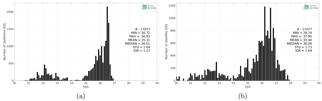
Figure 2: Histograms of SSS from Saildrone (a) and SMAP SSS L2 v5 (RSS) (b) considering all match-up pairs per bins of 0.1 over the Gulf Stream Pi-MEP region and for the full satellite product period.
