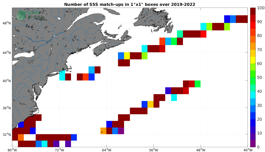
Figure 4: Number of SSS match-ups between Saildrone SSS and the SMAP SSS L2 v5 (RSS) SSS product for the Gulf Stream Pi-MEP region over 1^\circ \times 1^\circ boxes and for the full satellite product period.
