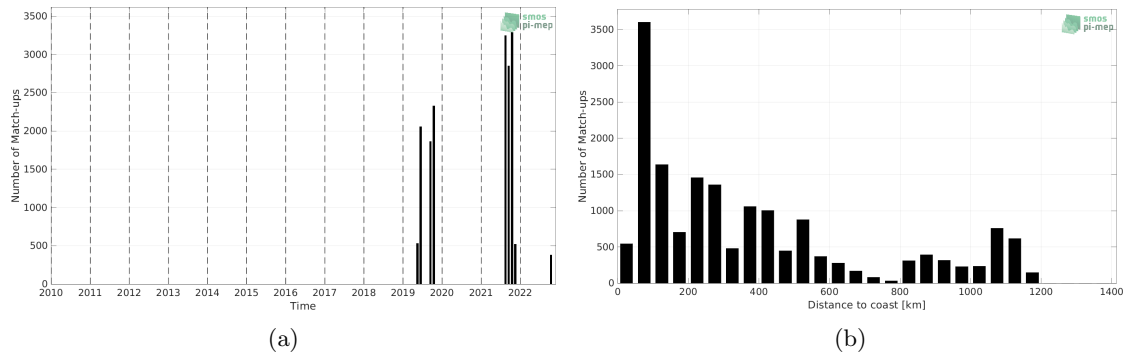
Figure 1: Number of match-ups between Saildrone and SMAP SSS L2 v5 (RSS) SSS as a function of time (a) and as function of the distance to coast (b) over the Gulf Stream Pi-MEP region and for the full satellite product period.
