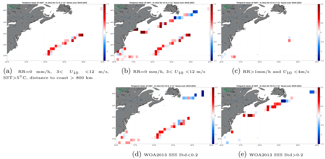
Figure 12: Temporal mean gridded over spatial boxes of size 1^\circ \times 1^\circ of \Delta SSS (SMAP SSS L2 v5 (RSS) - Saikrone) for 5 different subdatasets corresponding to:RR=0 mm/h, 3 < U_{10} < 12 m/s, SST >5^\circ C, distance to coast > 800 km (a), RR=0 mm/h, 3 < U_{10} < 12 m/s (b), RR >1 mm/h and U_{10} < 4 m/s (c), WOA2013 SSS Std <0.2 (d), WOA2013 SSS Std >0.2 (e).
