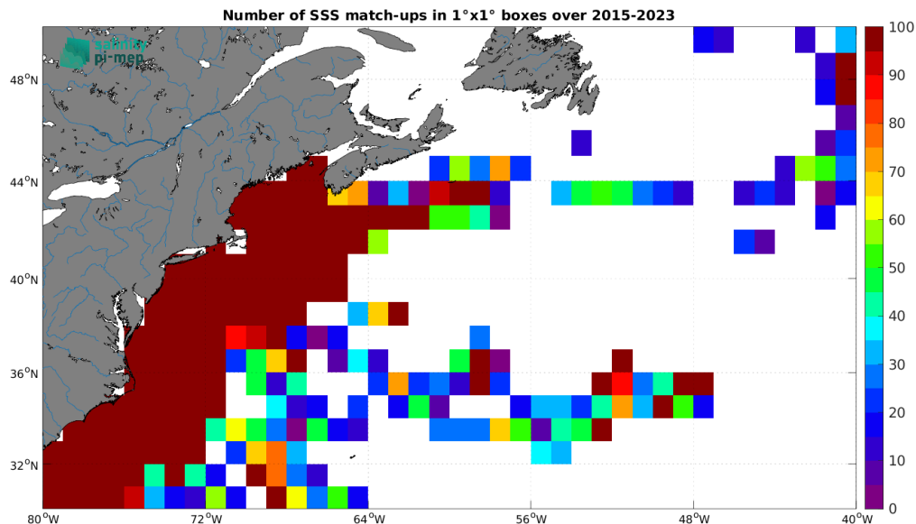
Figure 5: Number of SSS match-ups between TSG (SAMOS) SSS and the SMAP SSS L2 v5.3 (RSS) SSS product for the Gulf Stream Pi-MEP region over 1^\circ \times 1^\circ boxes and for the full satellite product period.
