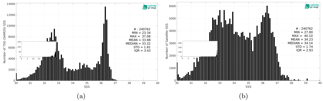
Figure 3: Histograms of SSS from TSG (SAMOS) (a) and SMAP SSS L2 v5.3 (RSS) (b) considering all match-up pairs per bins of 0.1 over the Gulf Stream Pi-MEP region and for the full satellite product period.
