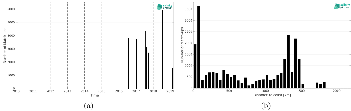
Figure 2: Number of match-ups between TSG (GOSUD-Research-vessel) and SMAP SSS L2 v5.3 (RSS) SSS as a function of time (a) and as function of the distance to coast (b) over the Gulf Stream Pi-MEP region and for the full satellite product period.
