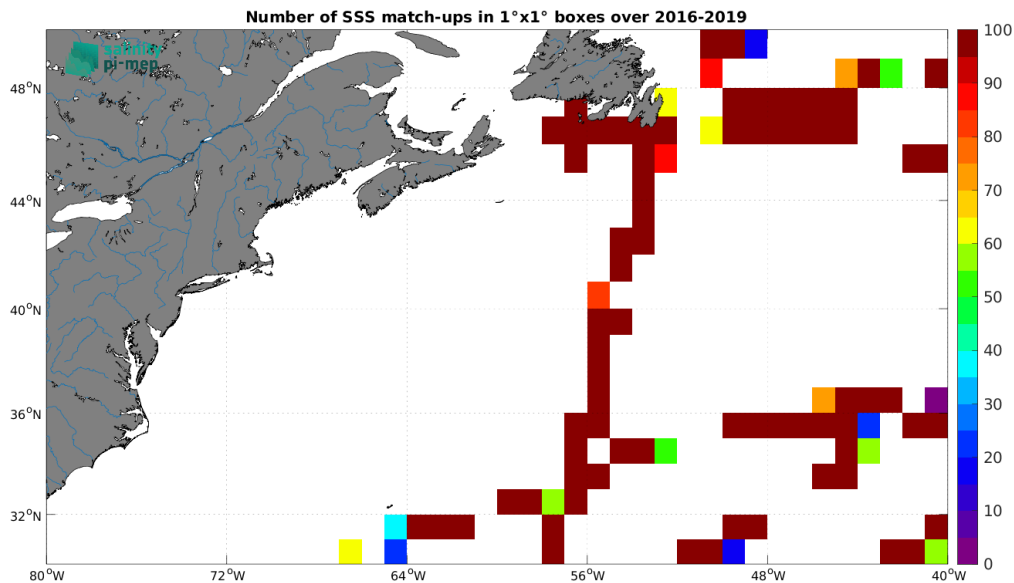
Figure 5: Number of SSS match-ups between TSG (GOSUD-Research-vessel) SSS and the SMAP SSS L2 v5.3 (RSS) SSS product for the Gulf Stream Pi-MEP region over 1^\circ \times 1^\circ boxes and for the full satellite product period.
