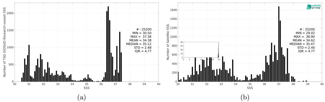
Figure 3: Histograms of SSS from TSG (GOSUD-Research-vessel) (a) and SMAP SSS L2 v5.3 (RSS) (b) considering all match-up pairs per bins of 0.1 over the Gulf Stream Pi-MEP region and for the full satellite product period.
