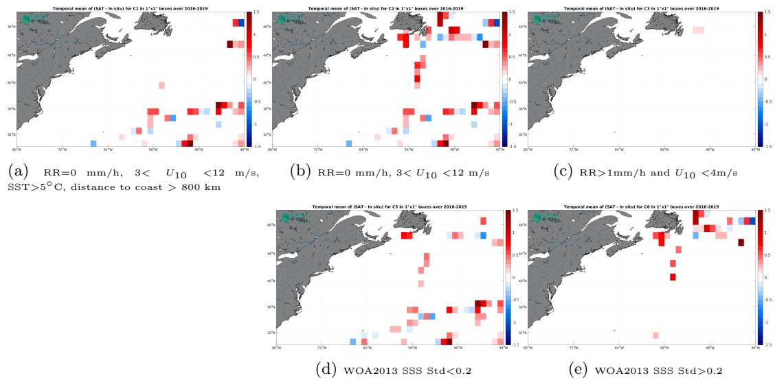
Figure 14: Temporal mean gridded over spatial boxes of size 1^\circ \times 1^\circ of \Delta SSS (SMAP SSS L2 v5.3 (RSS) - TSG (GOSUD-Research-vessel)) for 5 different subdatasets corresponding to:RR=0 mm/h, 3 < U_{10} < 12 m/s, SST > 5°C, distance to coast > 800 km (a), RR=0 mm/h, 3 < U_{10} < 12 m/s (b), RR > 1mm/h and U_{10} < 4 m/s (c), WOA2013 SSS Std < 0.2 (d), WOA2013 SSS Std > 0.2 (e).
