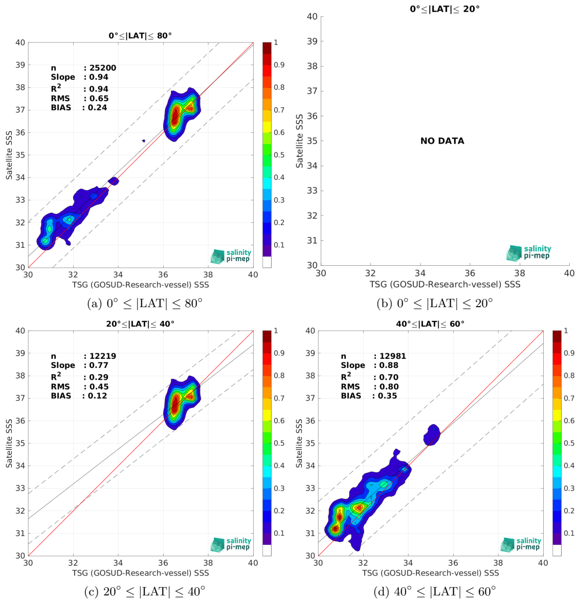
Figure 10: Contour maps of the concentration of SMAP SSS L2 v5.3 (RSS) SSS (y-axis) versus TSG (GOSUD-Research-vessel) SSS (x-axis) at match-up pairs for different latitude bands. For each plot, the red line shows x=y . The black thin and dashed lines indicate a linear fit through the data cloud and the \pm 95\% confidence levels, respectively. The number match-up pairs n , the slope and R^2 coefficient of the linear fit, the root mean square (RMS) and the mean bias between satellite and in situ data are indicated for each latitude band in each plots.
