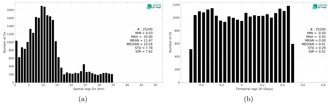
Figure 6: Histograms of the spatial (a) and temporal (b) lags between the location/time of the TSG (GOSUD-Research-vessel) measurement and the date of the corresponding SMAP SSS L2 v5.3 (RSS) SSS pixel.
