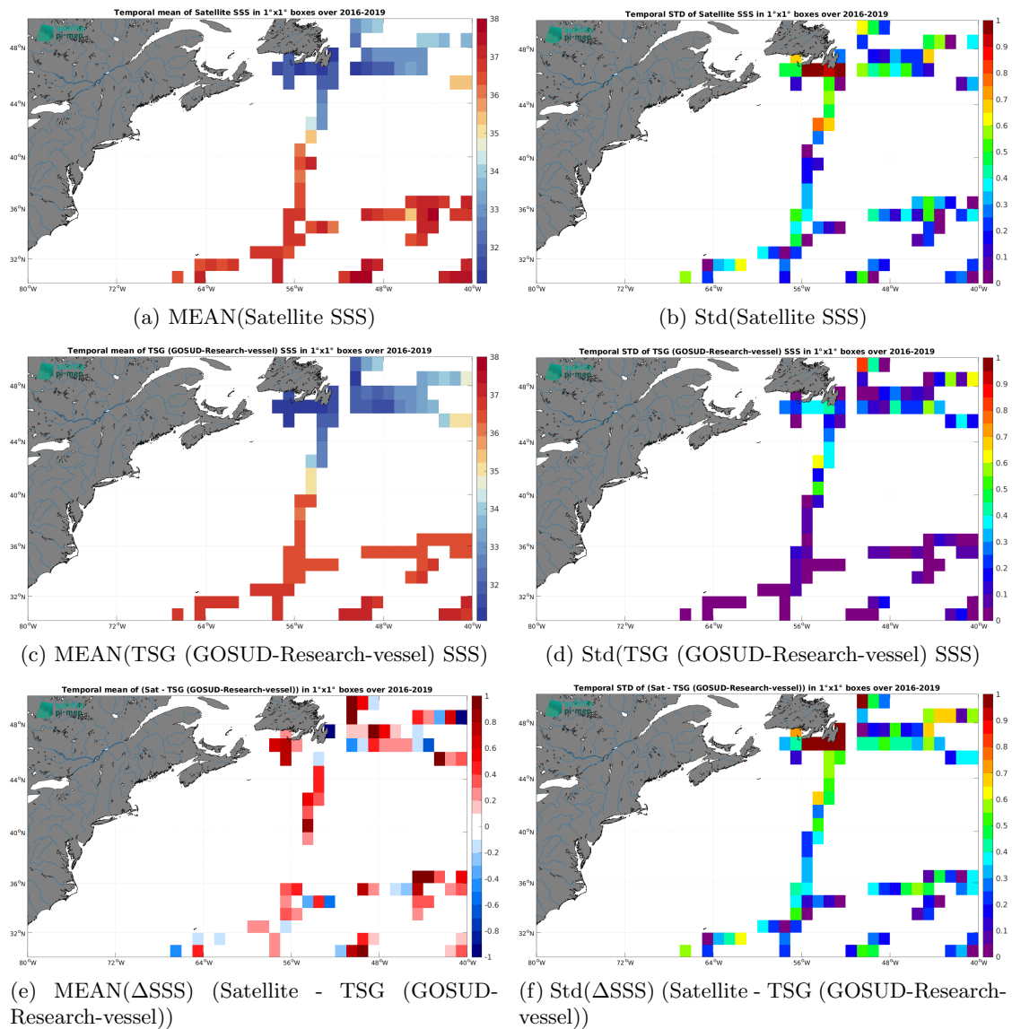
Figure 7: Temporal mean (left) and Std (right) of SSS from SMAP SSS L2 v5.3 (RSS) (top), TSG (GOSUD-Research-vessel) (middle), and of \Delta SSS (Satellite - TSG (GOSUD-Research-vessel)). Only match-up pairs are used to generate these maps.
