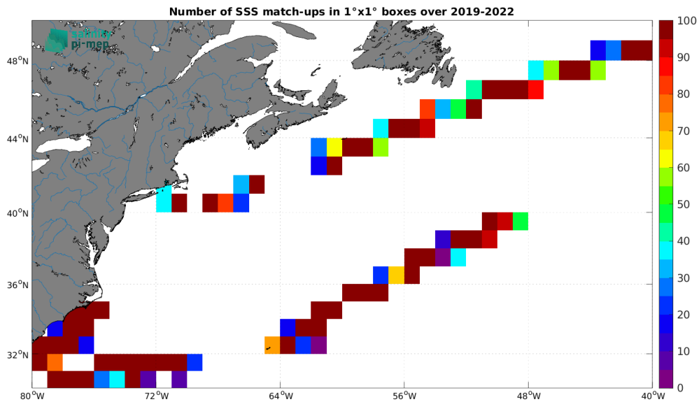
Figure 5: Number of SSS match-ups between Saildrone SSS and the SMAP SSS L2 v5.3 (RSS) SSS product for the Gulf Stream Pi-MEP region over 1^\circ \times 1^\circ boxes and for the full satellite product period.
