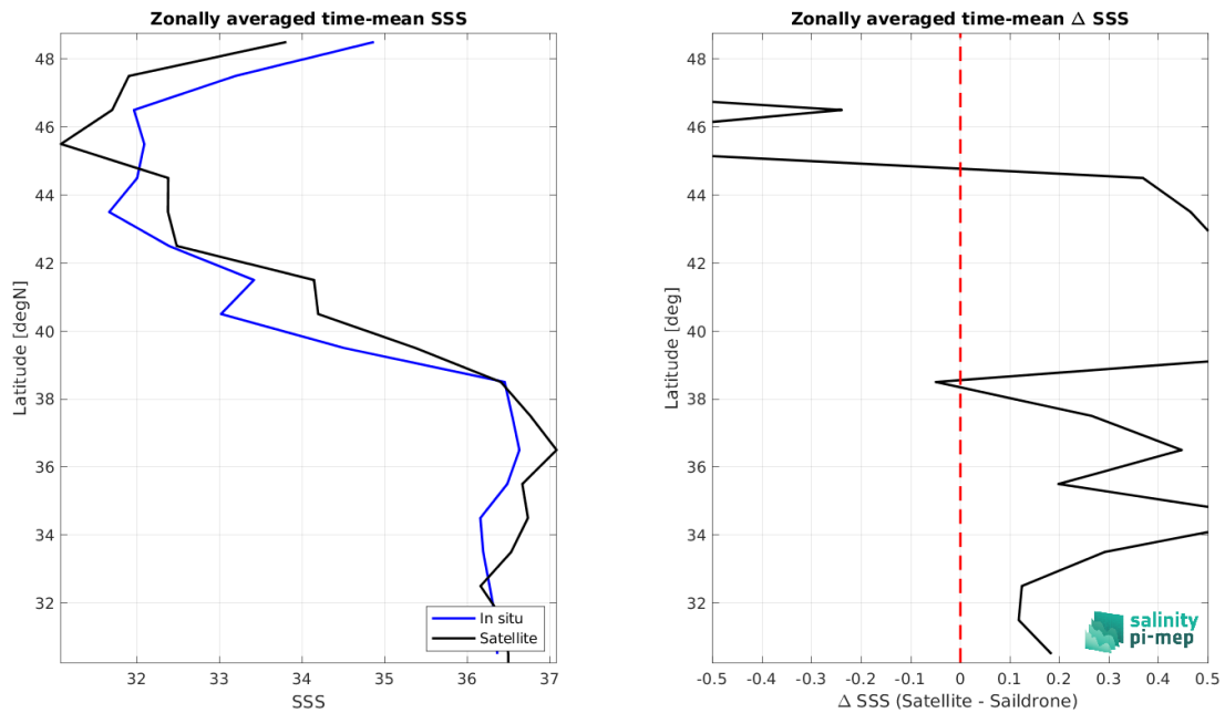
Figure 9: Left panel: Zonal mean SSS from SMAP SSS L2 v5.3 (RSS) satellite product (black) and from Sairdron (blue). Right panel: Zonal mean of \Delta SSS (Satellite - Sairdron) for all the collected Pi-MEP match-up pairs estimated over the full satellite product period.
