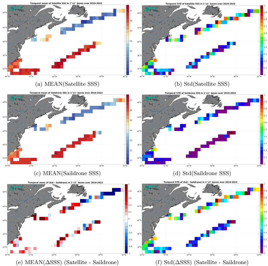
Figure 7: Temporal mean (left) and Std (right) of SSS from SMAP SSS L2 v5.3 (RSS) (top), Saildrone (middle), and of \Delta SSS (Satellite - Saildrone). Only match-up pairs are used to generate these maps.
