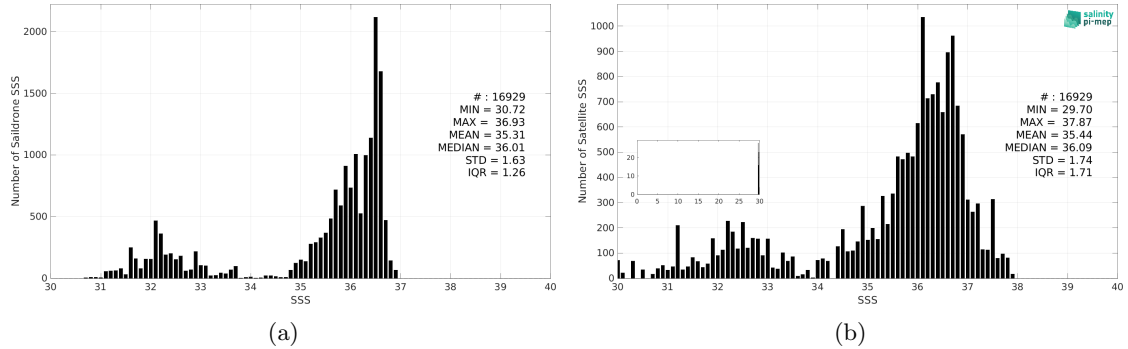
Figure 3: Histograms of SSS from Saildrone (a) and SMAP SSS L2 v5.3 (RSS) (b) considering all match-up pairs per bins of 0.1 over the Gulf Stream Pi-MEP region and for the full satellite product period.
