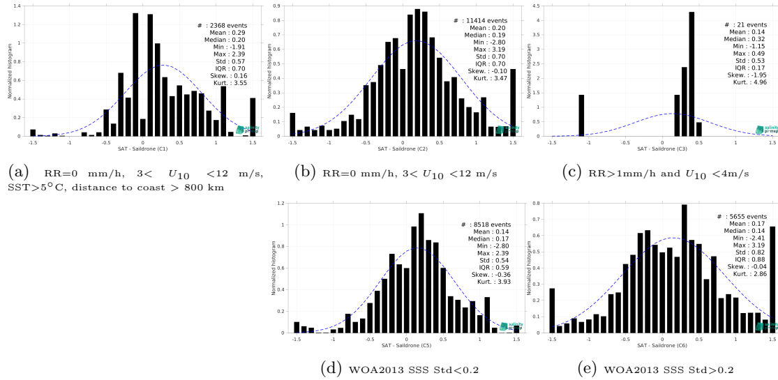
Figure 15: Normalized histogram of \Delta SSS (SMAP SSS L2 v5.3 (RSS) - Saildrone) for 5 different subdatasets corresponding to: RR=0 mm/h, 3 < U_{10} < 12 m/s, SST>5°C, distance to coast > 800 km (a), RR=0 mm/h, 3 < U_{10} < 12 m/s (b), RR>1mm/h and U_{10} < 4 m/s (c), WOA2013 SSS Std<0.2 (d), WOA2013 SSS Std>0.2 (e).
