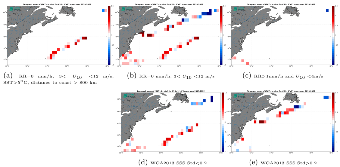
Figure 14: Temporal mean gridded over spatial boxes of size 1^\circ \times 1^\circ of \Delta SSS (SMAP SSS L2 v5.3 (RSS) - Saifdrone) for 5 different subdatasets corresponding to:RR=0 mm/h, 3 < U_{10} < 12 m/s, SST > 5°C, distance to coast > 800 km (a), RR=0 mm/h, 3 < U_{10} < 12 m/s (b), RR > 1mm/h and U_{10} < 4 m/s (c), WOA2013 SSS Std < 0.2 (d), WOA2013 SSS Std > 0.2 (e).
