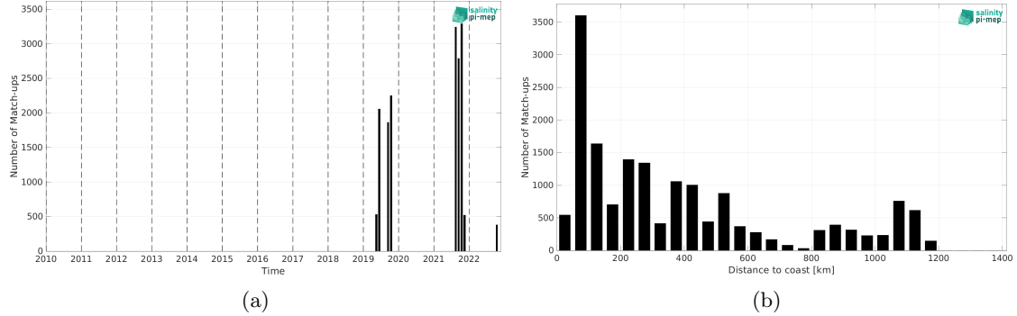
Figure 2: Number of match-ups between Saildrone and SMAP SSS L2 v5.3 (RSS) SSS as a function of time (a) and as function of the distance to coast (b) over the Gulf Stream Pi-MEP region and for the full satellite product period.
