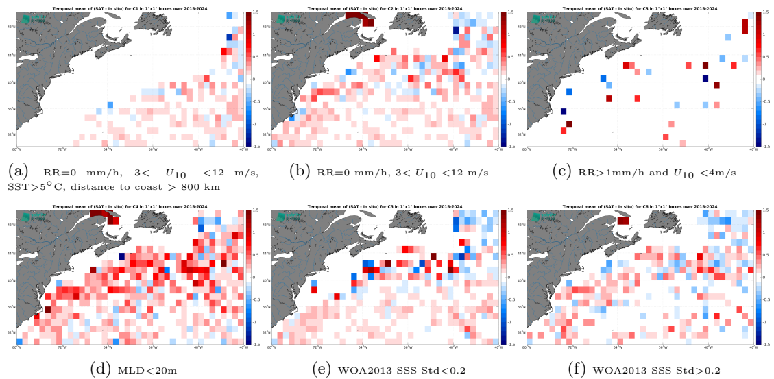
Figure 14: Temporal mean gridded over spatial boxes of size 1^\circ \times 1^\circ of \Delta SSS (SMAP SSS L2 v5.3 (RSS) - Argo) for 6 different subdatasets corresponding to:RR=0 mm/h, 3 < U_{10} < 12 m/s, SST>5°C, distance to coast > 800 km (a), RR=0 mm/h, 3 < U_{10} < 12 m/s (b), RR>1mm/h and U_{10} < 4 m/s (c),MLD<20m (d),WOA2013 SSS Std<0.2 (e),WOA2013 SSS Std>0.2 (f).
