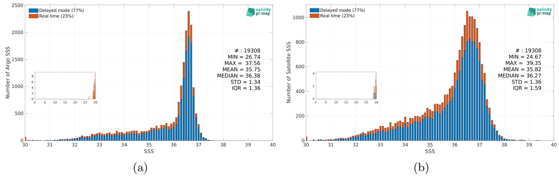
Figure 3: Histograms of SSS from Argo (a) and SMAP SSS L2 v5.3 (RSS) (b) considering all match-up pairs per bins of 0.1 over the Gulf Stream Pi-MEP region and for the full satellite product period.
