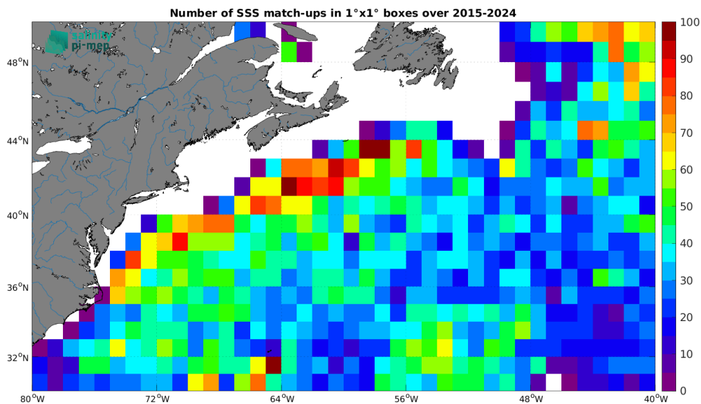
Figure 5: Number of SSS match-ups between Argo SSS and the SMAP SSS L2 v5.3 (RSS) SSS product for the Gulf Stream Pi-MEP region over 1^\circ \times 1^\circ boxes and for the full satellite product period.
