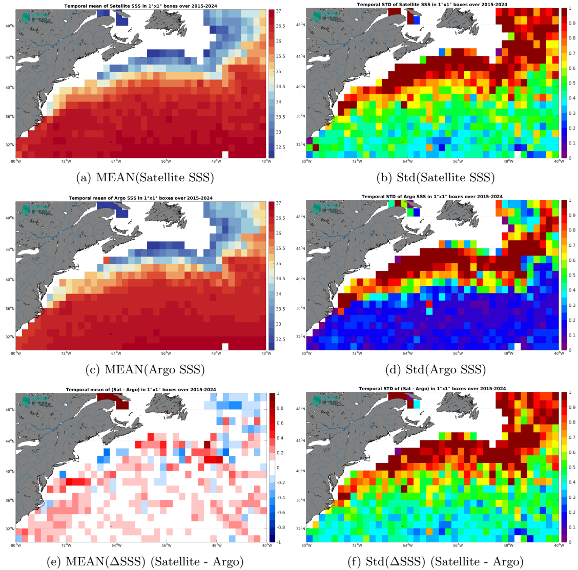
Figure 7: Temporal mean (left) and Std (right) of SSS from SMAP SSS L2 v5.3 (RSS) (top), Argo (middle), and of \Delta SSS (Satellite - Argo). Only match-up pairs are used to generate these maps.
