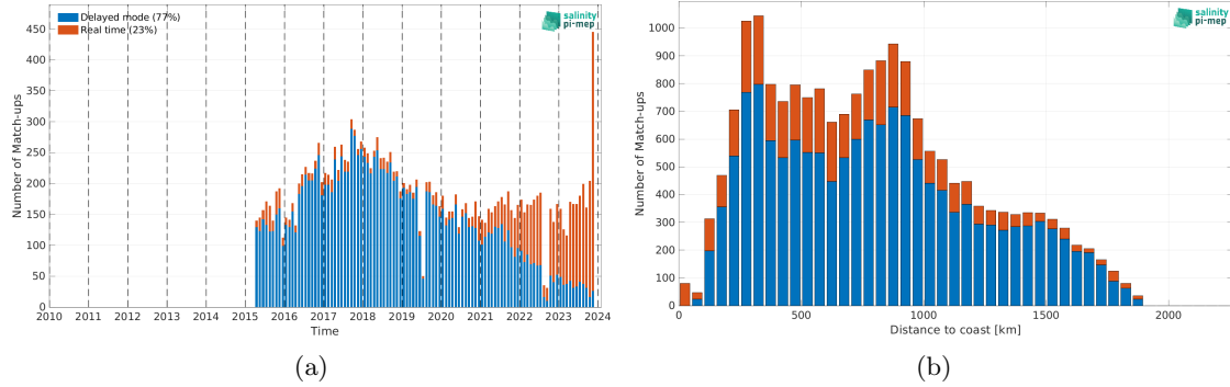
Figure 2: Number of match-ups between Argo and SMAP SSS L2 v5.3 (RSS) SSS as a function of time (a) and as function of the distance to coast (b) over the Gulf Stream Pi-MEP region and for the full satellite product period.
