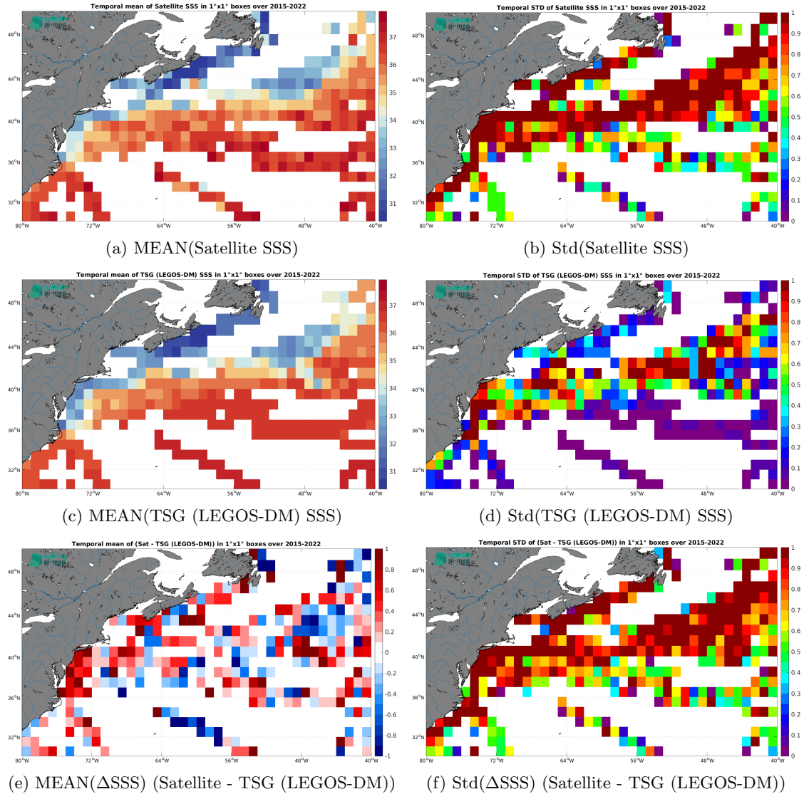
Figure 7: Temporal mean (left) and Std (right) of SSS from SMAP SSS L2 v5.3 - 40 km (RSS) (top), TSG (LEGOS-DM) (middle), and of \Delta SSS (Satellite - TSG (LEGOS-DM)). Only match-up pairs are used to generate these maps.
