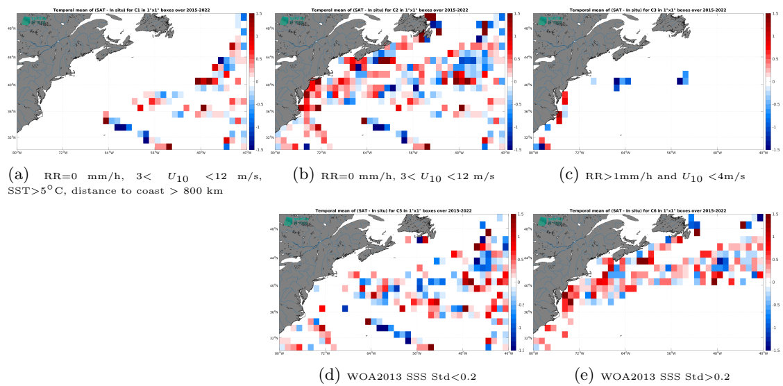
Figure 14: Temporal mean gridded over spatial boxes of size 1^\circ \times 1^\circ of \Delta SSS (SMAP SSS L2 v5.3 - 40 km (RSS) - TSG (LEGOS-DM)) for 5 different subdatasets corresponding to:RR=0 mm/h, 3 < U_{10} < 12 m/s, SST>5°C, distance to coast > 800 km (a), RR=0 mm/h, 3 < U_{10} < 12 m/s (b), RR>1mm/h and U_{10} < 4 m/s (c), WOA2013 SSS Std<0.2 (d), WOA2013 SSS Std>0.2 (e).
