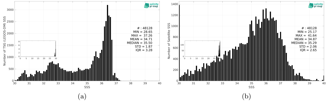
Figure 3: Histograms of SSS from TSG (LEGOS-DM) (a) and SMAP SSS L2 v5.3 - 40 km (RSS) (b) considering all match-up pairs per bins of 0.1 over the Gulf Stream Pi-MEP region and for the full satellite product period.
