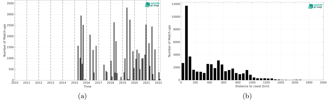
Figure 2: Number of match-ups between TSG (LEGOS-DM) and SMAP SSS L2 v5.3 - 40 km (RSS) SSS as a function of time (a) and as function of the distance to coast (b) over the Gulf Stream Pi-MEP region and for the full satellite product period.
