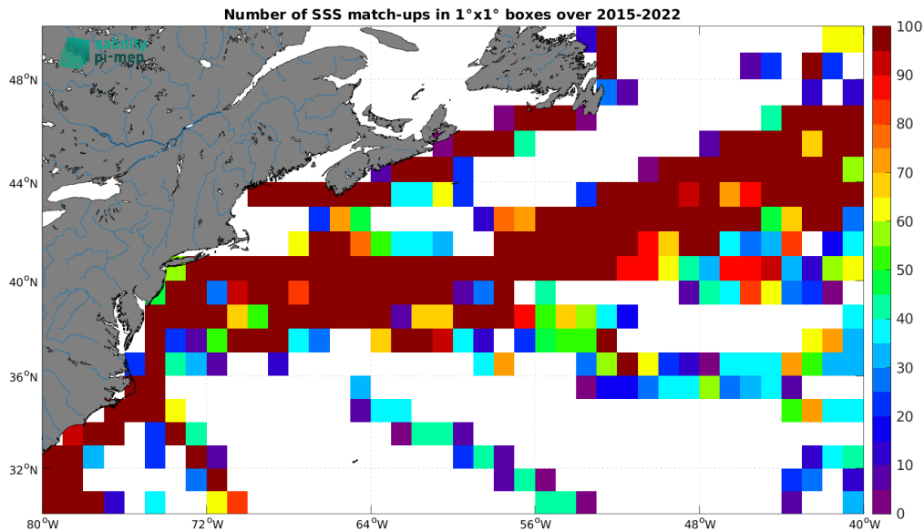
Figure 5: Number of SSS match-ups between TSG (LEGOS-DM) SSS and the SMAP SSS L2 v5.3 - 40 km (RSS) SSS product for the Gulf Stream Pi-MEP region over 1^\circ \times 1^\circ boxes and for the full satellite product period.
