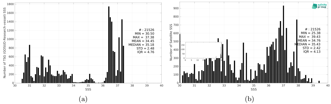
Figure 3: Histograms of SSS from TSG (GOSUD-Research-vessel) (a) and SMAP SSS L2 v5.3 - 40 km (RSS) (b) considering all match-up pairs per bins of 0.1 over the Gulf Stream Pi-MEP region and for the full satellite product period.
