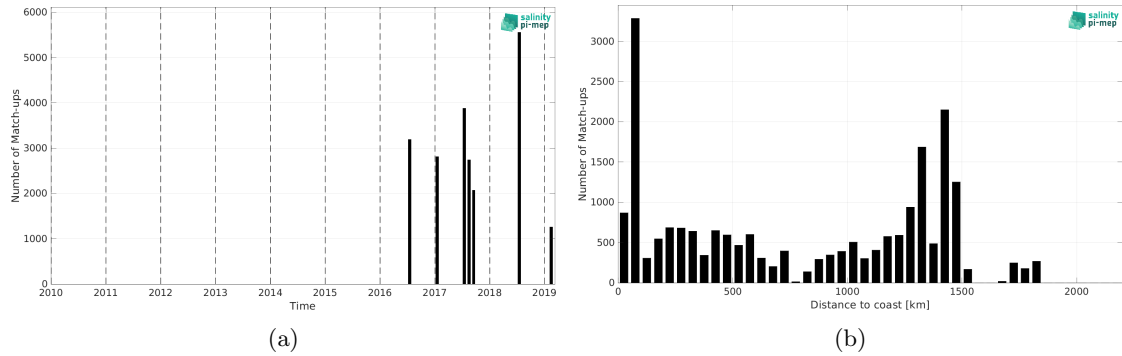
Figure 2: Number of match-ups between TSG (GOSUD-Research-vessel) and SMAP SSS L2 v5.3 - 40 km (RSS) SSS as a function of time (a) and as function of the distance to coast (b) over the Gulf Stream Pi-MEP region and for the full satellite product period.
