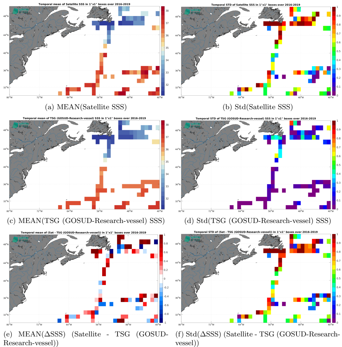
Figure 7: Temporal mean (left) and Std (right) of SSS from SMAP SSS L2 v5.3 - 40 km (RSS) (top), TSG (GOSUD-Research-vessel) (middle), and of \Delta SSS (Satellite - TSG (GOSUD-Research-vessel)). Only match-up pairs are used to generate these maps.
