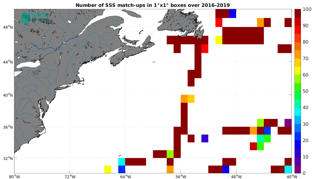
Figure 5: Number of SSS match-ups between TSG (GOSUD-Research-vessel) SSS and the SMAP SSS L2 v5.3 - 40 km (RSS) SSS product for the Gulf Stream Pi-MEP region over 1^\circ \times 1^\circ boxes and for the full satellite product period.
