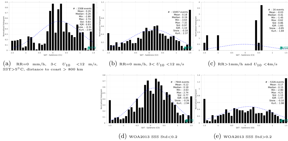
Figure 15: Normalized histogram of \Delta SSS (SMAP SSS L2 v5.3 - 40 km (RSS) - Saildrone) for 5 different subdatasets corresponding to: RR=0 mm/h, 3 < U_{10} < 12 m/s, SST>5°C, distance to coast > 800 km (a), RR=0 mm/h, 3 < U_{10} < 12 m/s (b), RR>1mm/h and U_{10} < 4 m/s (c), WOA2013 SSS Std<0.2 (d), WOA2013 SSS Std>0.2 (e).
