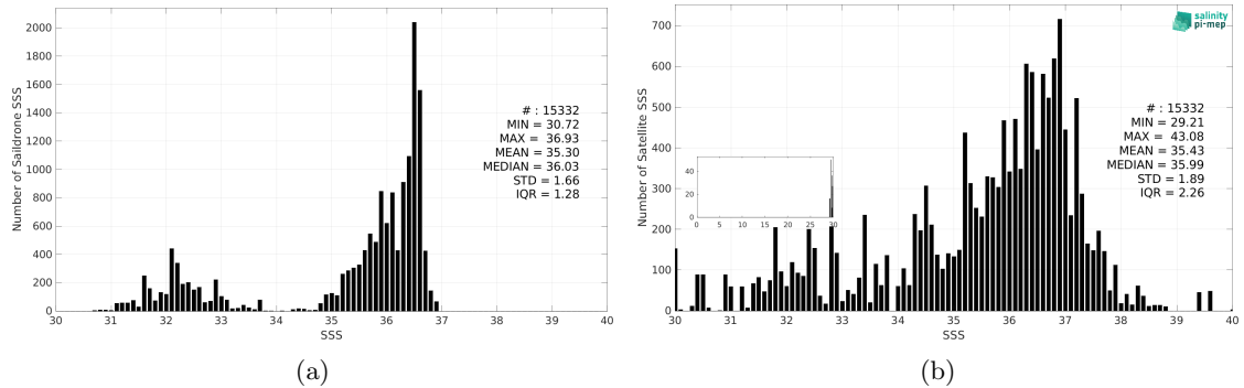
Figure 3: Histograms of SSS from Saildrone (a) and SMAP SSS L2 v5.3 - 40 km (RSS) (b) considering all match-up pairs per bins of 0.1 over the Gulf Stream Pi-MEP region and for the full satellite product period.
