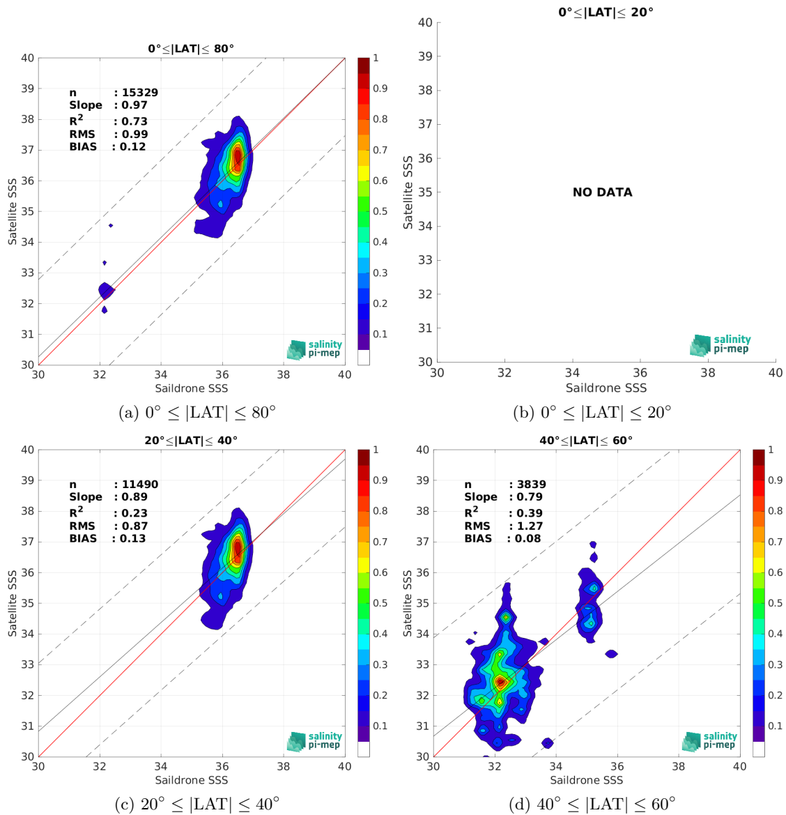
Figure 10: Contour maps of the concentration of SMAP SSS L2 v5.3 - 40 km (RSS) SSS (y-axis) versus Saildrone SSS (x-axis) at match-up pairs for different latitude bands. For each plot, the red line shows x=y . The black thin and dashed lines indicate a linear fit through the data cloud and the \pm 95\% confidence levels, respectively. The number match-up pairs n , the slope and R^2 coefficient of the linear fit, the root mean square (RMS) and the mean bias between satellite and in situ data are indicated for each latitude band in each plots.
