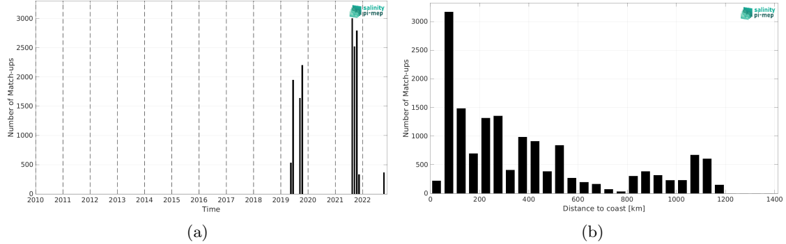
Figure 2: Number of match-ups between Saildrone and SMAP SSS L2 v5.3 - 40 km (RSS) SSS as a function of time (a) and as function of the distance to coast (b) over the Gulf Stream Pi-MEP region and for the full satellite product period.
