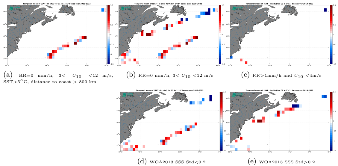
Figure 14: Temporal mean gridded over spatial boxes of size 1^\circ \times 1^\circ of \Delta SSS (SMAP SSS L2 v5.3 - 40 km (RSS) - Saildrone) for 5 different subdatasets corresponding to:RR=0 mm/h, 3 < U_{10} < 12 m/s, SST>5°C, distance to coast > 800 km (a), RR=0 mm/h, 3 < U_{10} < 12 m/s (b), RR>1mm/h and U_{10} < 4 m/s (c), WOA2013 SSS Std<0.2 (d), WOA2013 SSS Std>0.2 (e).
