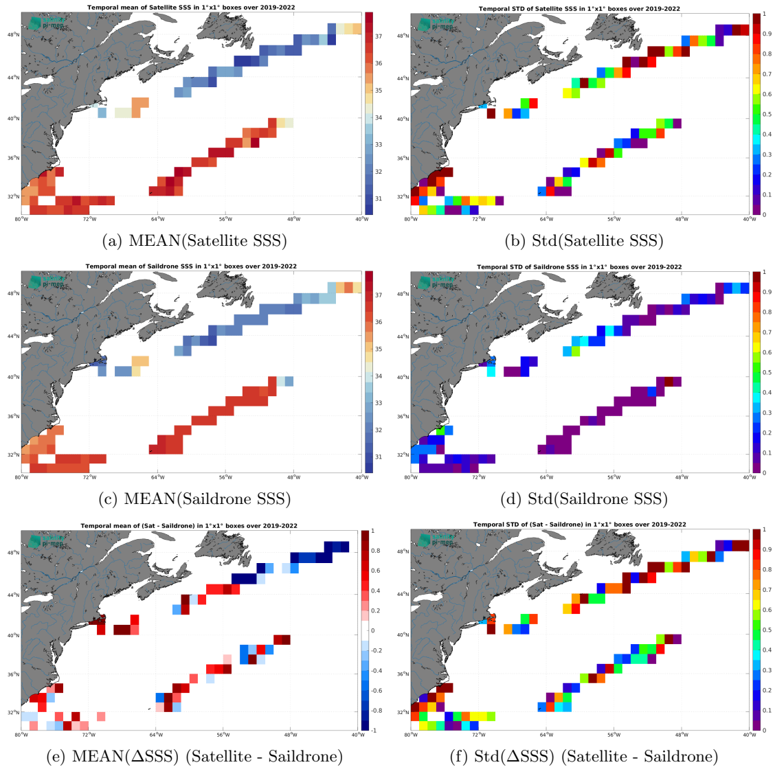
Figure 7: Temporal mean (left) and Std (right) of SSS from SMAP SSS L2 v5.3 - 40 km (RSS) (top), Saildrone (middle), and of \Delta SSS (Satellite - Saildrone). Only match-up pairs are used to generate these maps.
