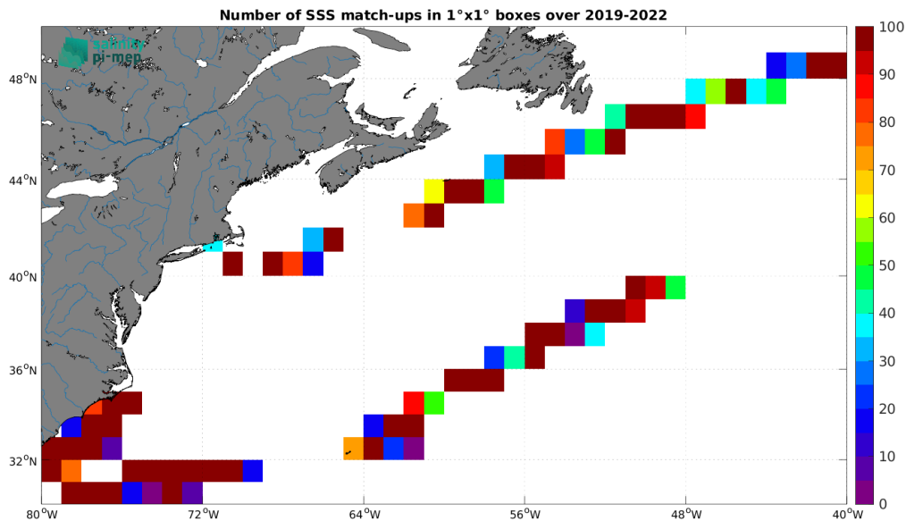
Figure 5: Number of SSS match-ups between Saildrone SSS and the SMAP SSS L2 v5.3 - 40 km (RSS) SSS product for the Gulf Stream Pi-MEP region over 1^\circ \times 1^\circ boxes and for the full satellite product period.
