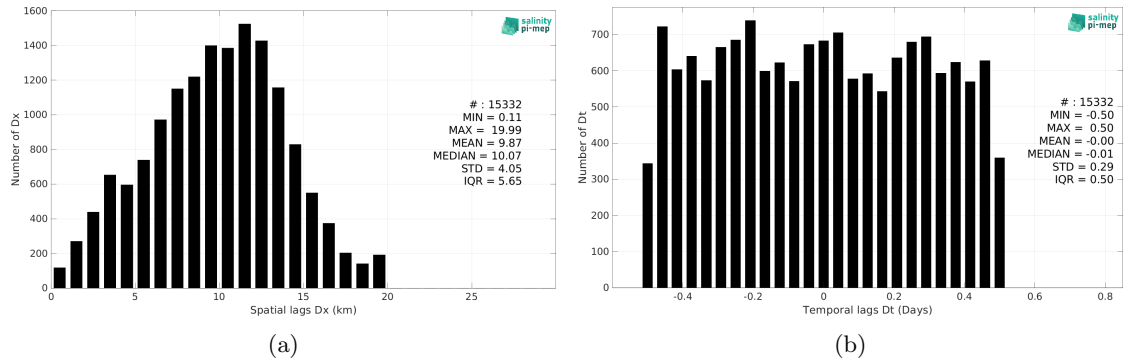
Figure 6: Histograms of the spatial (a) and temporal (b) lags between the location/time of the Sairdronne measurement and the date of the corresponding SMAP SSS L2 v5.3 - 40 km (RSS) SSS pixel.
