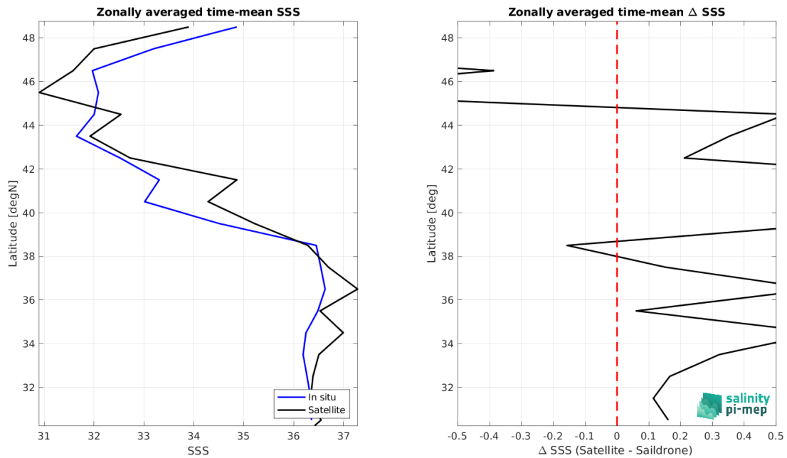
Figure 9: Left panel: Zonal mean SSS from SMAP SSS L2 v5.3 - 40 km (RSS) satellite product (black) and from Saildrone (blue). Right panel: Zonal mean of \Delta SSS (Satellite - Saildrone) for all the collected Pi-MEP match-up pairs estimated over the full satellite product period.
