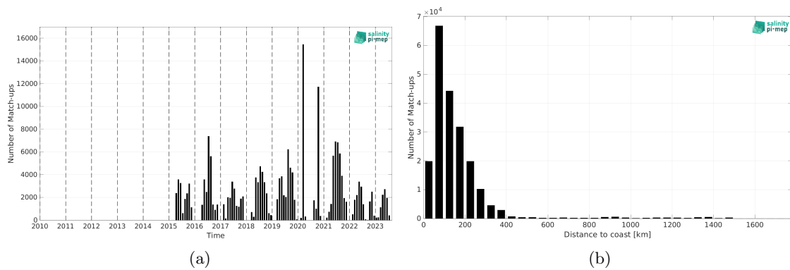
Figure 1: Number of match-ups between TSG (SAMOS) and SMAP SSS L2 v5 - 40 km (RSS) SSS as a function of time (a) and as function of the distance to coast (b) over the Gulf Stream Pi-MEP region and for the full satellite product period.
