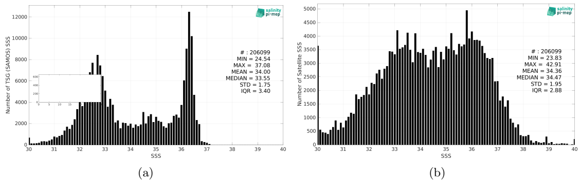
Figure 2: Histograms of SSS from TSG (SAMOS) (a) and SMAP SSS L2 v5 - 40 km (RSS) (b) considering all match-up pairs per bins of 0.1 over the Gulf Stream Pi-MEP region and for the full satellite product period.
