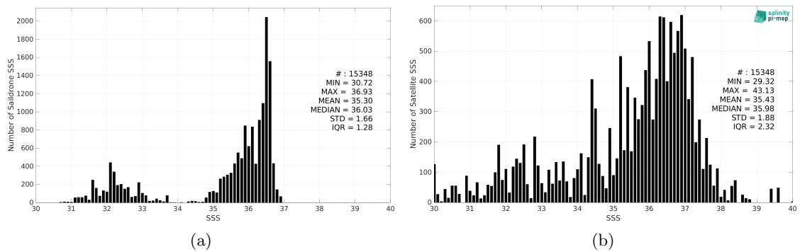
Figure 2: Histograms of SSS from Sairdrone (a) and SMAP SSS L2 v5 - 40 km (RSS) (b) considering all match-up pairs per bins of 0.1 over the Gulf Stream Pi-MEP region and for the full satellite product period.
