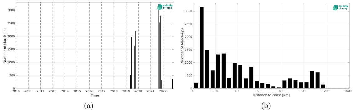
Figure 1: Number of match-ups between Sairdrone and SMAP SSS L2 v5 - 40 km (RSS) SSS as a function of time (a) and as function of the distance to coast (b) over the Gulf Stream Pi-MEP region and for the full satellite product period.
