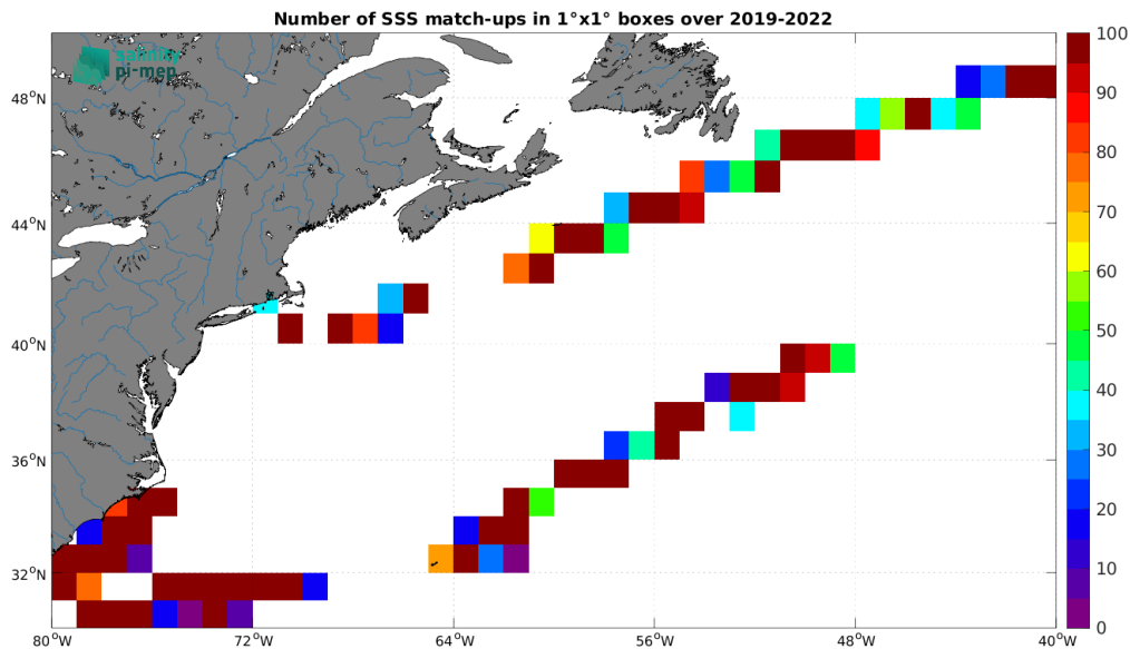
Figure 4: Number of SSS match-ups between Saildrone SSS and the SMAP SSS L2 v5 - 40 km (RSS) SSS product for the Gulf Stream Pi-MEP region over 1^\circ \times 1^\circ boxes and for the full satellite product period.
