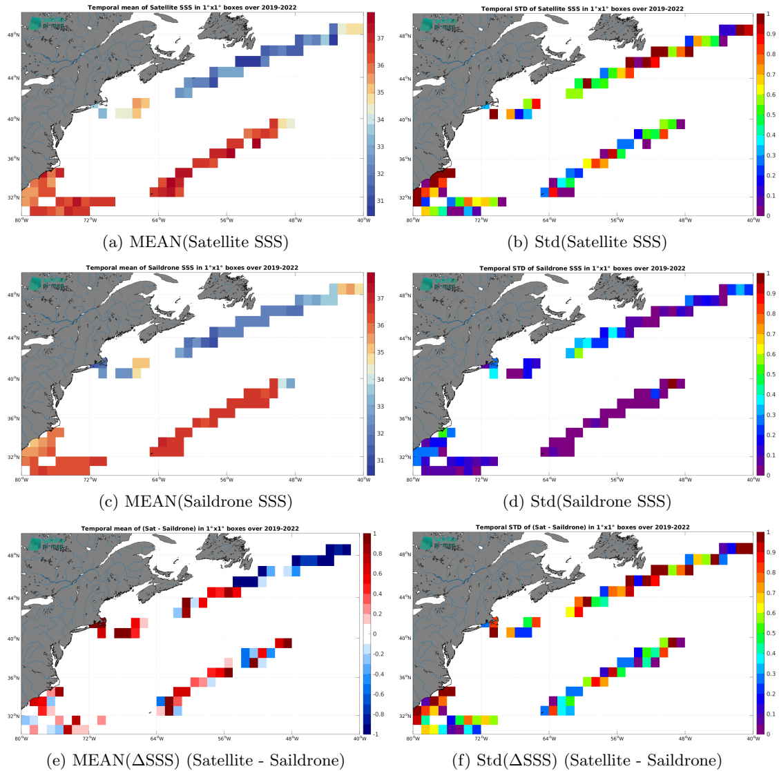
Figure 6: Temporal mean (left) and Std (right) of SSS from SMAP SSS L2 v5 - 40 km (RSS) (top), Saildrone (middle), and of \Delta SSS (Satellite - Saildrone). Only match-up pairs are used to generate these maps.
