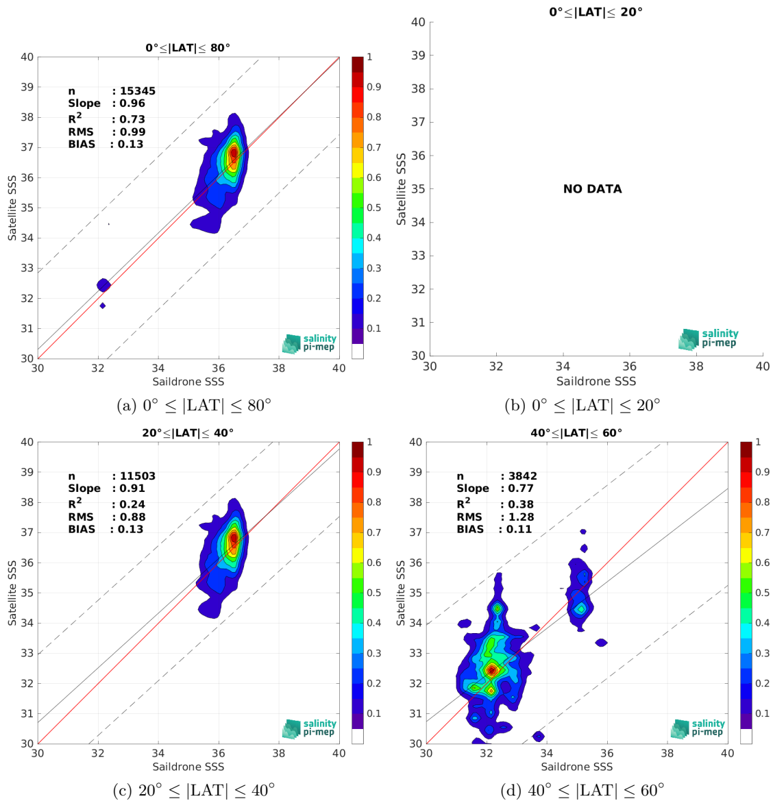
Figure 9: Contour maps of the concentration of SMAP SSS L2 v5 - 40 km (RSS) SSS (y-axis) versus Saildrone SSS (x-axis) at match-up pairs for different latitude bands. For each plot, the red line shows x=y . The black thin and dashed lines indicate a linear fit through the data cloud and the \pm 95\% confidence levels, respectively. The number match-up pairs n , the slope and R^2 coefficient of the linear fit, the root mean square (RMS) and the mean bias between satellite and in situ data are indicated for each latitude band in each plots.
