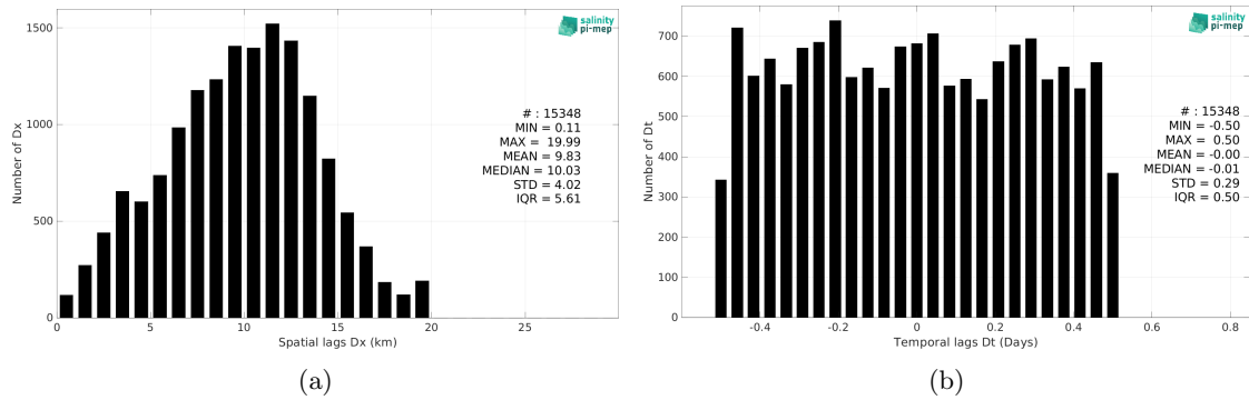
Figure 5: Histograms of the spatial (a) and temporal (b) lags between the location/time of the Saildrone measurement and the date of the corresponding SMAP SSS L2 v5 - 40 km (RSS) SSS pixel.
