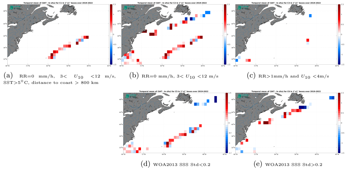
Figure 12: Temporal mean gridded over spatial boxes of size 1^\circ \times 1^\circ of \Delta SSS (SMAP SSS L2 v5 - 40 km (RSS) - Sairdrone) for 5 different subdatasets corresponding to:RR=0 mm/h, 3 < U_{10} < 12 m/s, SST >5^\circ C , distance to coast > 800 km (a), RR=0 mm/h, 3 < U_{10} < 12 m/s (b), RR >1 mm/h and U_{10} < 4 m/s (c), WOA2013 SSS Std <0.2 (d), WOA2013 SSS Std >0.2 (e).
