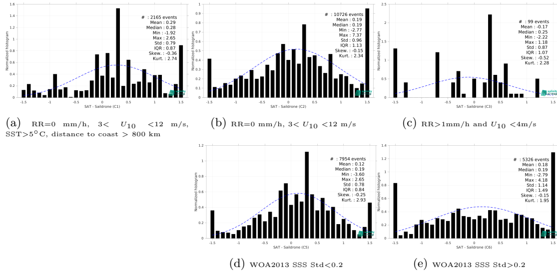
Figure 13: Normalized histogram of \Delta SSS (SMAP SSS L2 v5 - 40 km (RSS) - Saildrone) for 5 different subdatasets corresponding to: RR=0 mm/h, 3 < U_{10} < 12 m/s, SST>5°C, distance to coast > 800 km (a), RR=0 mm/h, 3 < U_{10} < 12 m/s (b), RR>1mm/h and U_{10} < 4 m/s (c), WOA2013 SSS Std<0.2 (d), WOA2013 SSS Std>0.2 (e).
