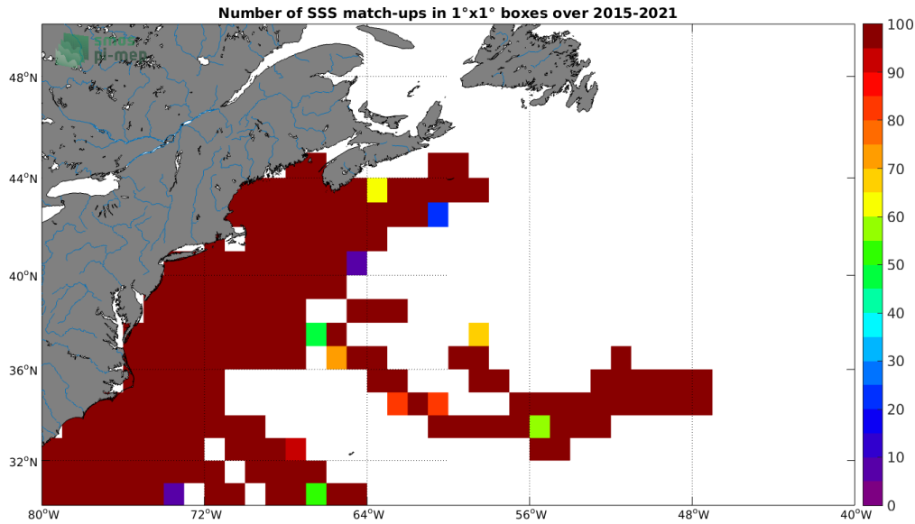
Figure 4: Number of SSS match-ups between TSG (SAMOS) SSS and the SMAP SSS L2 v4 (RSS) SSS product for the Gulf Stream Pi-MEP region over 1^\circ \times 1^\circ boxes and for the full satellite product period.
