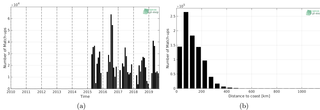
Figure 1: Number of match-ups between TSG-SAMOS and SMAP-L2-RSS-V4 SSS as a function of time (a) and as function of the distance to coast (b) over the Gulf Stream Pi-MEP region and for the full satellite product period.
