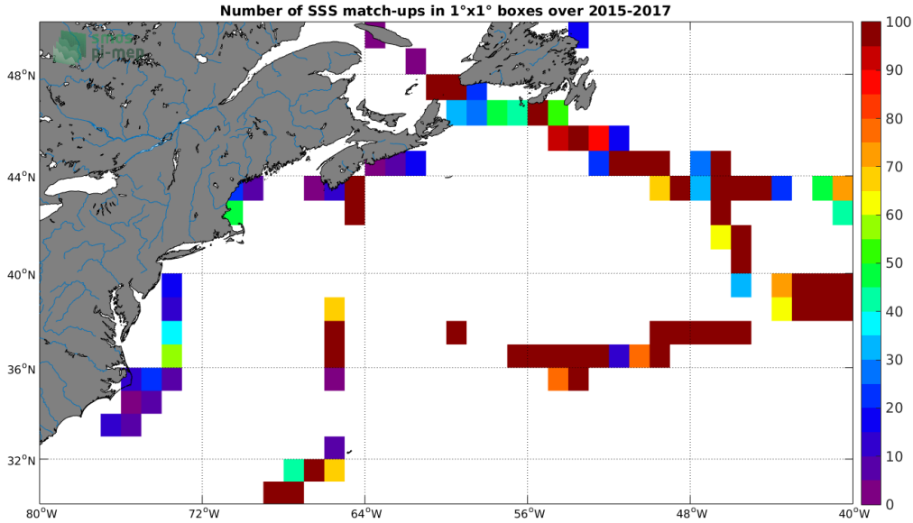
Figure 4: Number of SSS match-ups between TSG (GOSUD-Sailing-ship) SSS and the SMAP SSS L2 v4 (RSS) SSS product for the Gulf Stream Pi-MEP region over 1°x1° boxes and for the full satellite product period.
