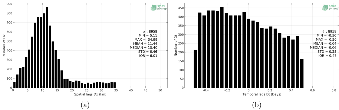
Figure 5: Histograms of the spatial (a) and temporal (b) lags between the time of the TSG (GOSUD-Sailing-ship) measurements and the date of the corresponding SMAP SSS L2 v4 (RSS) SSS product.
