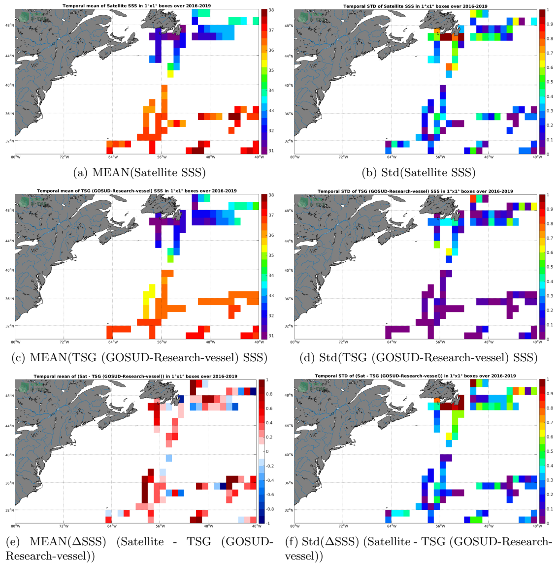
Figure 6: Temporal mean (left) and Std (right) of SSS from SMAP SSS L2 v4 (RSS) (top), TSG (GOSUD-Research-vessel) (middle), and of \Delta\text{SSS} (Satellite - TSG (GOSUD-Research-vessel)). Only match-up pairs are used to generate these maps.
