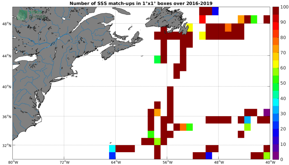
Figure 4: Number of SSS match-ups between TSG (GOSUD-Research-vessel) SSS and the SMAP SSS L2 v4 (RSS) SSS product for the Gulf Stream Pi-MEP region over 1°x1° boxes and for the full satellite product period.
