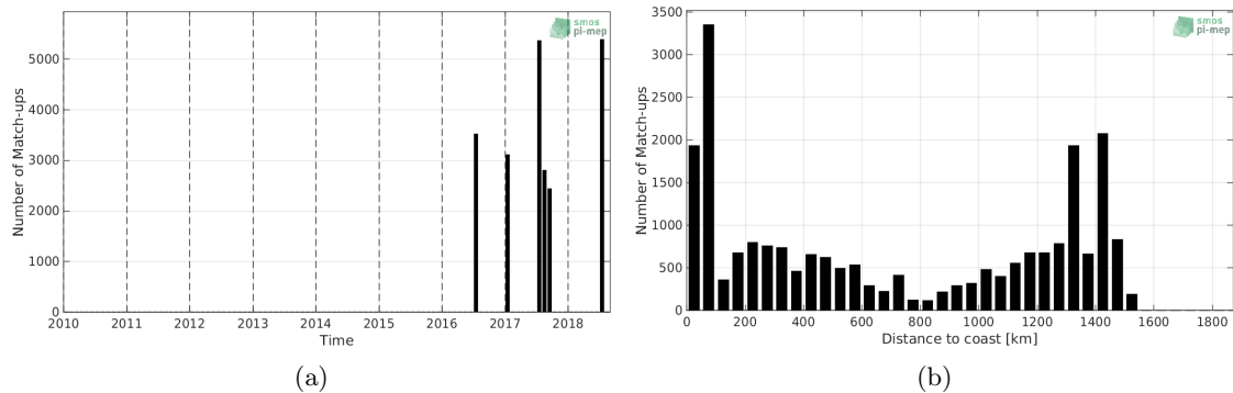
Figure 1: Number of match-ups between TSG-GOSUD-Research-vessel and SMAP-L2-RSS-V4 SSS as a function of time (a) and as function of the distance to coast (b) over the Gulf Stream Pi-MEP region and for the full satellite product period.
