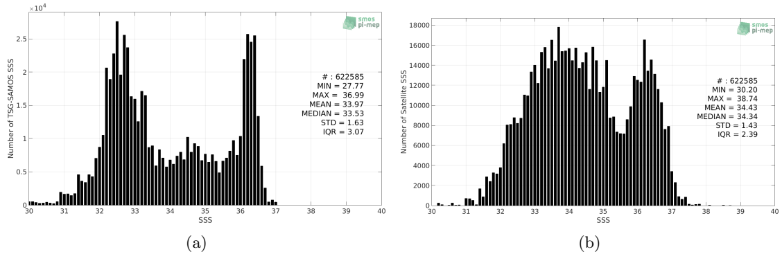
Figure 2: Histograms of SSS from TSG-SAMOS (a) and SMAP-L2-RSS-V3-70KM (b) considering all match-up pairs per bins of 0.1 over the Gulf Stream Pi-MEP region and for the full satellite product period.
