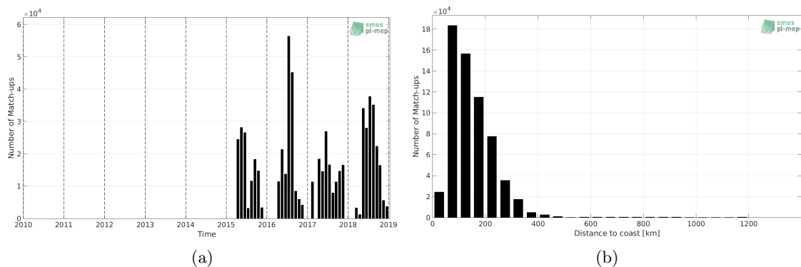
Figure 1: Number of match-ups between TSG-SAMOS and SMAP-L2-RSS-V3-70KM SSS as a function of time (a) and as function of the distance to coast (b) over the Gulf Stream Pi-MEP region and for the full satellite product period.
