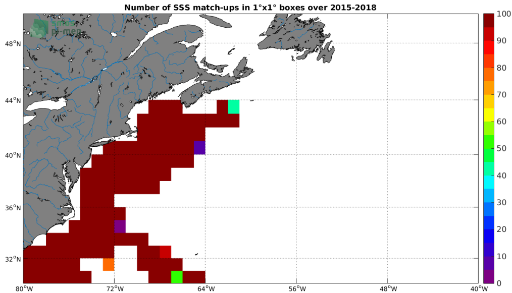
Figure 4: Number of SSS match-ups between TSG-SAMOS SSS and the SMAP-L2-RSS-V3-70KM SSS product for the Gulf Stream Pi-MEP region over 1^\circ \times 1^\circ boxes and for the full satellite product period.
