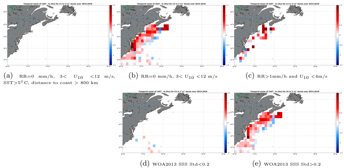
Figure 12: Temporal mean gridded over spatial boxes of size 1^\circ \times 1^\circ of \Delta SSS (SMAP-L2-RSS-V3-70KM - TSG-SAMOS) for 5 different subdatasets corresponding to:RR=0 mm/h, 3 < U_{10} < 12 m/s, SST >5^\circ C, distance to coast > 800 km (a), RR=0 mm/h, 3 < U_{10} < 12 m/s (b), RR >1 mm/h and U_{10} < 4 m/s (c), WOA2013 SSS Std <0.2 (d), WOA2013 SSS Std >0.2 (e).
