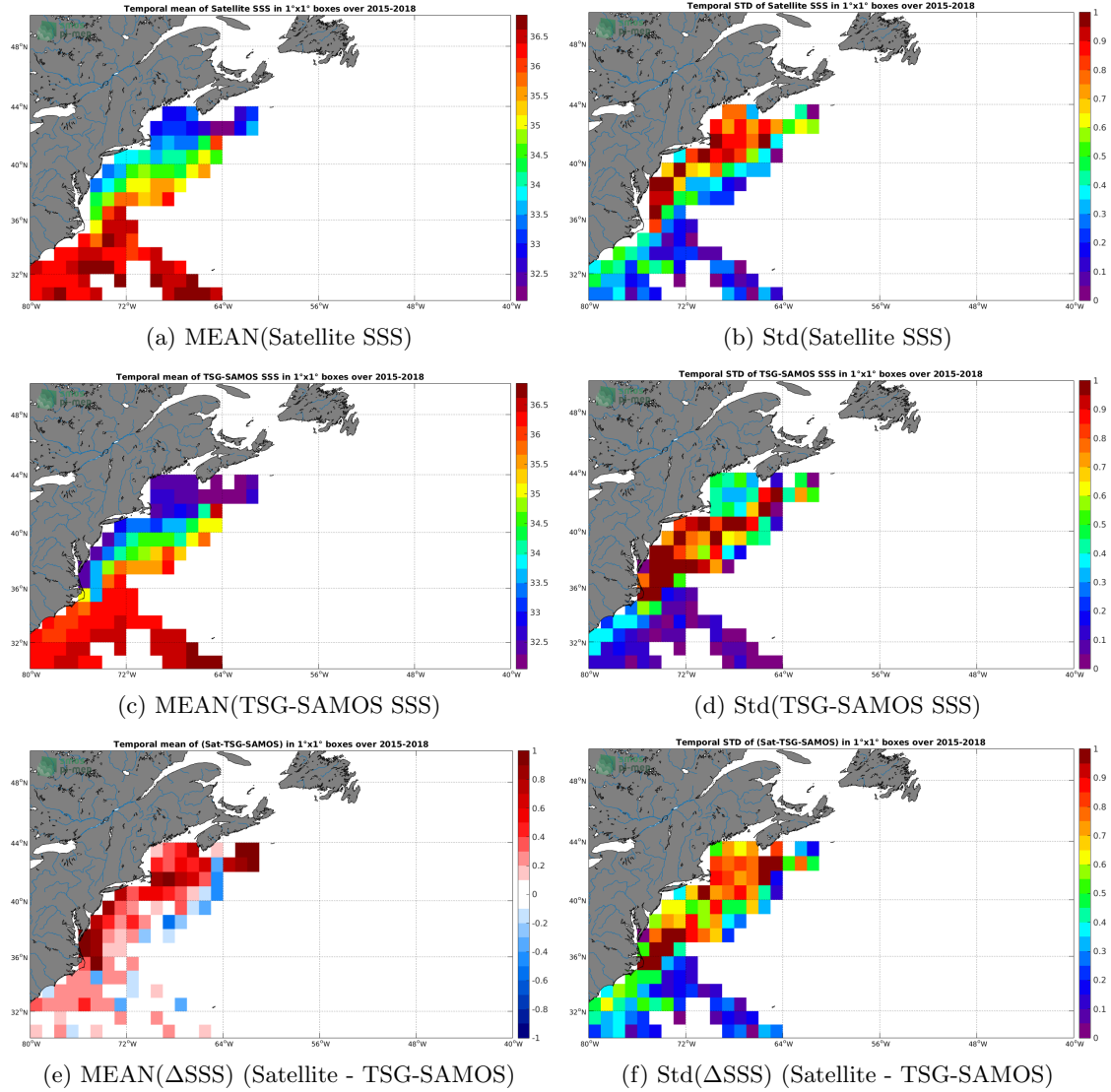
Figure 6: Temporal mean (left) and Std (right) of SSS from SMAP-L2-RSS-V3-70KM (top), TSG-SAMOS (middle), and of \Delta\text{SSS} (Satellite - TSG-SAMOS). Only match-up pairs are used to generate these maps.
