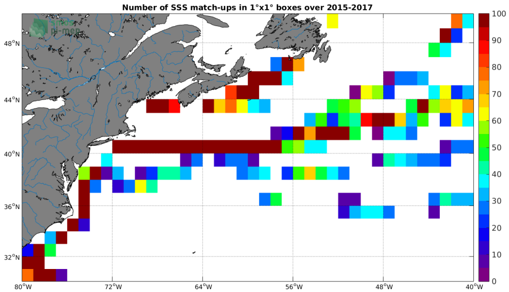
Figure 4: Number of SSS match-ups between TSG-LEGOS-DM SSS and the SMAP-L2-RSS-V3-70KM SSS product for the Gulf Stream Pi-MEP region over 1°x1° boxes and for the full satellite product period.
