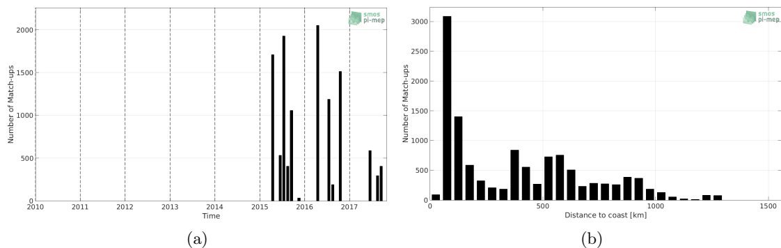
Figure 1: Number of match-ups between TSG-LEGOS-DM and SMAP-L2-RSS-V3-70KM SSS as a function of time (a) and as function of the distance to coast (b) over the Gulf Stream Pi-MEP region and for the full satellite product period.
