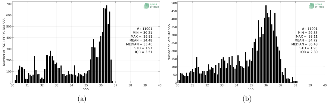
Figure 2: Histograms of SSS from TSG-LEGOS-DM (a) and SMAP-L2-RSS-V3-70KM (b) considering all match-up pairs per bins of 0.1 over the Gulf Stream Pi-MEP region and for the full satellite product period.
