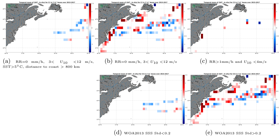
Figure 12: Temporal mean gridded over spatial boxes of size 1^\circ \times 1^\circ of \Delta SSS (SMAP-L2-RSS-V3-70KM - TSG-LEGOS-DM) for 5 different subdatasets corresponding to:RR=0 mm/h, 3 < U_{10} < 12 m/s, SST >5^\circ C, distance to coast > 800 km (a), RR=0 mm/h, 3 < U_{10} < 12 m/s (b), RR >1 mm/h and U_{10} < 4 m/s (c), WOA2013 SSS Std <0.2 (d), WOA2013 SSS Std >0.2 (e).
