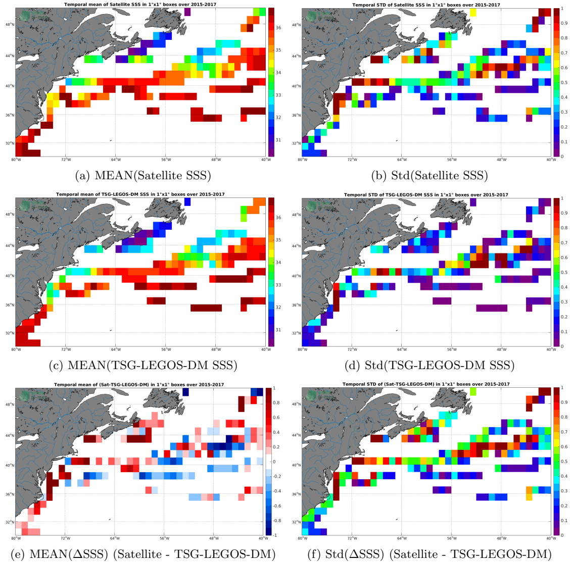
Figure 6: Temporal mean (left) and Std (right) of SSS from SMAP-L2-RSS-V3-70KM (top), TSG-LEGOS-DM (middle), and of \Delta SSS (Satellite - TSG-LEGOS-DM). Only match-up pairs are used to generate these maps.
