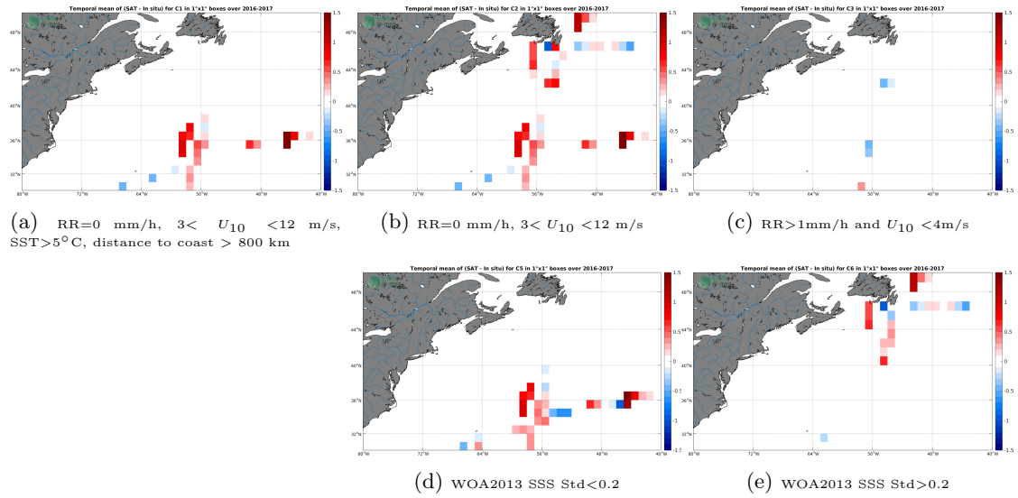
Figure 12: Temporal mean gridded over spatial boxes of size 1^\circ \times 1^\circ of \Delta SSS (SMAP-L2-RSS-V3-70KM - TSG-GOSUD-Research-vessel) for 5 different subdatasets corresponding to:RR=0 mm/h, 3 < U_{10} < 12 m/s, SST >5^\circ C, distance to coast > 800 km (a), RR=0 mm/h, 3 < U_{10} < 12 m/s (b), RR >1 mm/h and U_{10} < 4 m/s (c), WOA2013 SSS Std <0.2 (d), WOA2013 SSS Std >0.2 (e).
