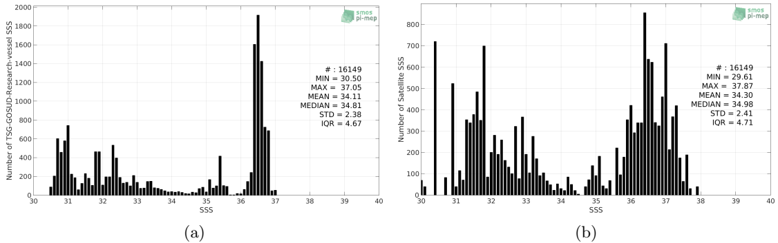
Figure 2: Histograms of SSS from TSG-GOSUD-Research-vessel (a) and SMAP-L2-RSS-V3-70KM (b) considering all match-up pairs per bins of 0.1 over the Gulf Stream Pi-MEP region and for the full satellite product period.
