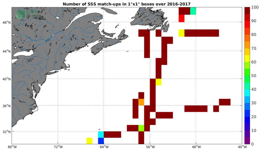
Figure 4: Number of SSS match-ups between TSG-GOSUD-Research-vessel SSS and the SMAP-L2-RSS-V3-70KM SSS product for the Gulf Stream Pi-MEP region over 1^\circ \times 1^\circ boxes and for the full satellite product period.
