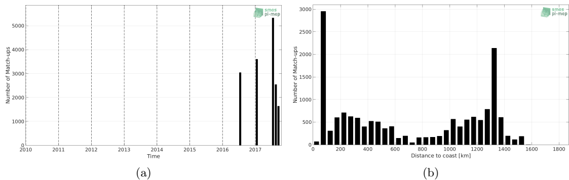
Figure 1: Number of match-ups between TSG-GOSUD-Research-vessel and SMAP-L2-RSS-V3-70KM SSS as a function of time (a) and as function of the distance to coast (b) over the Gulf Stream Pi-MEP region and for the full satellite product period.
