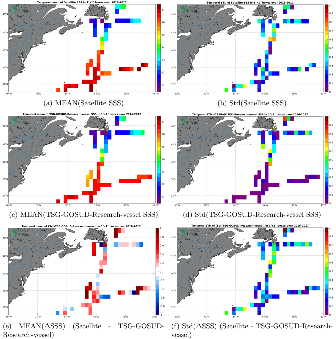
Figure 6: Temporal mean (left) and Std (right) of SSS from SMAP-L2-RSS-V3-70KM (top), TSG-GOSUD-Research-vessel (middle), and of \Delta SSS (Satellite - TSG-GOSUD-Research-vessel). Only match-up pairs are used to generate these maps.
