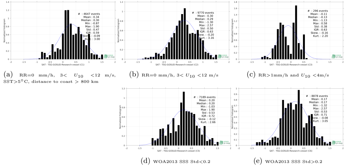
Figure 13: Normalized histogram of \Delta SSS (SMAP-L2-RSS-V3-70KM - TSG-GOSUD-Research-vessel) for 5 different subdatasets corresponding to: RR=0 mm/h, 3 < U_{10} < 12 m/s, SST > 5°C, distance to coast > 800 km (a), RR=0 mm/h, 3 < U_{10} < 12 m/s (b), RR > 1mm/h and U_{10} < 4 m/s (c), WOA2013 SSS Std < 0.2 (d), WOA2013 SSS Std > 0.2 (e).
