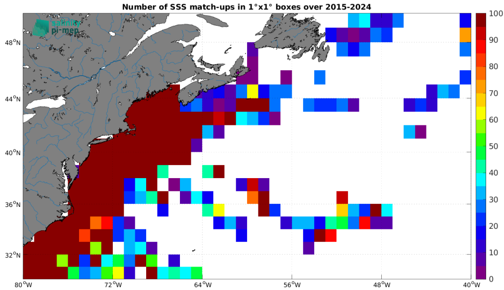
Figure 5: Number of SSS match-ups between TSG (SAMOS) SSS and the SMAP SSS L2 v5.0 (JPL) SSS product for the Gulf Stream Pi-MEP region over 1^\circ \times 1^\circ boxes and for the full satellite product period.
