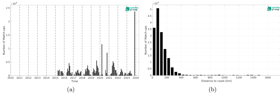
Figure 2: Number of match-ups between TSG (SAMOS) and SMAP SSS L2 v5.0 (JPL) SSS as a function of time (a) and as function of the distance to coast (b) over the Gulf Stream Pi-MEP region and for the full satellite product period.
