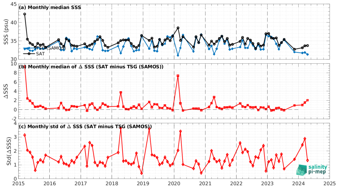
Figure 8: Time series of the monthly median SSS (top), median of \Delta\text{SSS} (Satellite - TSG (SAMOS)) and Std of \Delta\text{SSS} (Satellite - TSG (SAMOS)) over the Gulf Stream Pi-MEP region considering all match-ups collected by the Pi-MEP.
