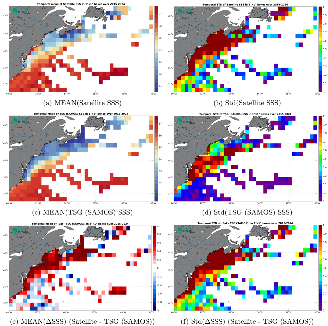
Figure 7: Temporal mean (left) and Std (right) of SSS from SMAP SSS L2 v5.0 (JPL) (top), TSG (SAMOS) (middle), and of \Delta SSS (Satellite - TSG (SAMOS)). Only match-up pairs are used to generate these maps.
