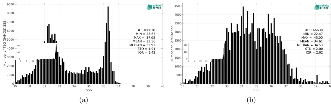
Figure 3: Histograms of SSS from TSG (SAMOS) (a) and SMAP SSS L2 v5.0 (JPL) (b) considering all match-up pairs per bins of 0.1 over the Gulf Stream Pi-MEP region and for the full satellite product period.
