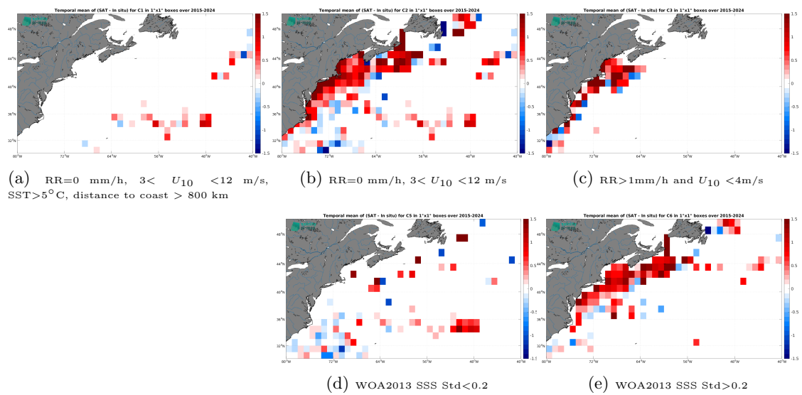
Figure 14: Temporal mean gridded over spatial boxes of size 1^\circ \times 1^\circ of \Delta SSS (SMAP SSS L2 v5.0 (JPL) - TSG (SAMOS)) for 5 different subdatasets corresponding to:RR=0 mm/h, 3 < U_{10} < 12 m/s, SST > 5°C, distance to coast > 800 km (a), RR=0 mm/h, 3 < U_{10} < 12 m/s (b), RR > 1mm/h and U_{10} < 4 m/s (c), WOA2013 SSS Std < 0.2 (d), WOA2013 SSS Std > 0.2 (e).
