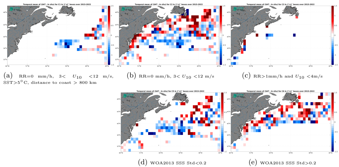
Figure 14: Temporal mean gridded over spatial boxes of size 1^\circ \times 1^\circ of \Delta SSS (SMAP SSS L2 v5.0 (JPL) - TSG (LEGOS-DM)) for 5 different subdatasets corresponding to: RR=0 mm/h, 3 < U_{10} < 12 m/s, SST > 5°C, distance to coast > 800 km (a), RR=0 mm/h, 3 < U_{10} < 12 m/s (b), RR > 1mm/h and U_{10} < 4 m/s (c), WOA2013 SSS Std < 0.2 (d), WOA2013 SSS Std > 0.2 (e).
