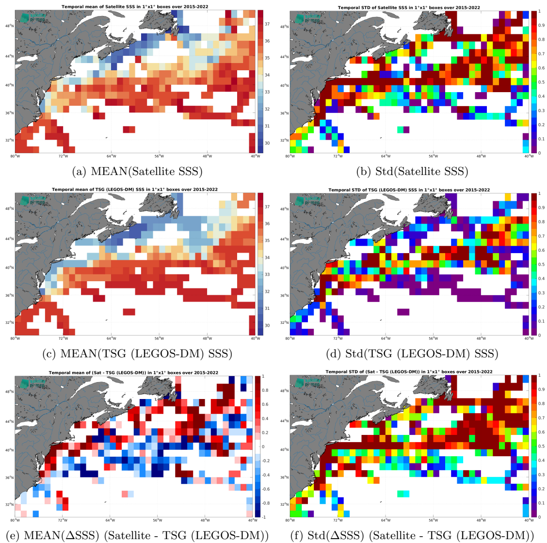
Figure 7: Temporal mean (left) and Std (right) of SSS from SMAP SSS L2 v5.0 (JPL) (top), TSG (LEGOS-DM) (middle), and of \Delta SSS (Satellite - TSG (LEGOS-DM)). Only match-up pairs are used to generate these maps.
