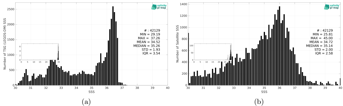
Figure 3: Histograms of SSS from TSG (LEGOS-DM) (a) and SMAP SSS L2 v5.0 (JPL) (b) considering all match-up pairs per bins of 0.1 over the Gulf Stream Pi-MEP region and for the full satellite product period.
