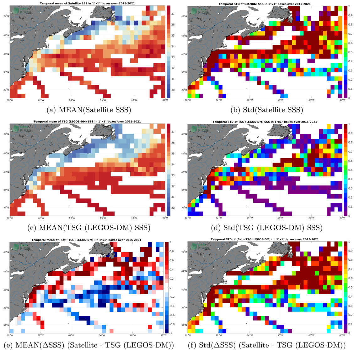
Figure 6: Temporal mean (left) and Std (right) of SSS from SMAP SSS L2 v5.0 (JPL) (top), TSG (LEGOS-DM) ( in situ ) (middle), and of \Delta SSS (Satellite - TSG (LEGOS-DM)). Only match-up pairs are used to generate these maps.
