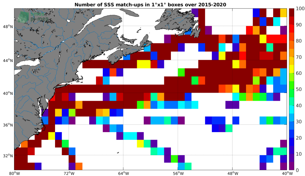
Figure 4: Number of SSS match-ups between TSG (LEGOS-DM) SSS and the SMAP SSS L2 v5.0 (JPL) SSS product for the Gulf Stream Pi-MEP region over 1°x1° boxes and for the full satellite product period.
