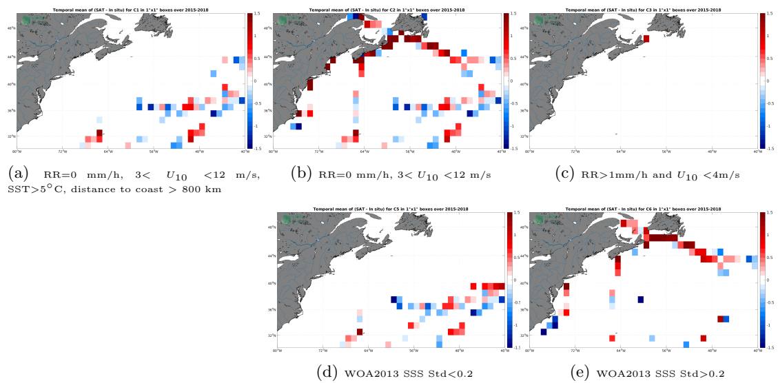
Figure 12: Temporal mean gridded over spatial boxes of size 1^\circ \times 1^\circ of \Delta SSS (SMAP SSS L2 v5.0 (JPL) - TSG (GOSUD-Sailing-ship)) for 5 different subdatasets corresponding to: RR=0 mm/h, 3 < U_{10} < 12 m/s, SST > 5°C, distance to coast > 800 km (a), RR=0 mm/h, 3 < U_{10} < 12 m/s (b), RR > 1mm/h and U_{10} < 4 m/s (c), WOA2013 SSS Std < 0.2 (d), WOA2013 SSS Std > 0.2 (e).
