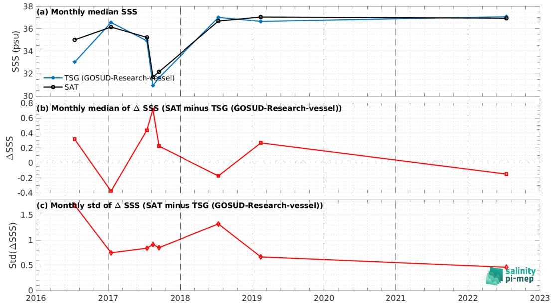
Figure 8: Time series of the monthly median SSS (top), median of \Delta SSS (Satellite - TSG (GOSUD-Research-vessel)) and Std of \Delta SSS (Satellite - TSG (GOSUD-Research-vessel)) over the Gulf Stream Pi-MEP region considering all match-ups collected by the Pi-MEP.
