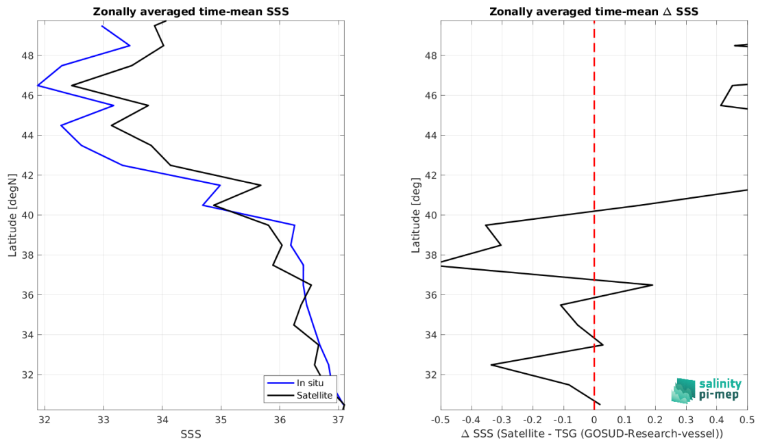
Figure 9: Left panel: Zonal mean SSS from SMAP SSS L2 v5.0 (JPL) satellite product (black) and from TSG (GOSUD-Research-vessel) (blue). Right panel: Zonal mean of \Delta SSS (Satellite - TSG (GOSUD-Research-vessel)) for all the collected Pi-MEP match-up pairs estimated over the full satellite product period.
