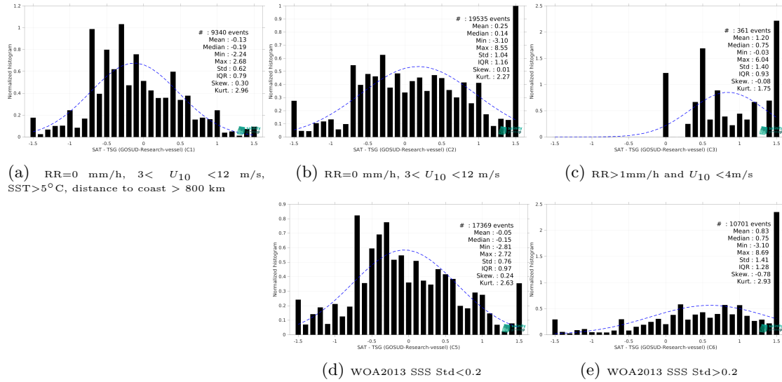
Figure 15: Normalized histogram of \Delta SSS (SMAP SSS L2 v5.0 (JPL) - TSG (GOSUD-Research-vessel)) for 5 different subdatasets corresponding to: RR=0 mm/h, 3 < U_{10} < 12 m/s, SST > 5°C, distance to coast > 800 km (a), RR=0 mm/h, 3 < U_{10} < 12 m/s (b), RR > 1mm/h and U_{10} < 4 m/s (c), WOA2013 SSS Std < 0.2 (d), WOA2013 SSS Std > 0.2 (e).
