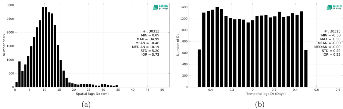
Figure 6: Histograms of the spatial (a) and temporal (b) lags between the location/time of the TSG (GOSUD-Research-vessel) measurement and the date of the corresponding SMAP SSS L2 v5.0 (JPL) SSS pixel.
