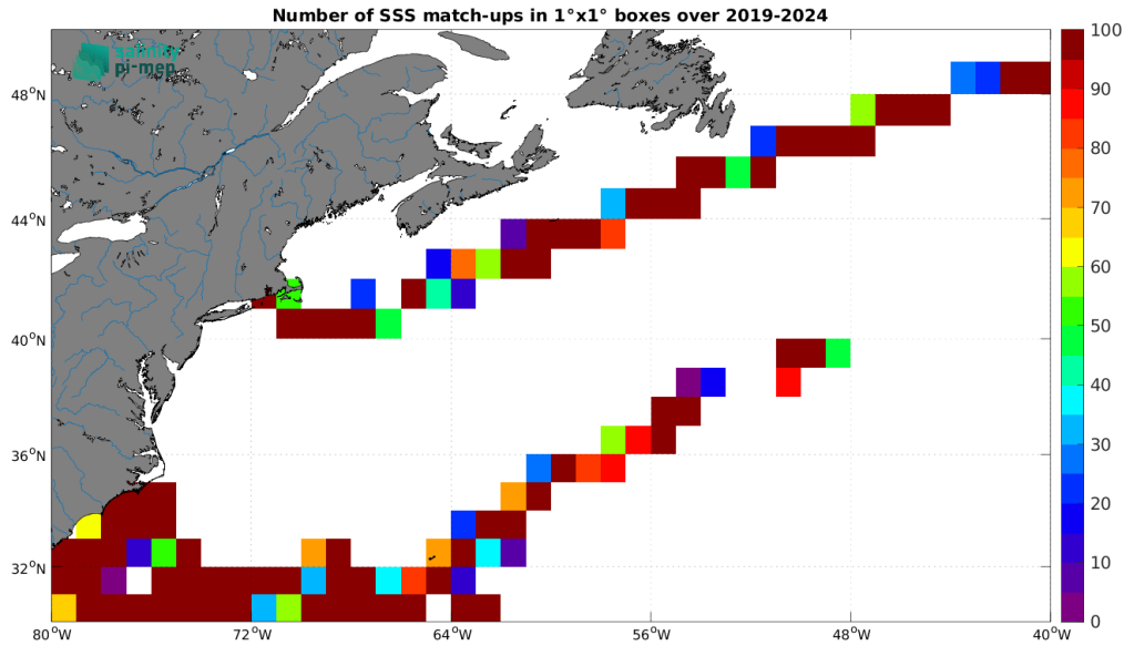
Figure 5: Number of SSS match-ups between Saildrone SSS and the SMAP SSS L2 v5.0 (JPL) SSS product for the Gulf Stream Pi-MEP region over 1^\circ \times 1^\circ boxes and for the full satellite product period.
