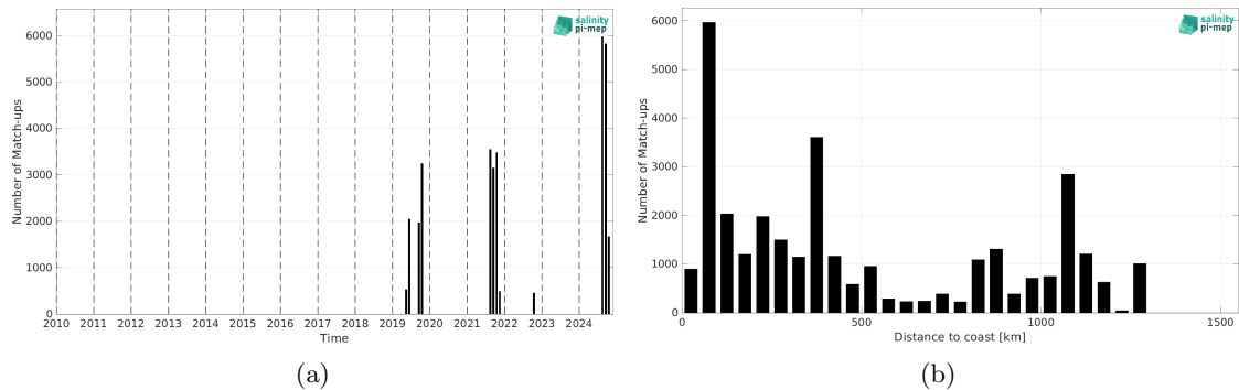
Figure 2: Number of match-ups between Saildrone and SMAP SSS L2 v5.0 (JPL) SSS as a function of time (a) and as function of the distance to coast (b) over the Gulf Stream Pi-MEP region and for the full satellite product period.
