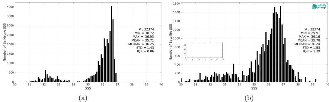
Figure 3: Histograms of SSS from Saildrone (a) and SMAP SSS L2 v5.0 (JPL) (b) considering all match-up pairs per bins of 0.1 over the Gulf Stream Pi-MEP region and for the full satellite product period.
