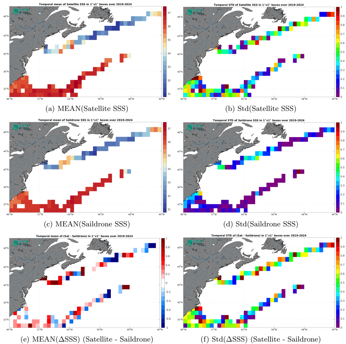
Figure 7: Temporal mean (left) and Std (right) of SSS from SMAP SSS L2 v5.0 (JPL) (top), Saildrone (middle), and of \Delta SSS (Satellite - Saildrone). Only match-up pairs are used to generate these maps.
