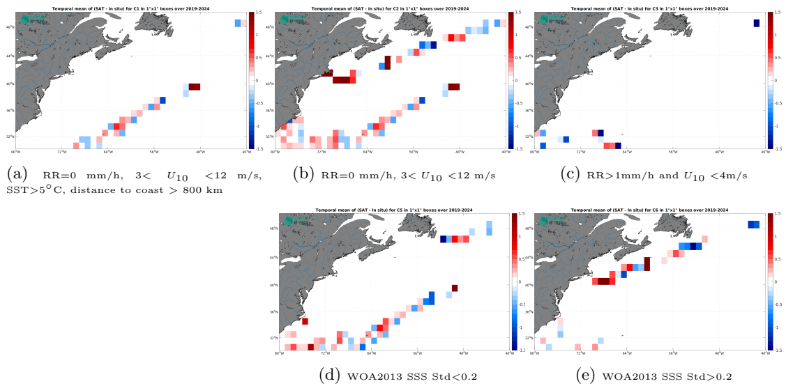
Figure 14: Temporal mean gridded over spatial boxes of size 1^\circ \times 1^\circ of \Delta SSS (SMAP SSS L2 v5.0 (JPL) - Saifdrone) for 5 different subdatasets corresponding to: RR=0 mm/h, 3 < U_{10} < 12 m/s, SST > 5°C, distance to coast > 800 km (a), RR=0 mm/h, 3 < U_{10} < 12 m/s (b), RR > 1mm/h and U_{10} < 4 m/s (c), WOA2013 SSS Std < 0.2 (d), WOA2013 SSS Std > 0.2 (e).
