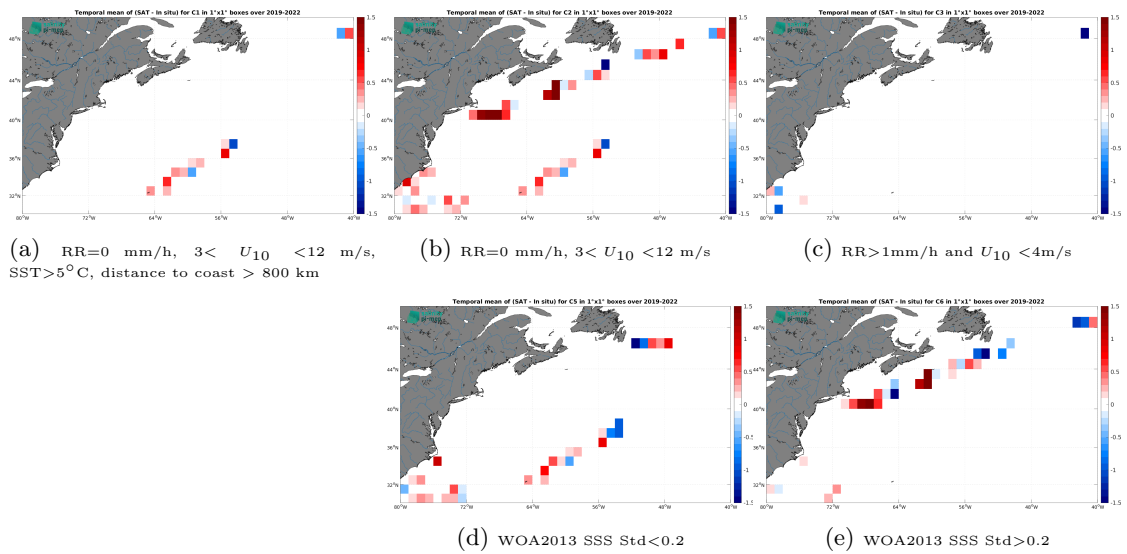
Figure 14: Temporal mean gridded over spatial boxes of size 1^\circ \times 1^\circ of \Delta SSS (SMAP SSS L2 v5.0 (JPL) - Saikrone) for 5 different subdatasets corresponding to: RR=0 mm/h, 3 < U_{10} < 12 m/s, SST > 5°C, distance to coast > 800 km (a), RR=0 mm/h, 3 < U_{10} < 12 m/s (b), RR > 1mm/h and U_{10} < 4 m/s (c), WOA2013 SSS Std < 0.2 (d), WOA2013 SSS Std > 0.2 (e).
