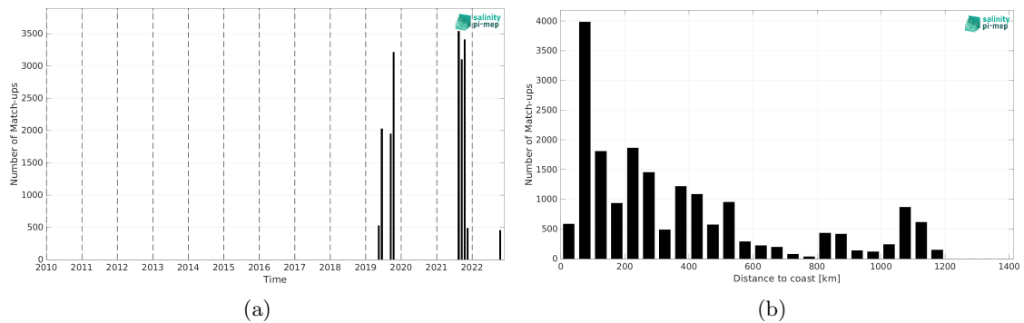
Figure 1: Number of match-ups between Sairdrone and SMAP SSS L2 v5.0 (JPL) SSS as a function of time (a) and as function of the distance to coast (b) over the Gulf Stream Pi-MEP region and for the full satellite product period.
