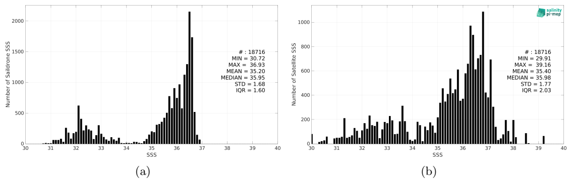
Figure 2: Histograms of SSS from Sairdrone (a) and SMAP SSS L2 v5.0 (JPL) (b) considering all match-up pairs per bins of 0.1 over the Gulf Stream Pi-MEP region and for the full satellite product period.
