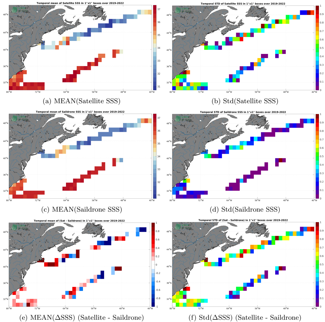
Figure 6: Temporal mean (left) and Std (right) of SSS from SMAP SSS L2 v5.0 (JPL) (top), Saildrone (middle), and of \Delta SSS (Satellite - Saildrone). Only match-up pairs are used to generate these maps.
