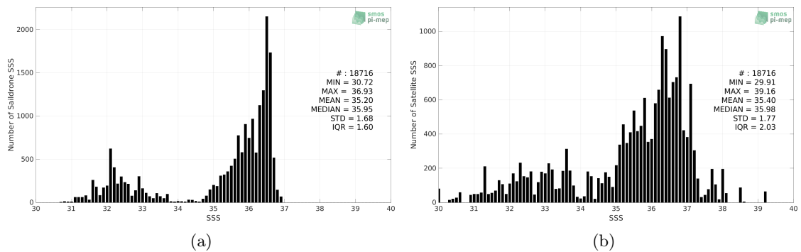
Figure 2: Histograms of SSS from Saildrone (a) and SMAP SSS L2 v5.0 (JPL) (b) considering all match-up pairs per bins of 0.1 over the Gulf Stream Pi-MEP region and for the full satellite product period.
