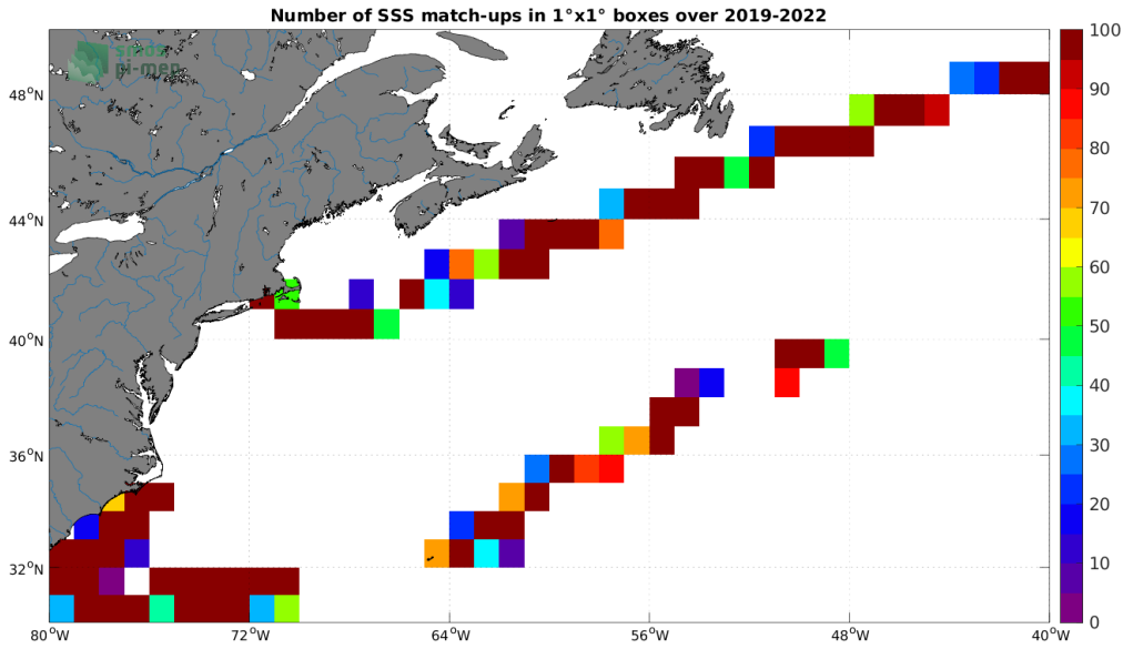
Figure 4: Number of SSS match-ups between Saildrone SSS and the SMAP SSS L2 v5.0 (JPL) SSS product for the Gulf Stream Pi-MEP region over 1^\circ \times 1^\circ boxes and for the full satellite product period.
