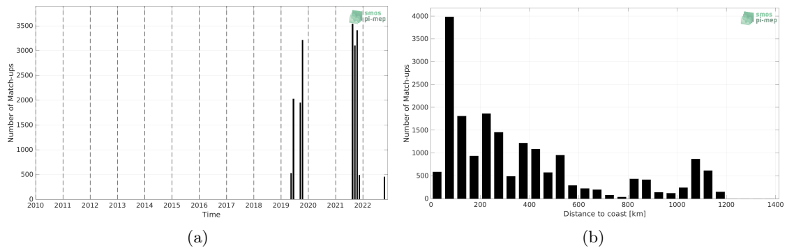
Figure 1: Number of match-ups between Saildrone and SMAP SSS L2 v5.0 (JPL) SSS as a function of time (a) and as function of the distance to coast (b) over the Gulf Stream Pi-MEP region and for the full satellite product period.
