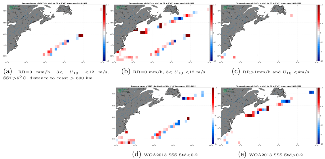
Figure 12: Temporal mean gridded over spatial boxes of size 1^\circ \times 1^\circ of \Delta SSS (SMAP SSS L2 v5.0 (JPL) - Saikrone) for 5 different subdatasets corresponding to:RR=0 mm/h, 3 < U_{10} < 12 m/s, SST >5^\circ C, distance to coast > 800 km (a), RR=0 mm/h, 3 < U_{10} < 12 m/s (b), RR >1 mm/h and U_{10} < 4 m/s (c), WOA2013 SSS Std <0.2 (d), WOA2013 SSS Std >0.2 (e).
