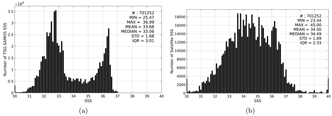
Figure 2: Histograms of SSS from TSG-SAMOS (a) and SMAP-L2-JPL-V4 (b) considering all match-up pairs per bins of 0.1 over the Gulf Stream Pi-MEP region and for the full satellite product period.
