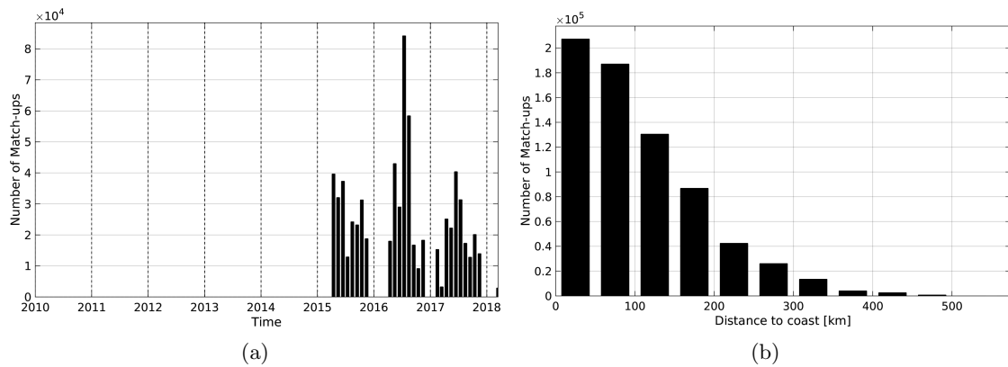
Figure 1: Number of match-ups between TSG-SAMOS and SMAP-L2-JPL-V4 SSS as a function of time (a) and as function of the distance to coast (b) over the Gulf Stream Pi-MEP region and for the full satellite product period.
