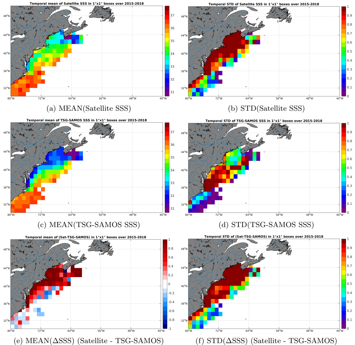
Figure 6: Temporal mean (left) and STD (right) of SSS from SMAP-L2-JPL-V4 (top), TSG-SAMOS (middle), and of \Delta SSS (Satellite - TSG-SAMOS). Only match-up pairs are used to generate these maps.
