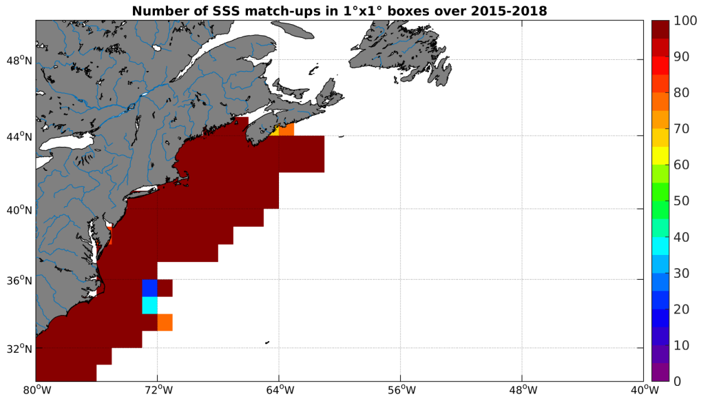
Figure 4: Number of SSS match-ups between TSG-SAMOS SSS and the SMAP-L2-JPL-V4 SSS product for the Gulf Stream Pi-MEP region over 1°x1° boxes and for the full satellite product period.
