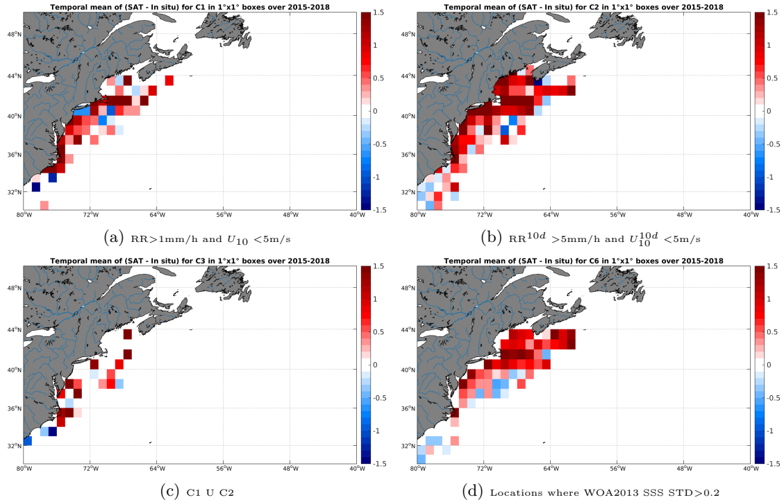
Figure 12: Temporal mean gridded over spatial boxes of size 1^\circ \times 1^\circ of \Delta SSS (SMAP-L2-JPL-V4 - TSG-SAMOS) for 4 different subdatasets corresponding to: RR > 1\text{mm/h} and U_{10} < 5\text{m/s} (a), RR^{10d} > 5\text{mm/h} and U_{10}^{10d} < 5\text{m/s} (b), C1 U C2 (c), Locations where WOA2013 SSS STD > 0.2 (d).
