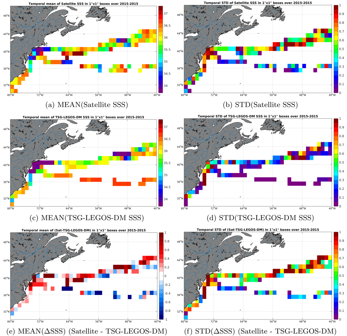
Figure 6: Temporal mean (left) and STD (right) of SSS from SMAP-L2-JPL-V4 (top), TSG-LEGOS-DM (middle), and of \Delta SSS (Satellite - TSG-LEGOS-DM). Only match-up pairs are used to generate these maps.
