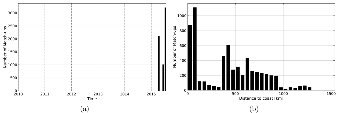
Figure 1: Number of match-ups between TSG-LEGOS-DM and SMAP-L2-JPL-V4 SSS as a function of time (a) and as function of the distance to coast (b) over the Gulf Stream Pi-MEP region and for the full satellite product period.
