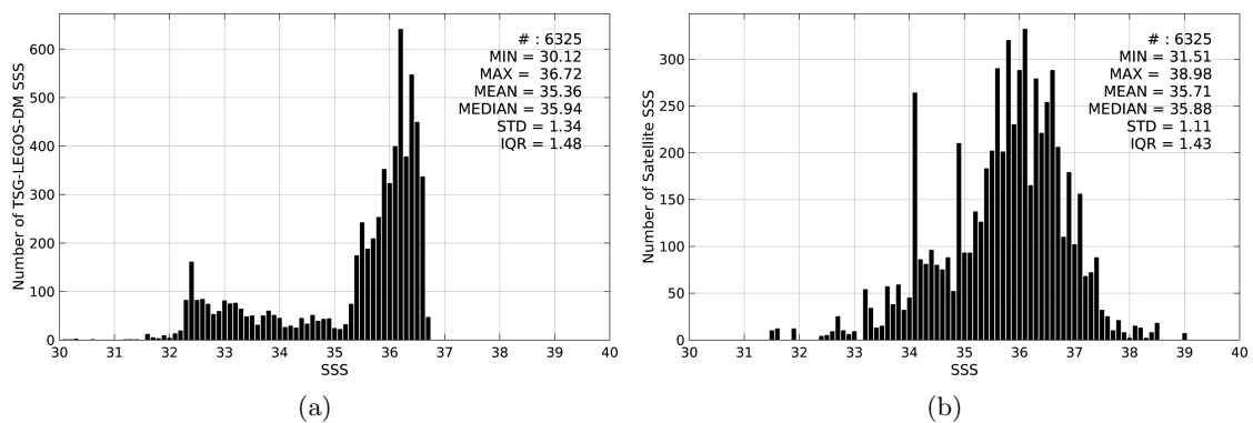
Figure 2: Histograms of SSS from TSG-LEGOS-DM (a) and SMAP-L2-JPL-V4 (b) considering all match-up pairs per bins of 0.1 over the Gulf Stream Pi-MEP region and for the full satellite product period.
