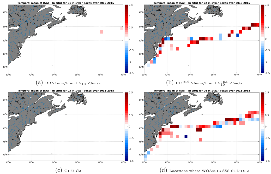
Figure 12: Temporal mean gridded over spatial boxes of size 1^\circ \times 1^\circ of \Delta SSS (SMAP-L2-JPL-V4 - TSG-LEGOS-DM) for 4 different subdatasets corresponding to: RR > 1mm/h and U_{10} < 5\text{m/s} (a), RR^{10d} > 5\text{mm/h} and U_{10}^{10d} < 5\text{m/s} (b), C1 U C2 (c), Locations where WOA2013 SSS STD > 0.2 (d).
