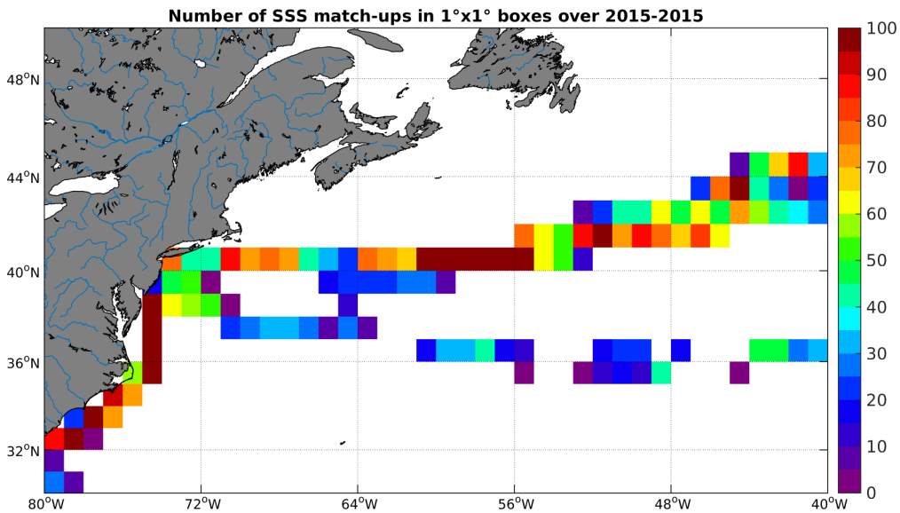
Figure 4: Number of SSS match-ups between TSG-LEGOS-DM SSS and the SMAP-L2-JPL-V4 SSS product for the Gulf Stream Pi-MEP region over 1^\circ \times 1^\circ boxes and for the full satellite product period.
