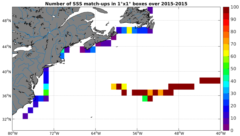
Figure 4: Number of SSS match-ups between TSG-GOSUD-Sailing-ship SSS and the SMAP-L2-JPL-V4 SSS product for the Gulf Stream Pi-MEP region over 1°x1° boxes and for the full satellite product period.
