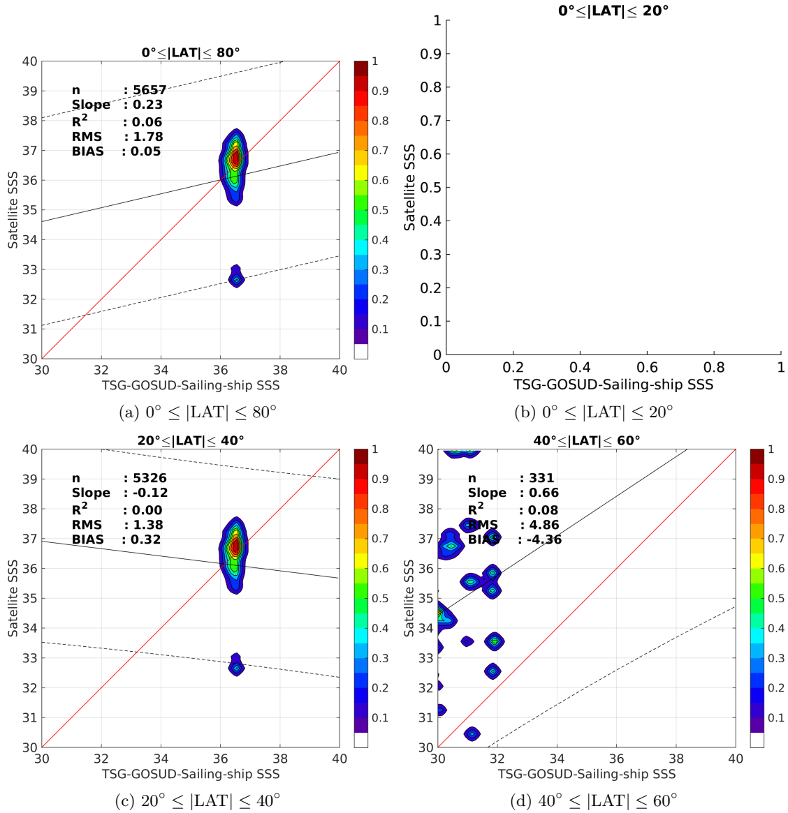
Figure 9: Contour maps of the concentration of SMAP-L2-JPL-V4 SSS (y-axis) versus TSG-GOSUD-Sailing-ship SSS (x-axis) at match-up pairs for different latitude bands. For each plot, the red line shows x=y . The black thin and dashed lines indicate a linear fit through the data cloud and the \pm 95\% confidence levels, respectively. The number match-up pairs n , the slope and R^2 coefficient of the linear fit, the root mean square (RMS) and the mean bias between satellite and in situ data are indicated for each latitude band in each plots.
