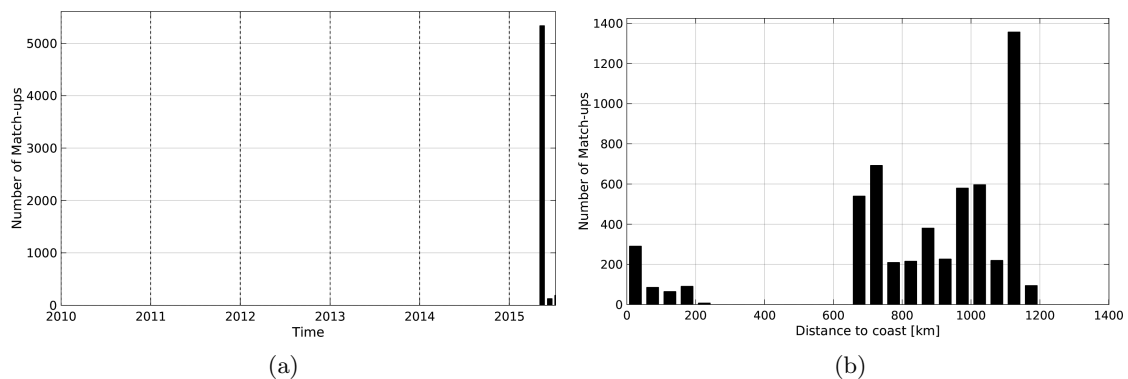
Figure 1: Number of match-ups between TSG-GOSUD-Sailing-ship and SMAP-L2-JPL-V4 SSS as a function of time (a) and as function of the distance to coast (b) over the Gulf Stream Pi-MEP region and for the full satellite product period.
