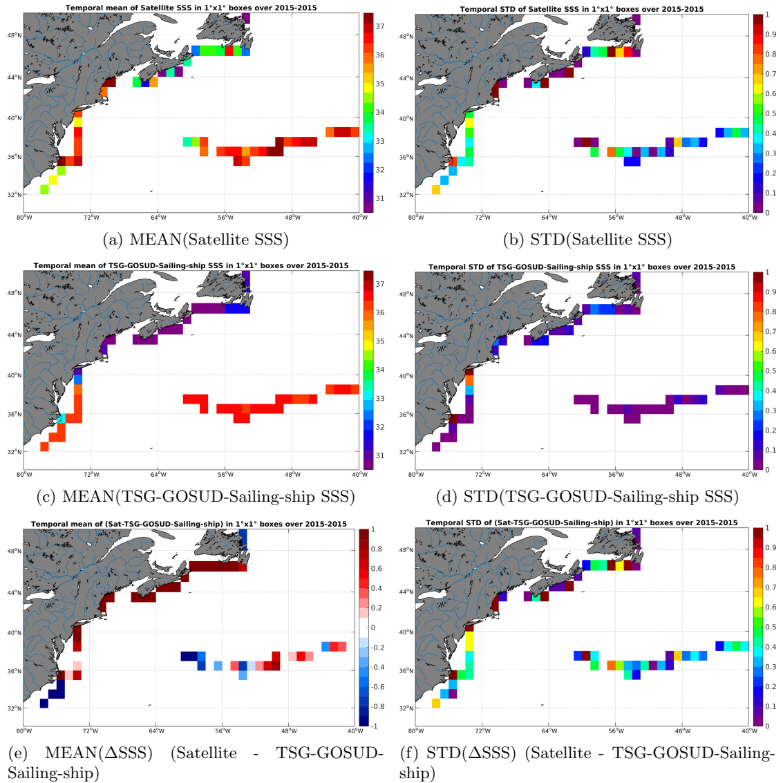
Figure 6: Temporal mean (left) and STD (right) of SSS from SMAP-L2-JPL-V4 (top), TSG-GOSUD-Sailing-ship (middle), and of \Delta SSS (Satellite - TSG-GOSUD-Sailing-ship). Only match-up pairs are used to generate these maps.
