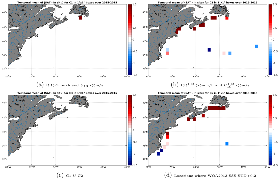
Figure 12: Temporal mean gridded over spatial boxes of size 1°x1° of \Delta SSS (SMAP-L2-JPL-V4 - TSG-GOSUD-Sailing-ship) for 4 different subdatasets corresponding to:RR>1mm/h and U_{10} < 5\text{m/s} (a), RR^{10d} > 5\text{mm/h} and U_{10}^{10d} < 5\text{m/s} (b), C1 U C2 (c),Locations where WOA2013 SSS STD>0.2 (d).
