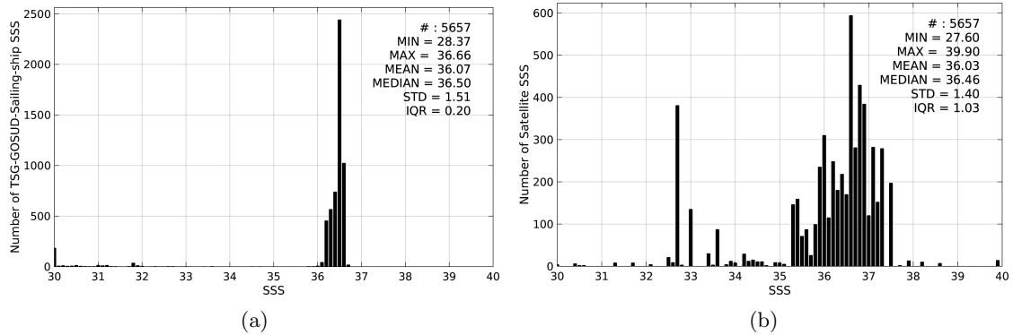
Figure 2: Histograms of SSS from TSG-GOSUD-Sailing-ship (a) and SMAP-L2-JPL-V4 (b) considering all match-up pairs per bins of 0.1 over the Gulf Stream Pi-MEP region and for the full satellite product period.
