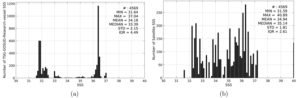
Figure 2: Histograms of SSS from TSG-GOSUD-Research-vessel (a) and SMAP-L2-JPL-V4 (b) considering all match-up pairs per bins of 0.1 over the Gulf Stream Pi-MEP region and for the full satellite product period.
