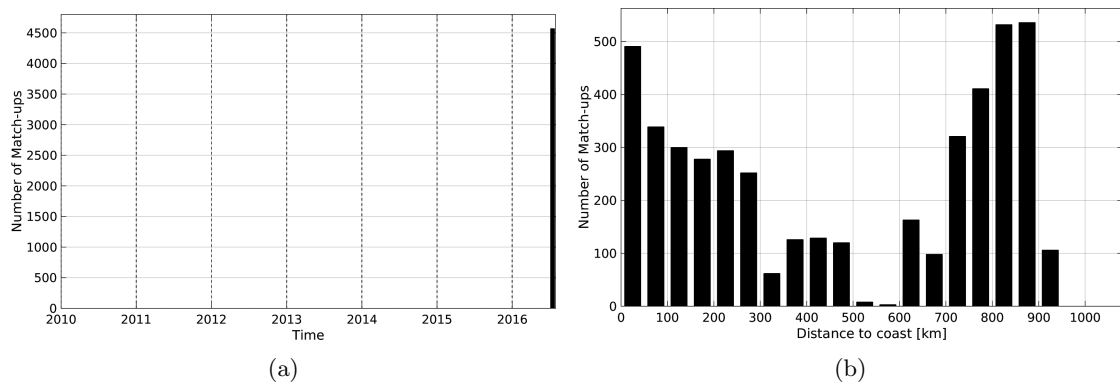
Figure 1: Number of match-ups between TSG-GOSUD-Research-vessel and SMAP-L2-JPL-V4 SSS as a function of time (a) and as function of the distance to coast (b) over the Gulf Stream Pi-MEP region and for the full satellite product period.
