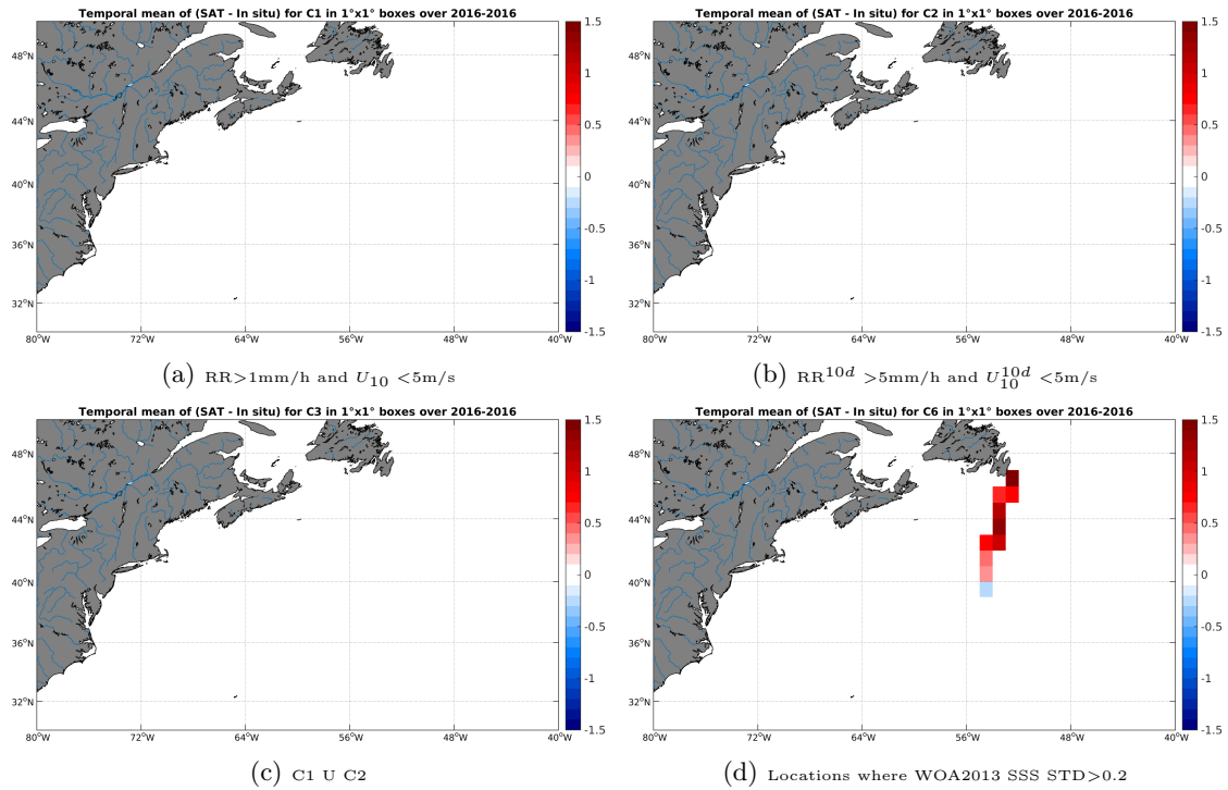
Figure 12: Temporal mean gridded over spatial boxes of size 1^\circ \times 1^\circ of \Delta SSS (SMAP-L2-JPL-V4 - TSG-GOSUD-Research-vessel) for 4 different subdatasets corresponding to: RR > 1mm/h and U_{10} < 5\text{m/s} (a), RR^{10d} > 5\text{mm/h} and U_{10}^{10d} < 5\text{m/s} (b), C1 U C2 (c), Locations where WOA2013 SSS STD > 0.2 (d).
