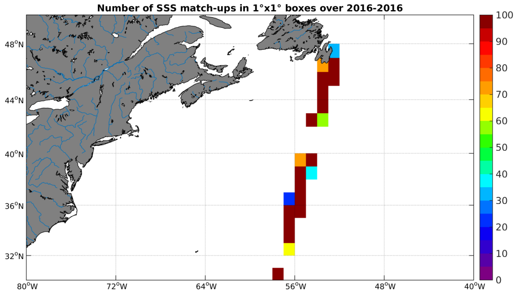
Figure 4: Number of SSS match-ups between TSG-GOSUD-Research-vessel SSS and the SMAP-L2-JPL-V4 SSS product for the Gulf Stream Pi-MEP region over 1°x1° boxes and for the full satellite product period.
