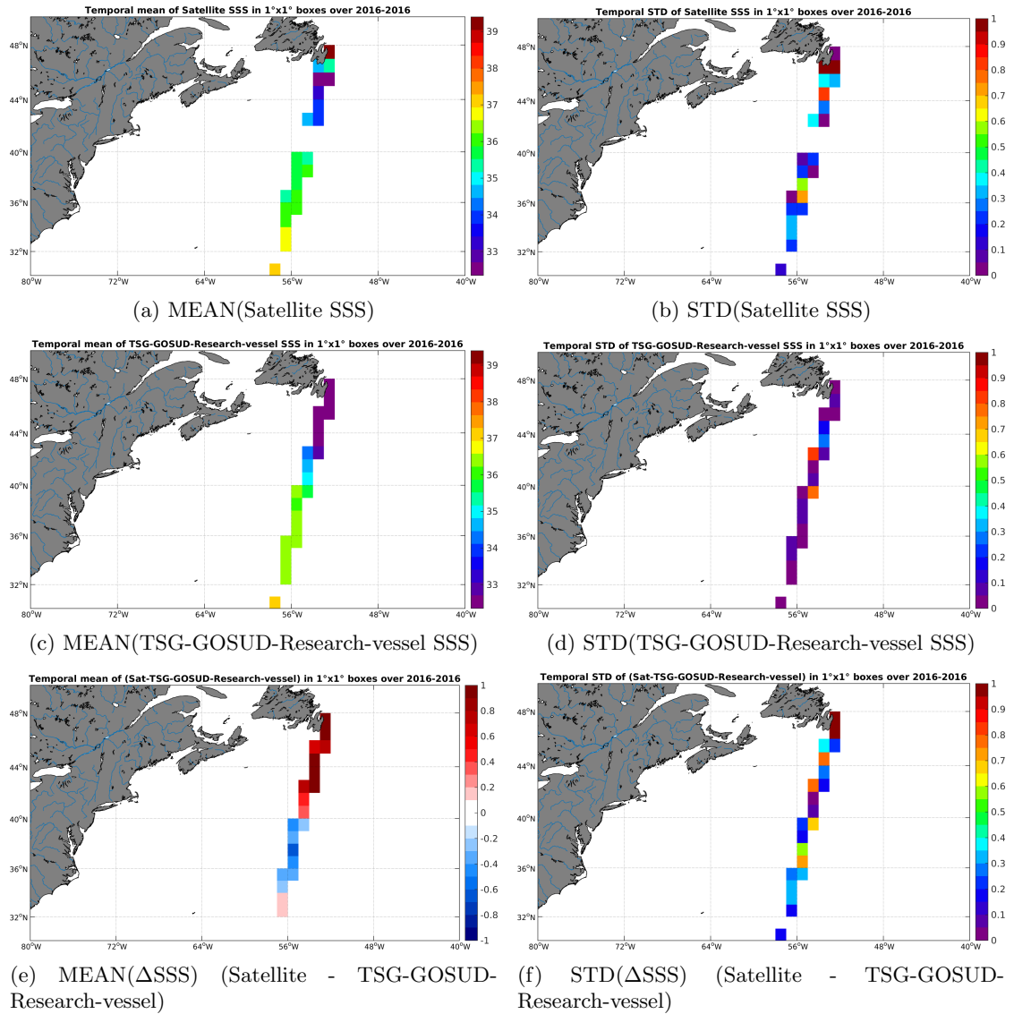
Figure 6: Temporal mean (left) and STD (right) of SSS from SMAP-L2-JPL-V4 (top), TSG-GOSUD-Research-vessel (middle), and of \Delta SSS (Satellite - TSG-GOSUD-Research-vessel). Only match-up pairs are used to generate these maps.
