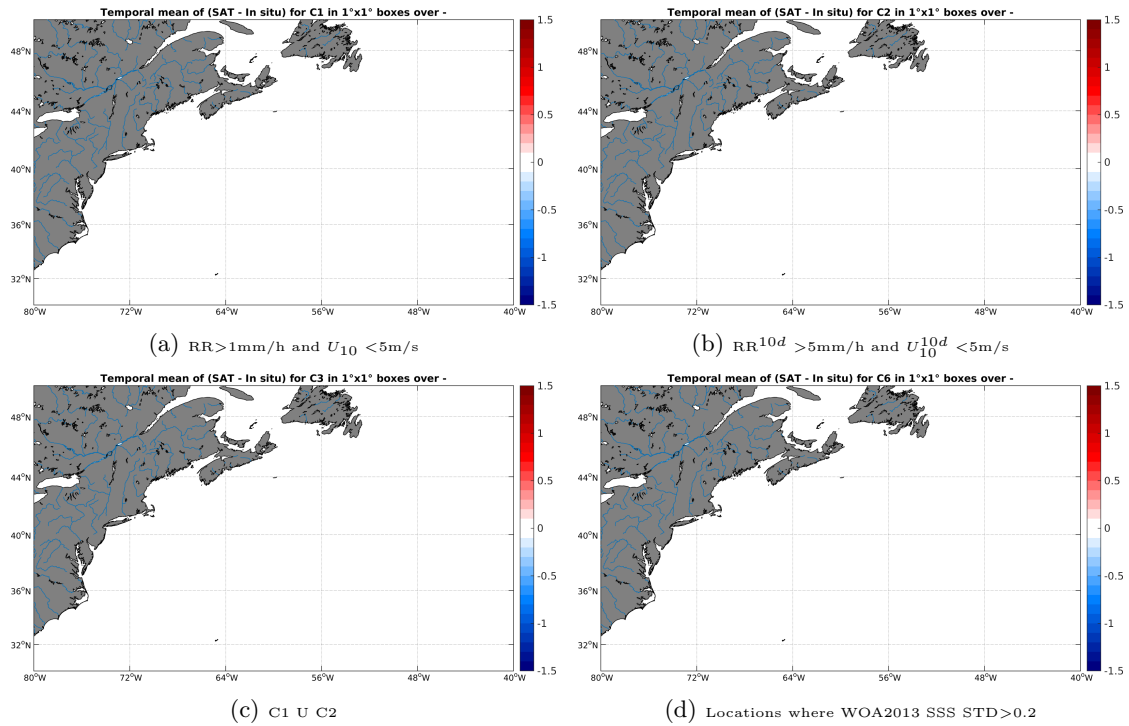
Figure 11: Temporal mean gridded over spatial boxes of size 1^\circ \times 1^\circ of \Delta SSS (SMAP-L2-JPL-V4 - Surface drifters) for 4 different subdatasets corresponding to: RR > 1mm/h and U_{10} < 5 m/s (a), RR^{10d} > 5 mm/h and U_{10}^{10d} < 5 m/s (b), C1 U C2 (c), Locations where WOA2013 SSS STD > 0.2 (d).
