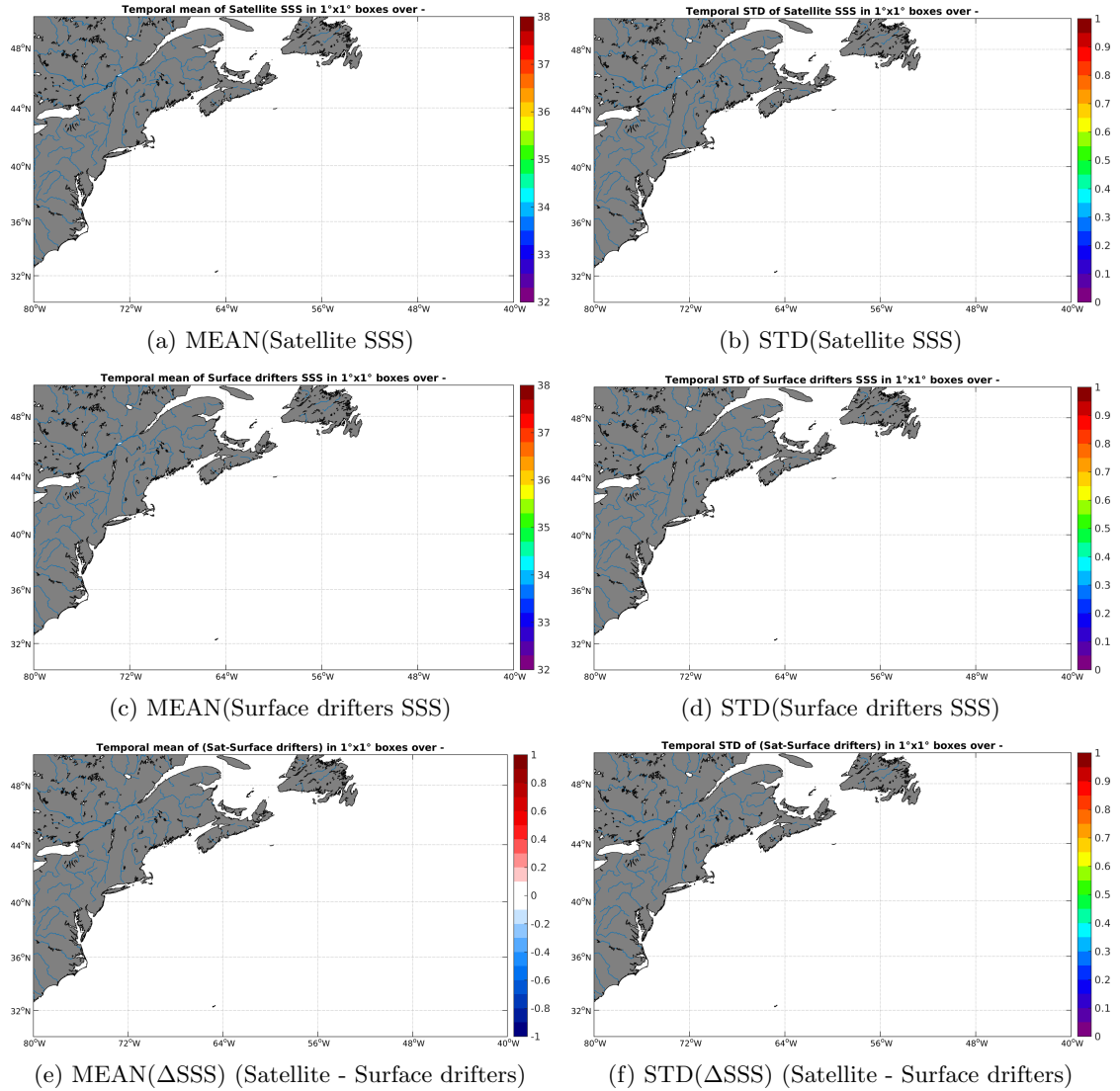
Figure 5: Temporal mean (left) and STD (right) of SSS from SMAP-L2-JPL-V4 (top), Surface drifters (middle), and of \Delta SSS (Satellite - Surface drifters). Only match-up pairs are used to generate these maps.
