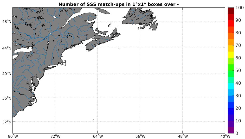
Figure 3: Number of SSS match-ups between Surface drifters SSS and the SMAP-L2-JPL-V4 SSS product for the Gulf Stream Pi-MEP region over 1°x1° boxes and for the full satellite product period.
