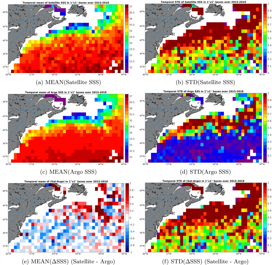
Figure 6: Temporal mean (left) and STD (right) of SSS from SMAP-L2-JPL-V4 (top), Argo (middle), and of \Delta\text{SSS} (Satellite - Argo). Only match-up pairs are used to generate these maps.
