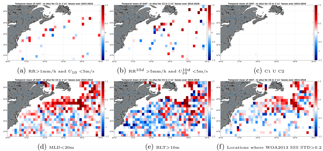
Figure 12: Temporal mean gridded over spatial boxes of size 1^\circ \times 1^\circ of \Delta\text{SSS} (SMAP-L2-JPL-V4 - Argo) for 6 different subdatasets corresponding to: RR > 1\text{mm/h} and U_{10} < 5\text{m/s} (a), RR^{10d} > 5\text{mm/h} and U_{10}^{10d} < 5\text{m/s} (b), C1 U C2 (c), MLD < 20\text{m} (d), BLT > 10\text{m} (e), Locations where WOA2013 SSS STD > 0.2 (f).
