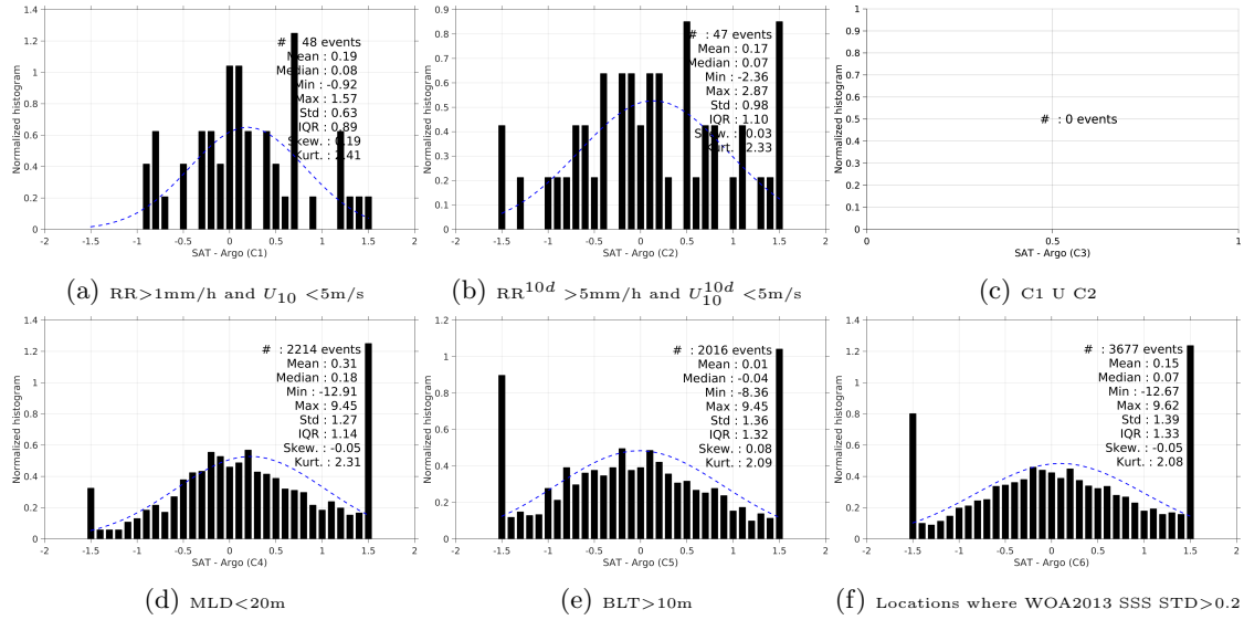
Figure 13: Normalized histogram of \Delta SSS (SMAP-L2-JPL-V4 - Argo) for 6 different subdatasets corresponding to: RR>1mm/h and U_{10} < 5 m/s (a), RR 10d >5mm/h and U_{10}^{10d} < 5 m/s (b), C1 U C2 (c),MLD<20m (d),BLT>10m (e),Locations where WOA2013 SSS STD>0.2 (f).
