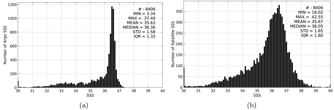
Figure 2: Histograms of SSS from Argo (a) and SMAP-L2-JPL-V4 (b) considering all match-up pairs per bins of 0.1 over the Gulf Stream Pi-MEP region and for the full satellite product period.
