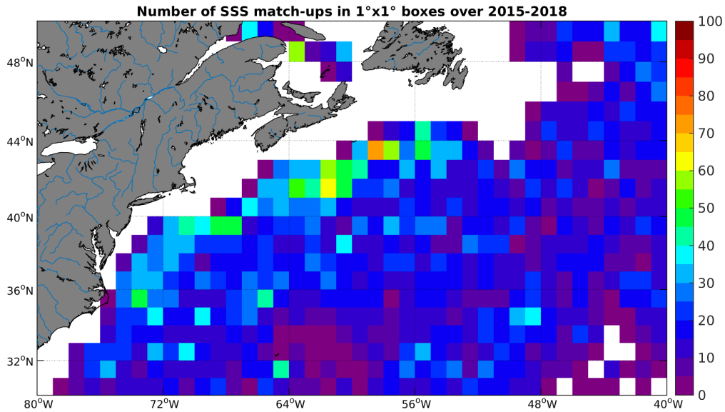
Figure 4: Number of SSS match-ups between Argo SSS and the SMAP-L2-JPL-V4 SSS product for the Gulf Stream Pi-MEP region over 1^\circ \times 1^\circ boxes and for the full satellite product period.
