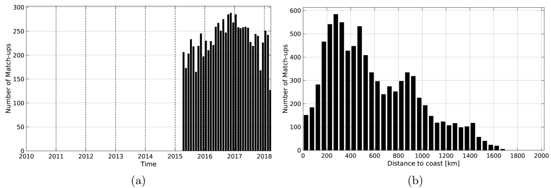
Figure 1: Number of match-ups between Argo and SMAP-L2-JPL-V4 SSS as a function of time (a) and as function of the distance to coast (b) over the Gulf Stream Pi-MEP region and for the full satellite product period.
