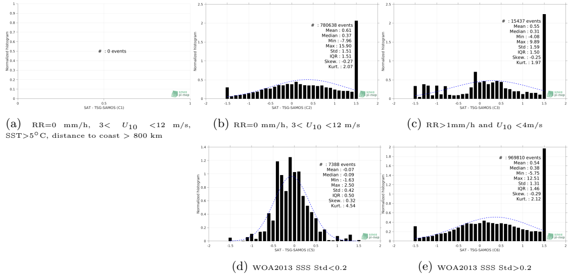
Figure 13: Normalized histogram of \Delta SSS (SMAP-L2-JPL-V4.3 - TSG-SAMOS) for 5 different subdatasets corresponding to: RR=0 mm/h, 3 < U_{10} < 12 m/s, SST > 5°C, distance to coast > 800 km (a), RR=0 mm/h, 3 < U_{10} < 12 m/s (b), RR > 1mm/h and U_{10} < 4 m/s (c), WOA2013 SSS Std < 0.2 (d), WOA2013 SSS Std > 0.2 (e).
