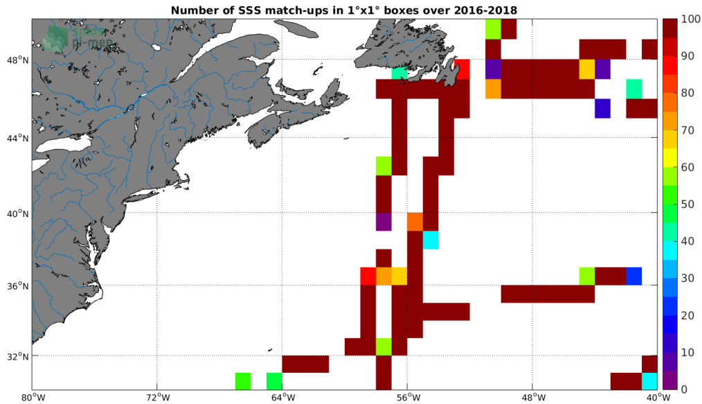
Figure 4: Number of SSS match-ups between TSG-GOSUD-Research-vessel SSS and the SMAP-L2-JPL-V4.3 SSS product for the Gulf Stream Pi-MEP region over 1^\circ \times 1^\circ boxes and for the full satellite product period.
