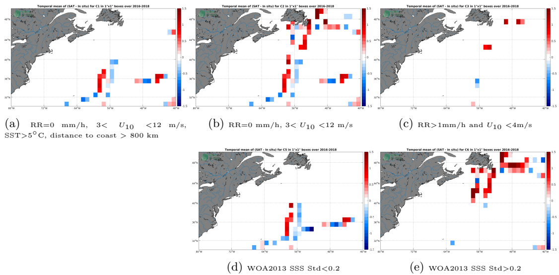
Figure 12: Temporal mean gridded over spatial boxes of size 1°x1° of \Delta SSS (SMAP-L2-JPL-V4.3 - TSG-GOSUD-Research-vessel) for 5 different subdatasets corresponding to:RR=0 mm/h, 3 < U_{10} < 12 m/s, SST>5°C, distance to coast > 800 km (a), RR=0 mm/h, 3 < U_{10} < 12 m/s (b), RR>1mm/h and U_{10} < 4 m/s (c), WOA2013 SSS Std<0.2 (d), WOA2013 SSS Std>0.2 (e).
