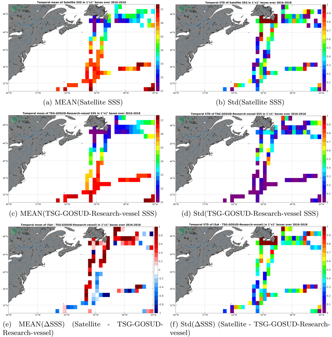
Figure 6: Temporal mean (left) and Std (right) of SSS from SMAP-L2-JPL-V4.3 (top), TSG-GOSUD-Research-vessel (middle), and of \Delta\text{SSS} (Satellite - TSG-GOSUD-Research-vessel). Only match-up pairs are used to generate these maps.
