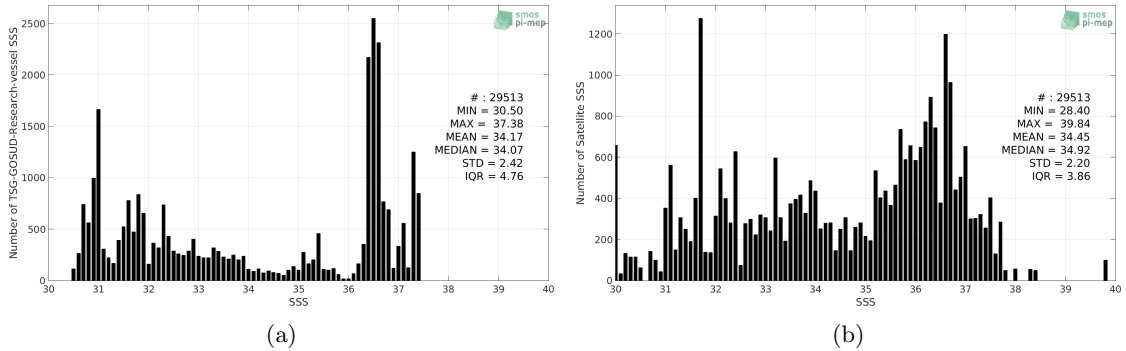
Figure 2: Histograms of SSS from TSG-GOSUD-Research-vessel (a) and SMAP-L2-JPL-V4.3 (b) considering all match-up pairs per bins of 0.1 over the Gulf Stream Pi-MEP region and for the full satellite product period.
