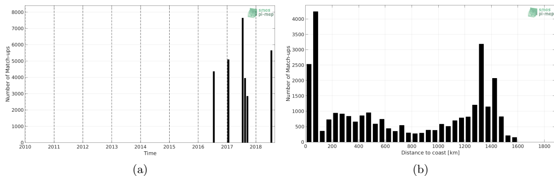
Figure 1: Number of match-ups between TSG-GOSUD-Research-vessel and SMAP-L2-JPL-V4.3 SSS as a function of time (a) and as function of the distance to coast (b) over the Gulf Stream Pi-MEP region and for the full satellite product period.
