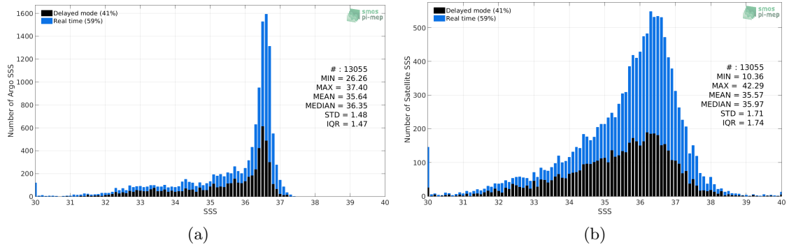
Figure 2: Histograms of SSS from Argo (a) and SMAP-L2-JPL-V4.3 (b) considering all match-up pairs per bins of 0.1 over the Gulf Stream Pi-MEP region and for the full satellite product period.
