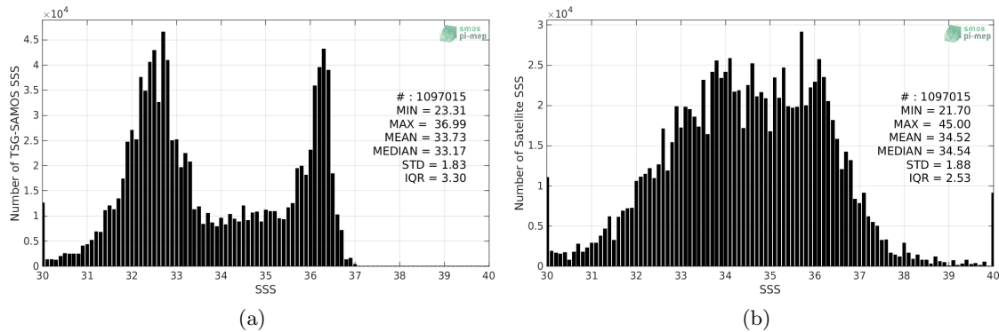
Figure 2: Histograms of SSS from TSG-SAMOS (a) and SMAP-L2-JPL-V4.2 (b) considering all match-up pairs per bins of 0.1 over the Gulf Stream Pi-MEP region and for the full satellite product period.
