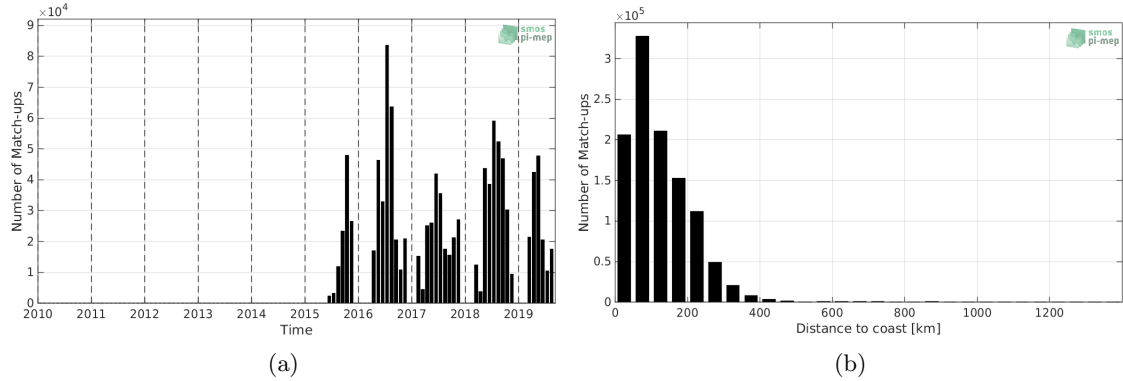
Figure 1: Number of match-ups between TSG-SAMOS and SMAP-L2-JPL-V4.2 SSS as a function of time (a) and as function of the distance to coast (b) over the Gulf Stream Pi-MEP region and for the full satellite product period.
