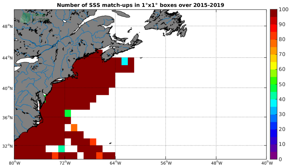
Figure 4: Number of SSS match-ups between TSG-SAMOS SSS and the SMAP-L2-JPL-V4.2 SSS product for the Gulf Stream Pi-MEP region over 1^\circ \times 1^\circ boxes and for the full satellite product period.
