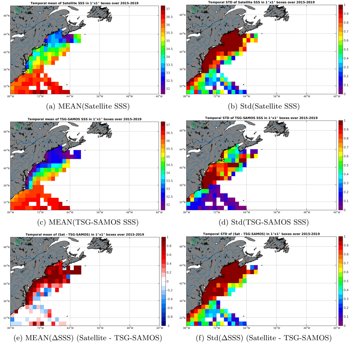
Figure 6: Temporal mean (left) and Std (right) of SSS from SMAP-L2-JPL-V4.2 (top), TSG-SAMOS (middle), and of \Delta SSS (Satellite - TSG-SAMOS). Only match-up pairs are used to generate these maps.
