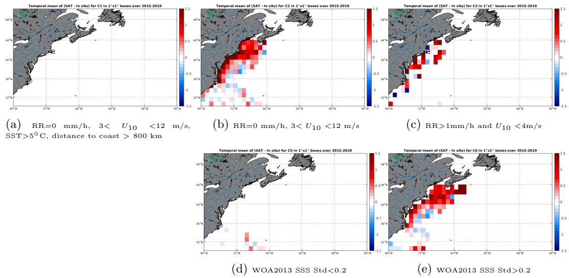
Figure 12: Temporal mean gridded over spatial boxes of size 1^\circ \times 1^\circ of \Delta SSS (SMAP-L2-JPL-V4.2 - TSG-SAMOS) for 5 different subdatasets corresponding to:RR=0 mm/h, 3 < U_{10} < 12 m/s, SST >5^\circ C, distance to coast > 800 km (a), RR=0 mm/h, 3 < U_{10} < 12 m/s (b), RR >1 mm/h and U_{10} < 4 m/s (c), WOA2013 SSS Std <0.2 (d), WOA2013 SSS Std >0.2 (e).
