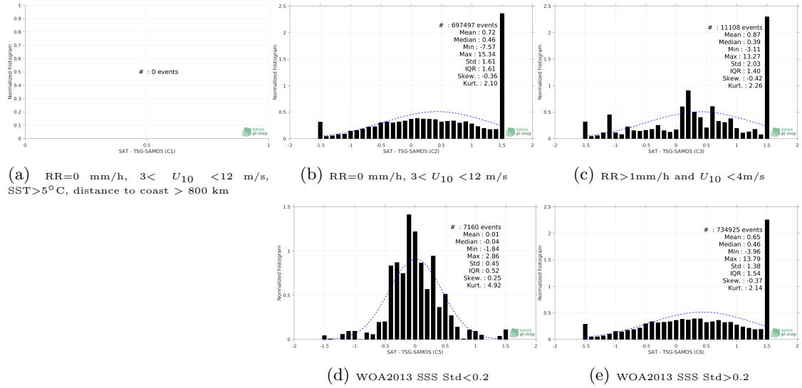
Figure 13: Normalized histogram of \Delta SSS (SMAP-L2-JPL-V4.2 - TSG-SAMOS) for 5 different subdatasets corresponding to: RR=0 mm/h, 3 < U_{10} < 12 m/s, SST > 5°C, distance to coast > 800 km (a), RR=0 mm/h, 3 < U_{10} < 12 m/s (b), RR > 1mm/h and U_{10} < 4 m/s (c), WOA2013 SSS Std < 0.2 (d), WOA2013 SSS Std > 0.2 (e).
