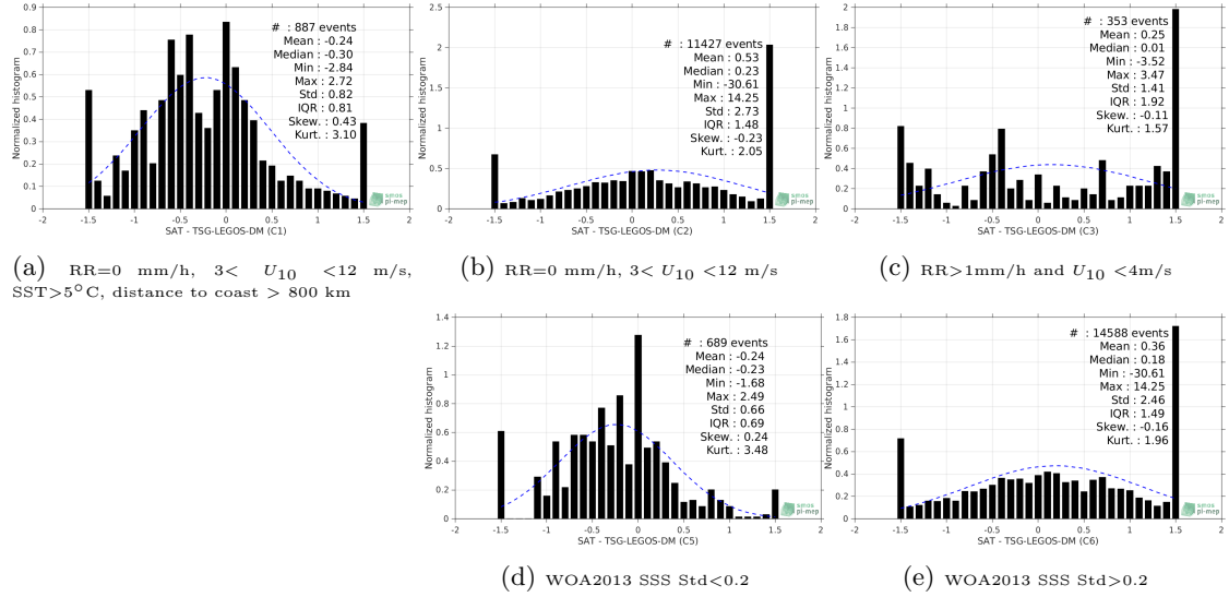
Figure 13: Normalized histogram of \Delta\text{SSS} (SMAP-L2-JPL-V4.2 - TSG-LEGOS-DM) for 5 different subdatasets corresponding to: RR=0 mm/h, 3 < U_{10} < 12 m/s, SST>5°C, distance to coast > 800 km (a), RR=0 mm/h, 3 < U_{10} < 12 m/s (b), RR>1mm/h and U_{10} < 4 m/s (c), WOA2013 SSS Std<0.2 (d), WOA2013 SSS Std>0.2 (e).
