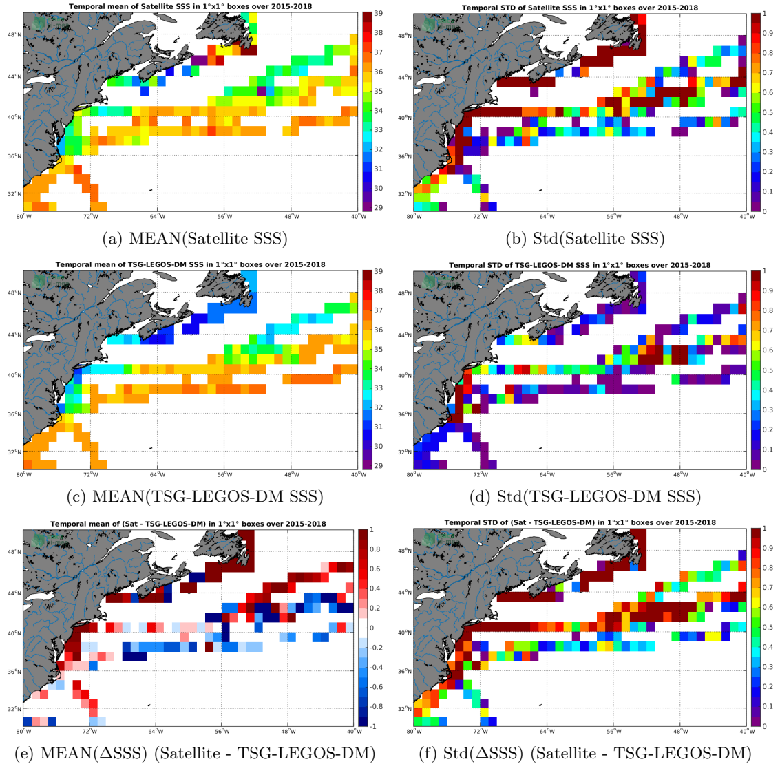
Figure 6: Temporal mean (left) and Std (right) of SSS from SMAP-L2-JPL-V4.2 (top), TSG-LEGOS-DM (middle), and of \Delta SSS (Satellite - TSG-LEGOS-DM). Only match-up pairs are used to generate these maps.
