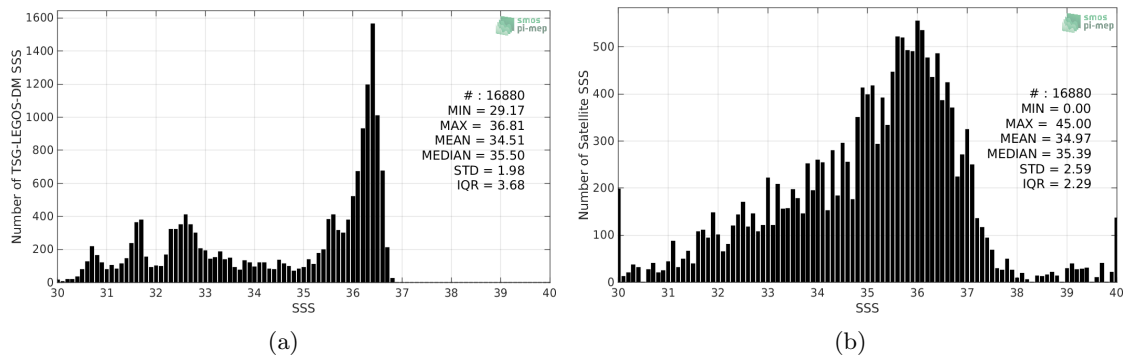
Figure 2: Histograms of SSS from TSG-LEGOS-DM (a) and SMAP-L2-JPL-V4.2 (b) considering all match-up pairs per bins of 0.1 over the Gulf Stream Pi-MEP region and for the full satellite product period.
