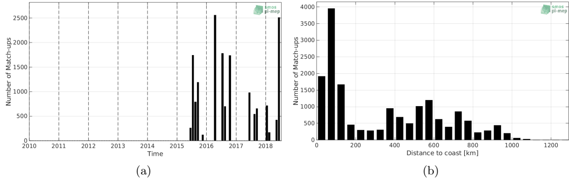
Figure 1: Number of match-ups between TSG-LEGOS-DM and SMAP-L2-JPL-V4.2 SSS as a function of time (a) and as function of the distance to coast (b) over the Gulf Stream Pi-MEP region and for the full satellite product period.
