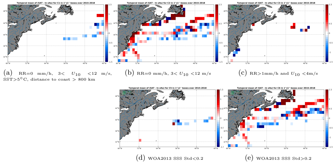
Figure 12: Temporal mean gridded over spatial boxes of size 1^\circ \times 1^\circ of \Delta SSS (SMAP-L2-JPL-V4.2 - TSG-LEGOS-DM) for 5 different subdatasets corresponding to:RR=0 mm/h, 3 < U_{10} < 12 m/s, SST >5^\circ C, distance to coast > 800 km (a), RR=0 mm/h, 3 < U_{10} < 12 m/s (b), RR >1 mm/h and U_{10} < 4 m/s (c), WOA2013 SSS Std <0.2 (d), WOA2013 SSS Std >0.2 (e).
