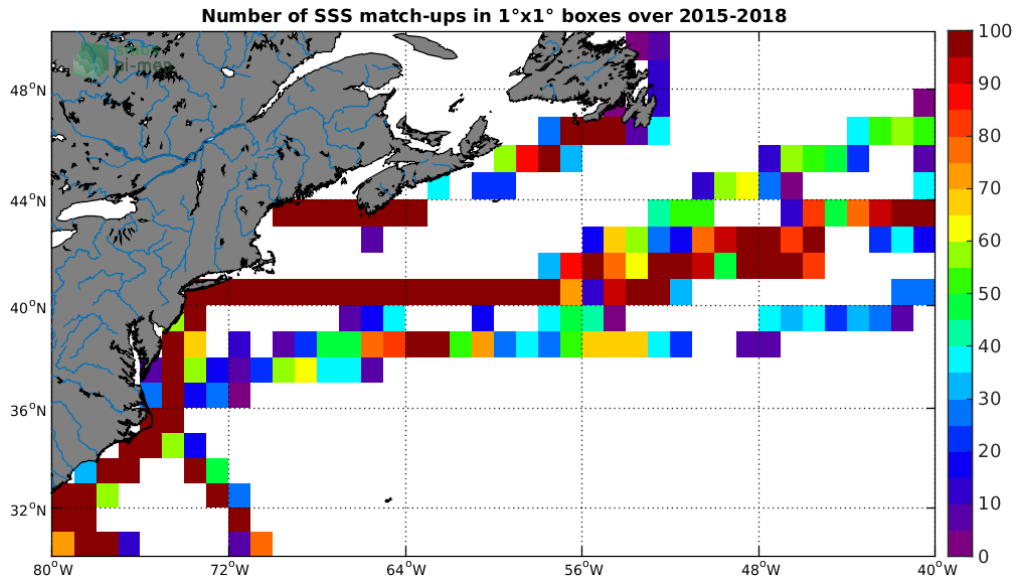
Figure 4: Number of SSS match-ups between TSG-LEGOS-DM SSS and the SMAP-L2-JPL-V4.2 SSS product for the Gulf Stream Pi-MEP region over 1^\circ \times 1^\circ boxes and for the full satellite product period.
