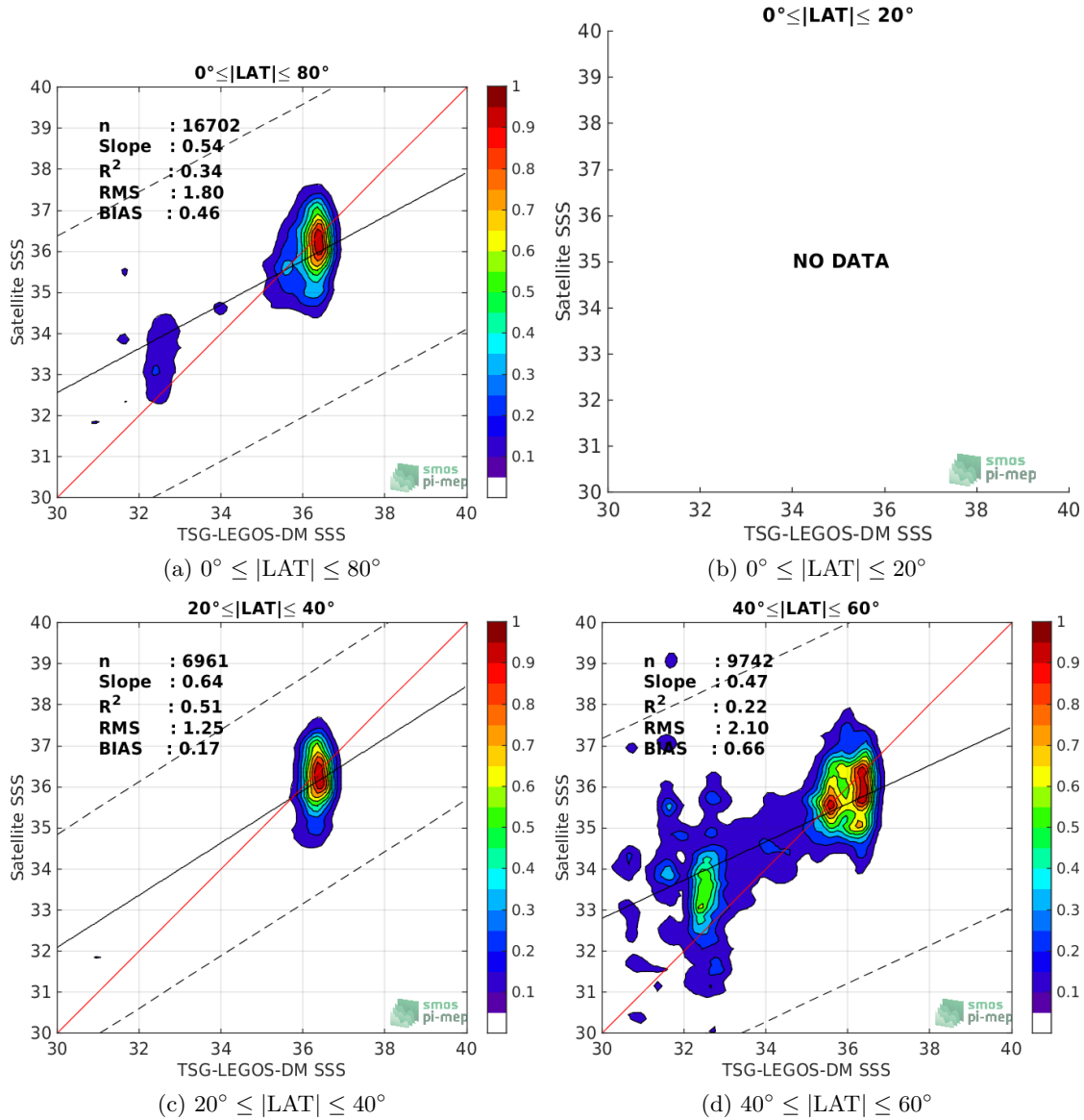
Figure 9: Contour maps of the concentration of SMAP-L2-JPL-V4.2 SSS (y-axis) versus TSG-LEGOS-DM SSS (x-axis) at match-up pairs for different latitude bands. For each plot, the red line shows x=y . The black thin and dashed lines indicate a linear fit through the data cloud and the \pm 95\% confidence levels, respectively. The number match-up pairs n , the slope and R^2 coefficient of the linear fit, the root mean square (RMS) and the mean bias between satellite and in situ data are indicated for each latitude band in each plots.
