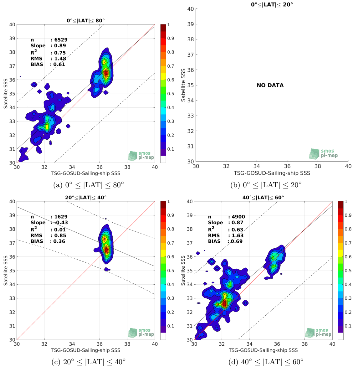
Figure 9: Contour maps of the concentration of SMAP-L2-JPL-V4.2 SSS (y-axis) versus TSG-GOSUD-Sailing-ship SSS (x-axis) at match-up pairs for different latitude bands. For each plot, the red line shows x=y . The black thin and dashed lines indicate a linear fit through the data cloud and the \pm 95\% confidence levels, respectively. The number match-up pairs n , the slope and R^2 coefficient of the linear fit, the root mean square (RMS) and the mean bias between satellite and in situ data are indicated for each latitude band in each plots.
