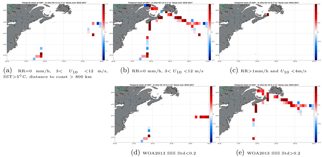
Figure 12: Temporal mean gridded over spatial boxes of size 1^\circ \times 1^\circ of \Delta SSS (SMAP-L2-JPL-V4.2 - TSG-GOSUD-Sailing-ship) for 5 different subdatasets corresponding to: RR=0 mm/h, 3 < U_{10} < 12 m/s, SST > 5^\circ C , distance to coast > 800 km (a), RR=0 mm/h, 3 < U_{10} < 12 m/s (b), RR > 1 mm/h and U_{10} < 4 m/s (c), WOA2013 SSS Std < 0.2 (d), WOA2013 SSS Std > 0.2 (e).
