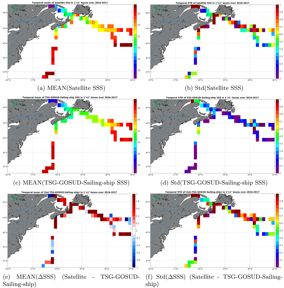
Figure 6: Temporal mean (left) and Std (right) of SSS from SMAP-L2-JPL-V4.2 (top), TSG-GOSUD-Sailing-ship (middle), and of \Delta SSS (Satellite - TSG-GOSUD-Sailing-ship). Only match-up pairs are used to generate these maps.
