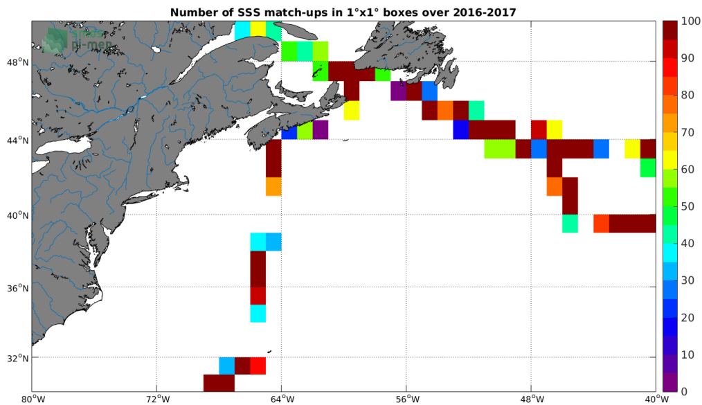
Figure 4: Number of SSS match-ups between TSG-GOSUD-Sailing-ship SSS and the SMAP-L2-JPL-V4.2 SSS product for the Gulf Stream Pi-MEP region over 1^\circ \times 1^\circ boxes and for the full satellite product period.
