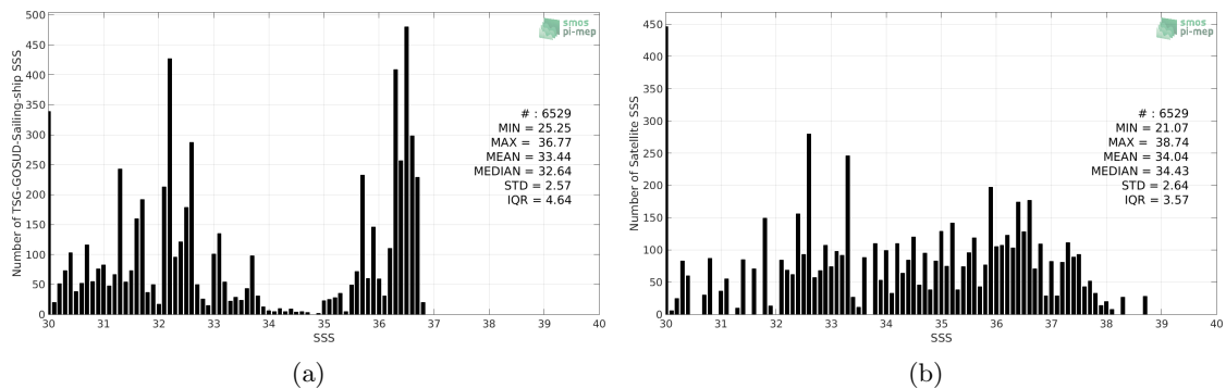
Figure 2: Histograms of SSS from TSG-GOSUD-Sailing-ship (a) and SMAP-L2-JPL-V4.2 (b) considering all match-up pairs per bins of 0.1 over the Gulf Stream Pi-MEP region and for the full satellite product period.
