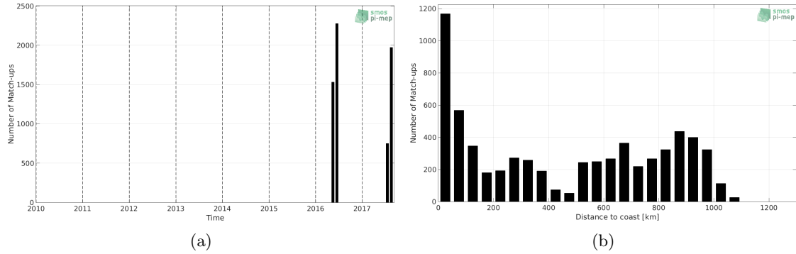
Figure 1: Number of match-ups between TSG-GOSUD-Sailing-ship and SMAP-L2-JPL-V4.2 SSS as a function of time (a) and as function of the distance to coast (b) over the Gulf Stream Pi-MEP region and for the full satellite product period.
