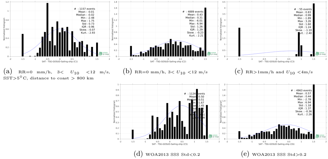
Figure 13: Normalized histogram of \Delta SSS (SMAP-L2-JPL-V4.2 - TSG-GOSUD-Sailing-ship) for 5 different subdatasets corresponding to: RR=0 mm/h, 3 < U_{10} < 12 m/s, SST > 5°C, distance to coast > 800 km (a), RR=0 mm/h, 3 < U_{10} < 12 m/s (b), RR > 1mm/h and U_{10} < 4 m/s (c), WOA2013 SSS Std < 0.2 (d), WOA2013 SSS Std > 0.2 (e).
