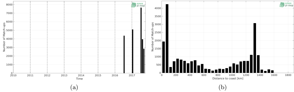
Figure 1: Number of match-ups between TSG-GOSUD-Research-vessel and SMAP-L2-JPL-V4.2 SSS as a function of time (a) and as function of the distance to coast (b) over the Gulf Stream Pi-MEP region and for the full satellite product period.
