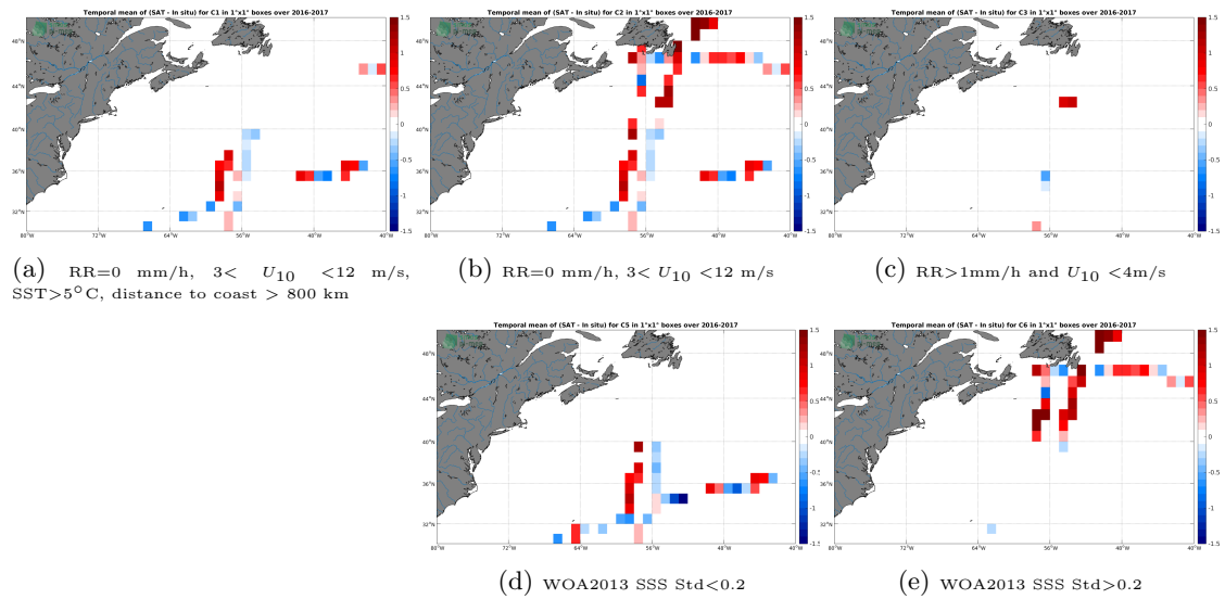
Figure 12: Temporal mean gridded over spatial boxes of size 1^\circ \times 1^\circ of \Delta SSS (SMAP-L2-JPL-V4.2 - TSG-GOSUD-Research-vessel) for 5 different subdatasets corresponding to:RR=0 mm/h, 3 < U_{10} < 12 m/s, SST >5^\circ C, distance to coast > 800 km (a), RR=0 mm/h, 3 < U_{10} < 12 m/s (b), RR >1 mm/h and U_{10} < 4 m/s (c), WOA2013 SSS Std <0.2 (d), WOA2013 SSS Std >0.2 (e).
