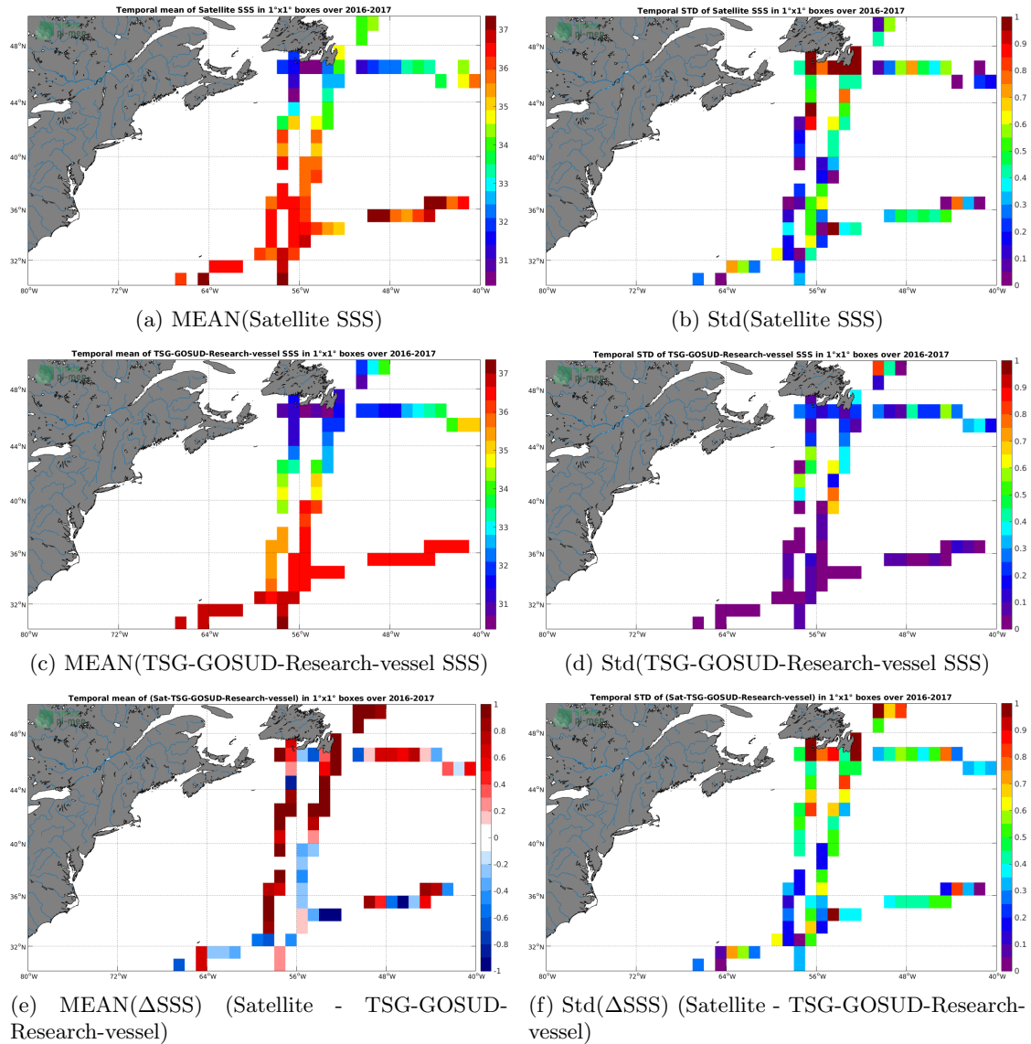
Figure 6: Temporal mean (left) and Std (right) of SSS from SMAP-L2-JPL-V4.2 (top), TSG-GOSUD-Research-vessel (middle), and of \Delta SSS (Satellite - TSG-GOSUD-Research-vessel). Only match-up pairs are used to generate these maps.
