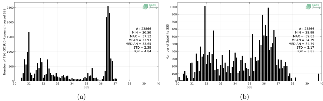
Figure 2: Histograms of SSS from TSG-GOSUD-Research-vessel (a) and SMAP-L2-JPL-V4.2 (b) considering all match-up pairs per bins of 0.1 over the Gulf Stream Pi-MEP region and for the full satellite product period.
