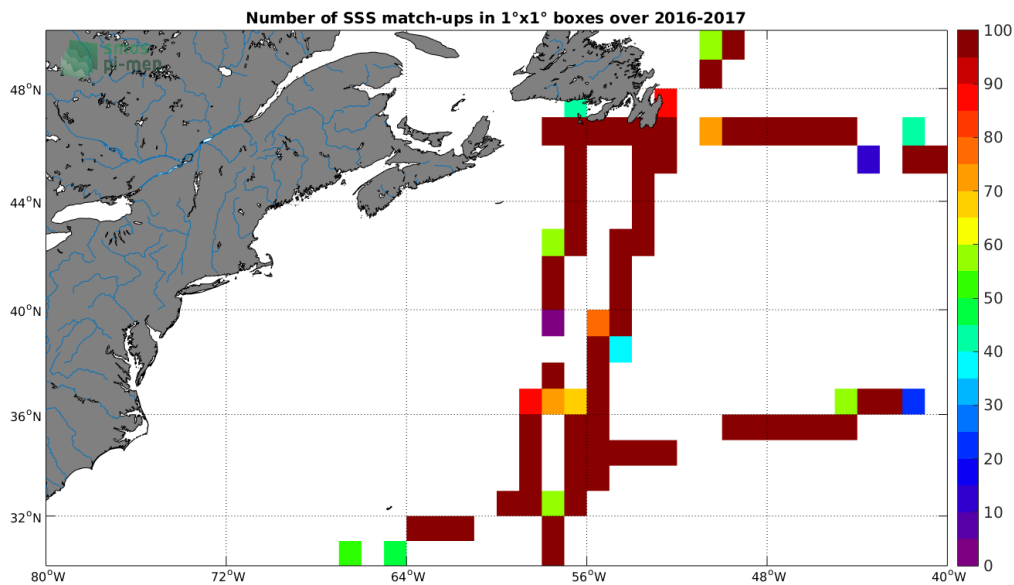
Figure 4: Number of SSS match-ups between TSG-GOSUD-Research-vessel SSS and the SMAP-L2-JPL-V4.2 SSS product for the Gulf Stream Pi-MEP region over 1^\circ \times 1^\circ boxes and for the full satellite product period.
