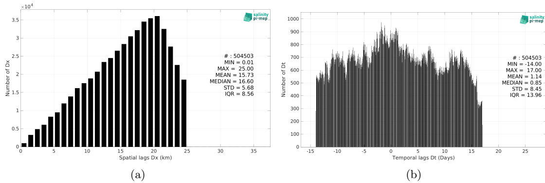
Figure 6: Histograms of the spatial (a) and temporal (b) lags between the location/time of the TSG (SAMOS) measurement and the date of the corresponding ISAS v7 - Monthly (Ifremer-LOPS-CMEMS) SSS pixel.
