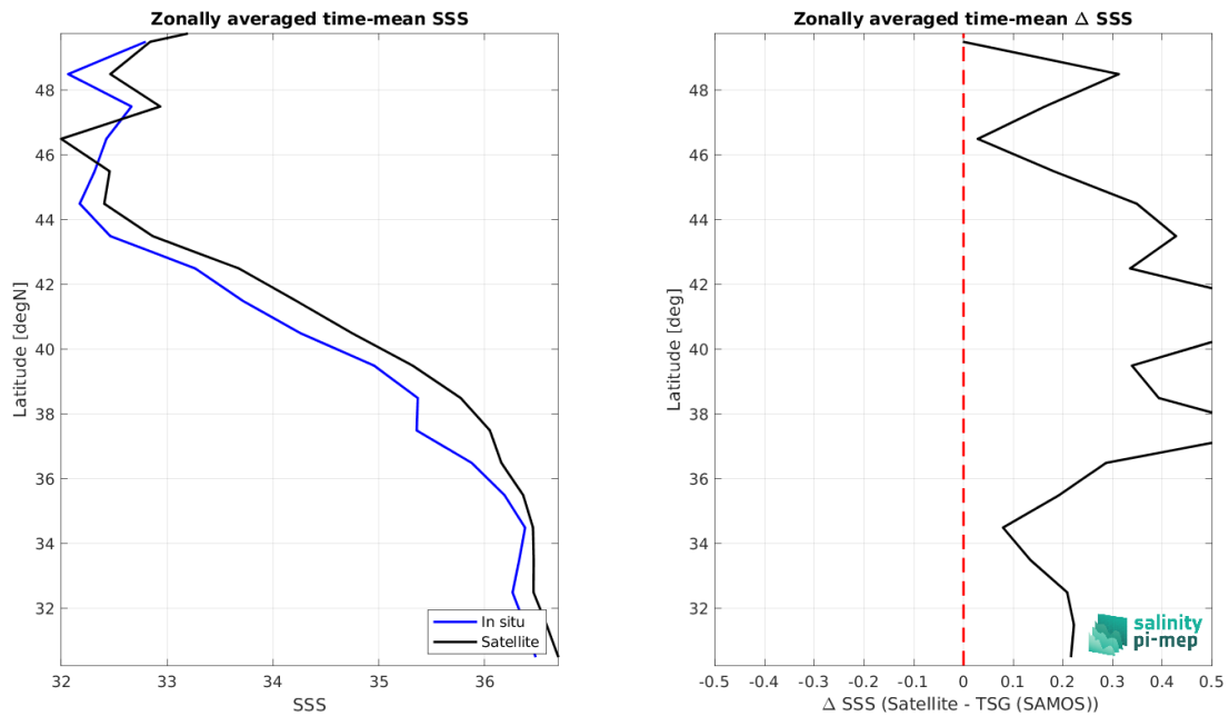
Figure 9: Left panel: Zonal mean SSS from ISAS v7 - Monthly (Ifremer-LOPS-CMEMS) satellite product (black) and from TSG (SAMOS) (blue). Right panel: Zonal mean of \Delta SSS (Satellite - TSG (SAMOS)) for all the collected Pi-MEP match-up pairs estimated over the full satellite product period.
