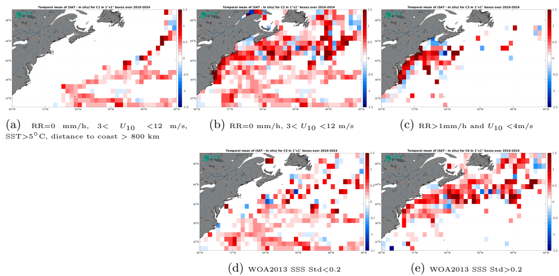
Figure 14: Temporal mean gridded over spatial boxes of size 1^\circ \times 1^\circ of \Delta SSS (ISAS v7 - Monthly (Ifremer-LOPS-CMEMS) - TSG (SAMOS)) for 5 different subdatasets corresponding to:RR=0 mm/h, 3 < U_{10} < 12 m/s, SST > 5^\circ\text{C} , distance to coast > 800 km (a), RR=0 mm/h, 3 < U_{10} < 12 m/s (b), RR > 1 mm/h and U_{10} < 4 m/s (c), WOA2013 SSS Std < 0.2 (d), WOA2013 SSS Std > 0.2 (e).
