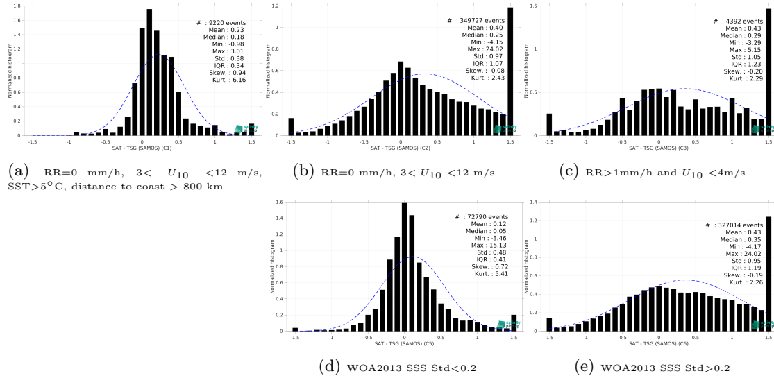
Figure 15: Normalized histogram of \Delta SSS (ISAS v7 - Monthly (Ifremer-LOPS-CMEMS) - TSG (SAMOS)) for 5 different subdatasets corresponding to: RR=0 mm/h, 3 < U_{10} < 12 m/s, SST>5°C, distance to coast > 800 km (a), RR=0 mm/h, 3 < U_{10} < 12 m/s (b), RR>1mm/h and U_{10} < 4 m/s (c), WOA2013 SSS Std<0.2 (d), WOA2013 SSS Std>0.2 (e).
