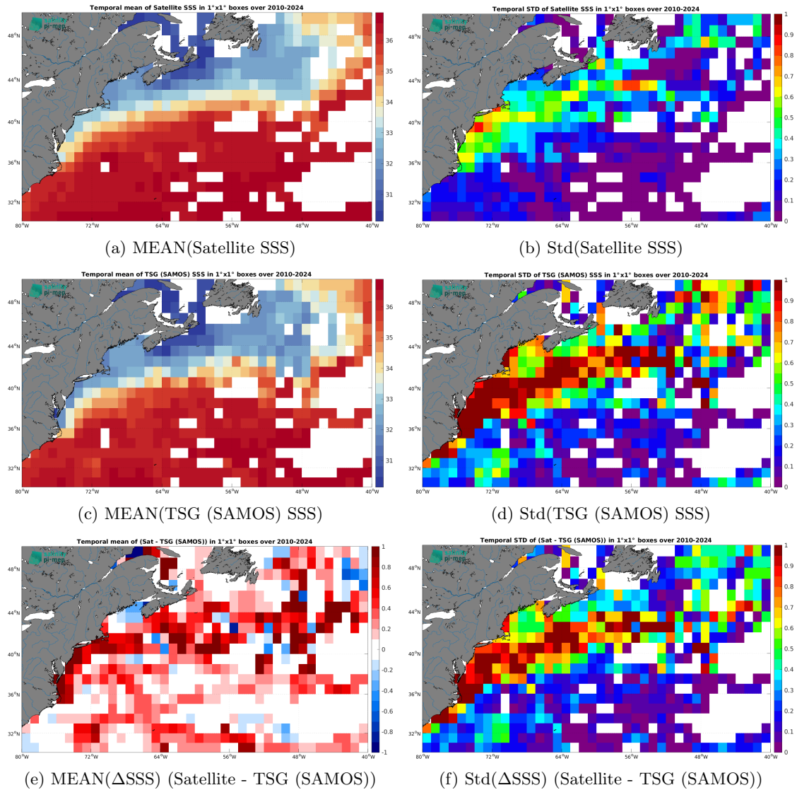
Figure 7: Temporal mean (left) and Std (right) of SSS from ISAS v7 - Monthly (Ifremer-LOPS-CMEMS) (top), TSG (SAMOS) (middle), and of \Delta SSS (Satellite - TSG (SAMOS)). Only match-up pairs are used to generate these maps.
