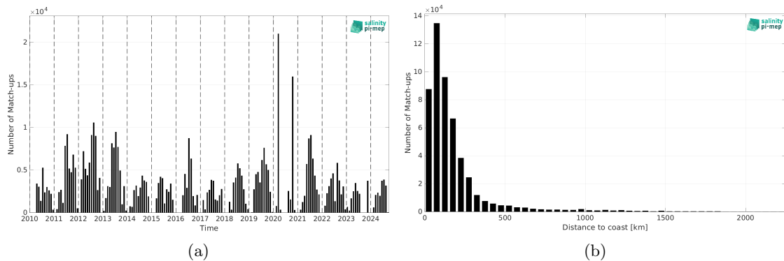
Figure 2: Number of match-ups between TSG (SAMOS) and ISAS v7 - Monthly (Ifremer-LOPS-CMEMS) SSS as a function of time (a) and as function of the distance to coast (b) over the Gulf Stream Pi-MEP region and for the full satellite product period.
