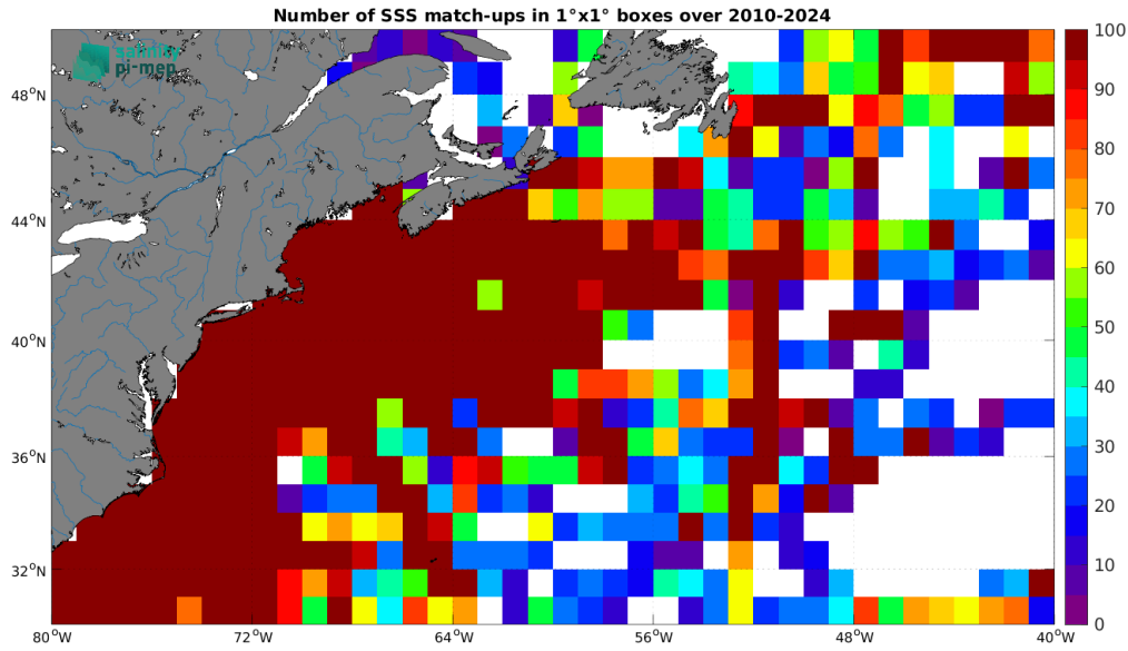
Figure 5: Number of SSS match-ups between TSG (SAMOS) SSS and the ISAS v7 - Monthly (Ifremer-LOPS-CMEMS) SSS product for the Gulf Stream Pi-MEP region over 1^\circ \times 1^\circ boxes and for the full satellite product period.
