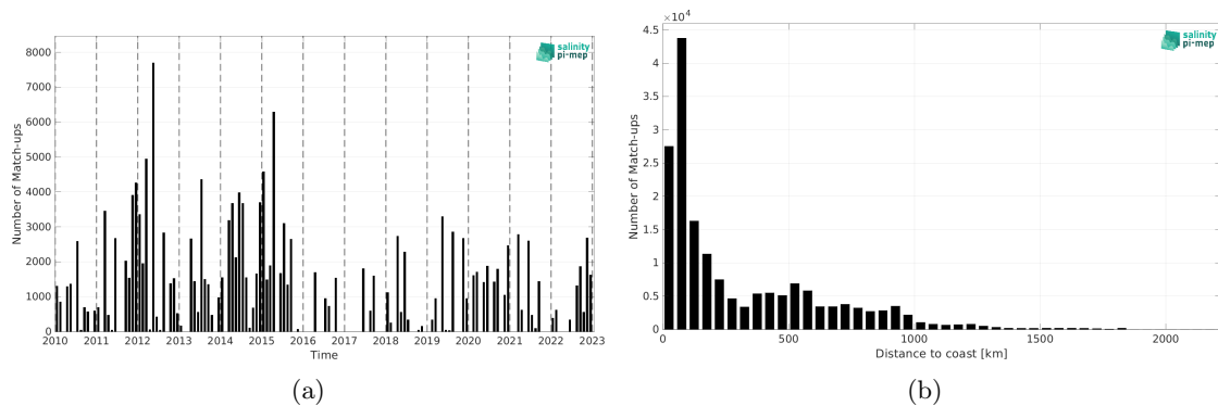
Figure 2: Number of match-ups between TSG (LEGOS-DM) and ISAS v7 - Monthly (Ifremer-LOPS-CMEMS) SSS as a function of time (a) and as function of the distance to coast (b) over the Gulf Stream Pi-MEP region and for the full satellite product period.
