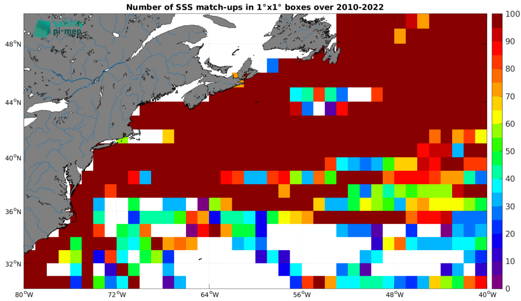
Figure 5: Number of SSS match-ups between TSG (LEGOS-DM) SSS and the ISAS v7 - Monthly (Ifremer-LOPS-CMEMS) SSS product for the Gulf Stream Pi-MEP region over 1^\circ \times 1^\circ boxes and for the full satellite product period.
