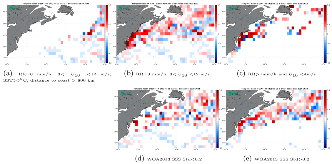
Figure 14: Temporal mean gridded over spatial boxes of size 1^\circ \times 1^\circ of \Delta SSS (ISAS v7 - Monthly (Ifremer-LOPS-CMEMS) - TSG (LEGOS-DM)) for 5 different subdatasets corresponding to: RR=0 mm/h, 3 < U_{10} < 12 m/s, SST > 5°C, distance to coast > 800 km (a), RR=0 mm/h, 3 < U_{10} < 12 m/s (b), RR > 1mm/h and U_{10} < 4 m/s (c), WOA2013 SSS Std < 0.2 (d), WOA2013 SSS Std > 0.2 (e).
