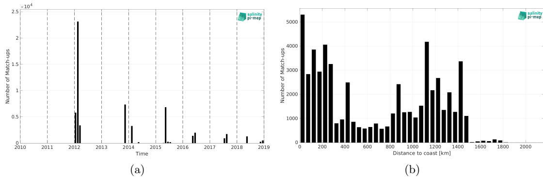
Figure 2: Number of match-ups between TSG (GOSUD-Sailing-ship) and ISAS v7 - Monthly (Ifremer-LOPS-CMEMS) SSS as a function of time (a) and as function of the distance to coast (b) over the Gulf Stream Pi-MEP region and for the full satellite product period.
