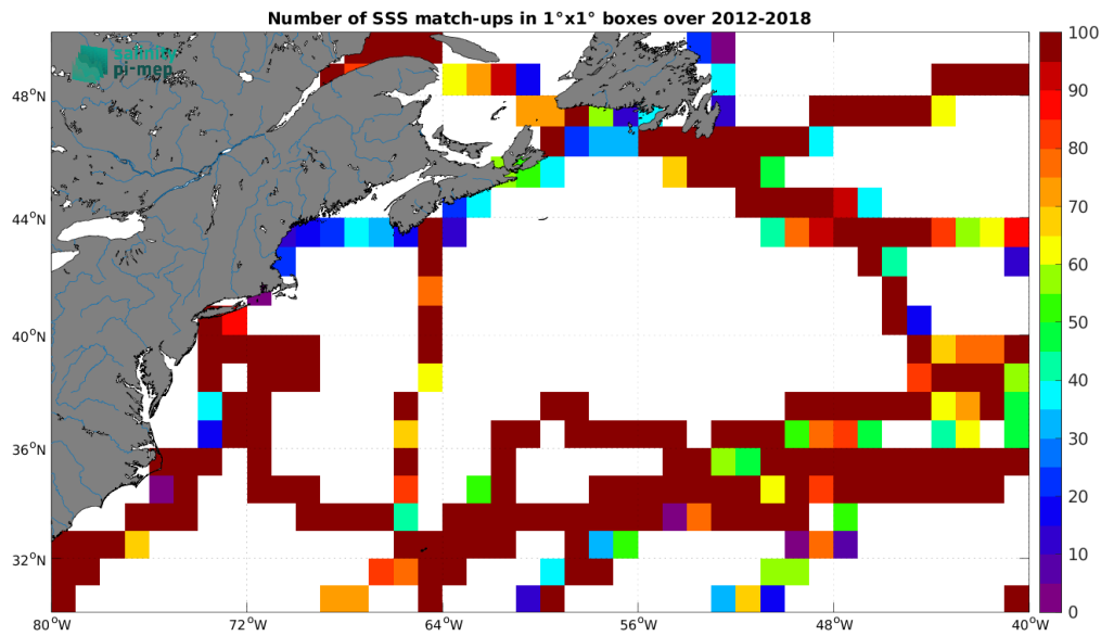
Figure 5: Number of SSS match-ups between TSG (GOSUD-Sailing-ship) SSS and the ISAS v7 - Monthly (Ifremer-LOPS-CMEMS) SSS product for the Gulf Stream Pi-MEP region over 1^\circ \times 1^\circ boxes and for the full satellite product period.
