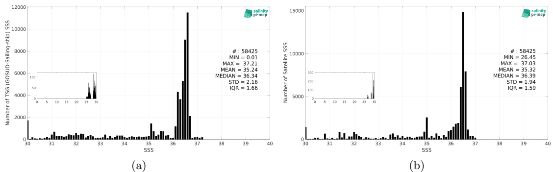
Figure 3: Histograms of SSS from TSG (GOSUD-Sailing-ship) (a) and ISAS v7 - Monthly (Ifremer-LOPS-CMEMS) (b) considering all match-up pairs per bins of 0.1 over the Gulf Stream Pi-MEP region and for the full satellite product period.
