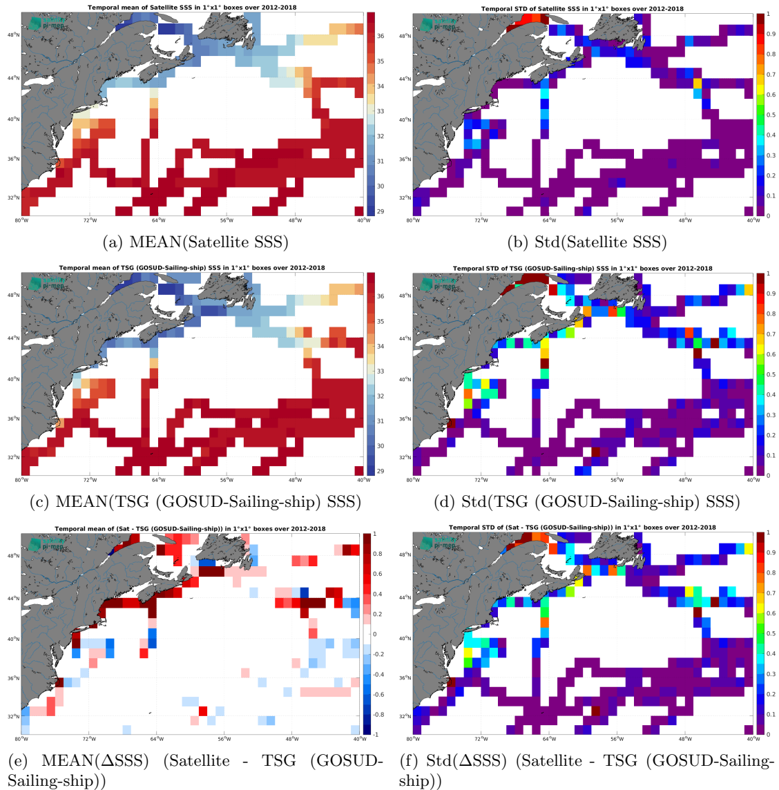
Figure 7: Temporal mean (left) and Std (right) of SSS from ISAS v7 - Monthly (Ifremer-LOPS-CMEMS) (top), TSG (GOSUD-Sailing-ship) (middle), and of \Delta SSS (Satellite - TSG (GOSUD-Sailing-ship)). Only match-up pairs are used to generate these maps.
